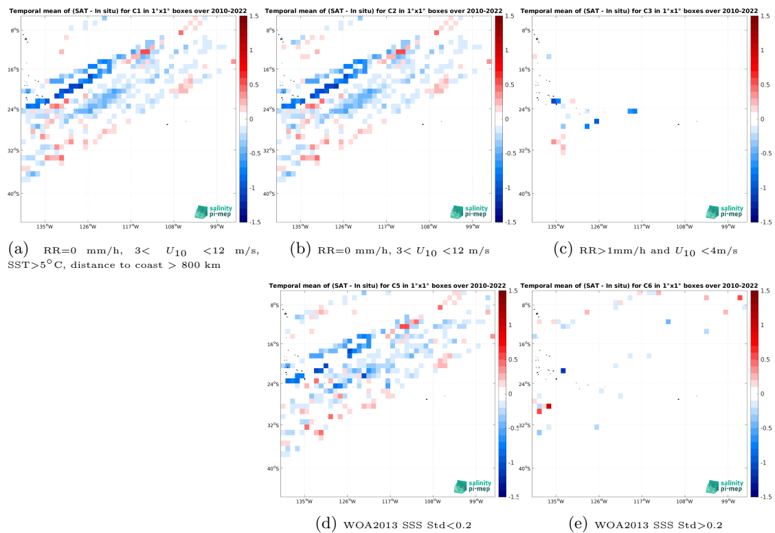
Figure 14: Temporal mean gridded over spatial boxes of size 1^\circ \times 1^\circ of \Delta SSS (SMOS SSS L4 v1 - Daily (CMEMS-CNR) - TSG (LEGOS-DM)) for 5 different subdatasets corresponding to: RR=0 mm/h, 3 < U_{10} < 12 m/s, SST > 5^\circ\text{C} , distance to coast > 800 km (a), RR=0 mm/h, 3 < U_{10} < 12 m/s (b), RR > 1 mm/h and U_{10} < 4 m/s (c), WOA2013 SSS Std < 0.2 (d), WOA2013 SSS Std > 0.2 (e).
