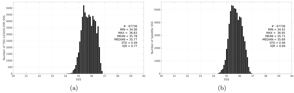
Figure 3: Histograms of SSS from TSG (LEGOS-DM) (a) and SMOS SSS L4 v1 - Daily (CMEMS-CNR) (b) considering all match-up pairs per bins of 0.1 over the OTT zone Pi-MEP region and for the full satellite product period.
