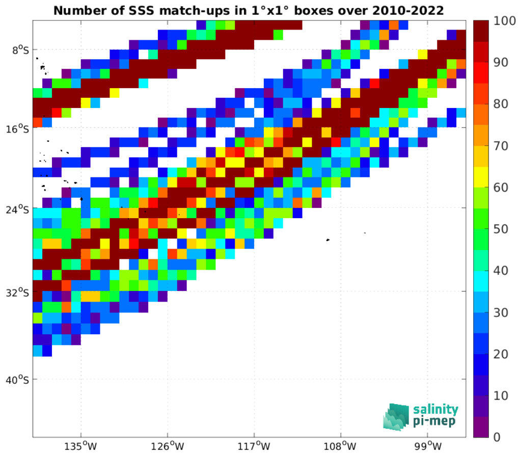
Figure 5: Number of SSS match-ups between TSG (LEGOS-DM) SSS and the SMOS SSS L4 v1 - Daily (CMEMS-CNR) SSS product for the OTT zone Pi-MEP region over 1^\circ \times 1^\circ boxes and for the full satellite product period.
