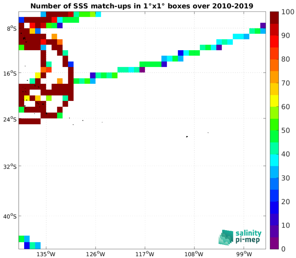
Figure 5: Number of SSS match-ups between TSG (GOSUD-Research-vessel) SSS and the SMOS SSS L4 v1 - Daily (CMEMS-CNR) SSS product for the OTT zone Pi-MEP region over 1^{\circ}\times 1^{\circ} boxes and for the full satellite product period.
