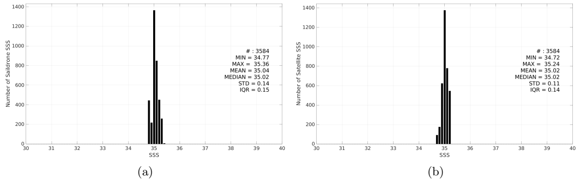
Figure 3: Histograms of SSS from Saildrone (a) and SMOS SSS L4 v1 - Daily (CMEMS-CNR) (b) considering all match-up pairs per bins of 0.1 over the OTT zone Pi-MEP region and for the full satellite product period.
