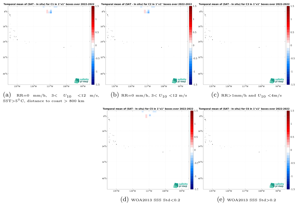
Figure 14: Temporal mean gridded over spatial boxes of size 1^\circ \times 1^\circ of \Delta SSS (SMOS SSS L4 v1 - Daily (CMEMS-CNR) - Sairdrone) for 5 different subdatasets corresponding to: RR=0 mm/h, 3 < U_{10} < 12 m/s, SST > 5^\circ C , distance to coast > 800 km (a), RR=0 mm/h, 3 < U_{10} < 12 m/s (b), RR > 1 mm/h and U_{10} < 4 m/s (c), WOA2013 SSS Std < 0.2 (d), WOA2013 SSS Std > 0.2 (e).
