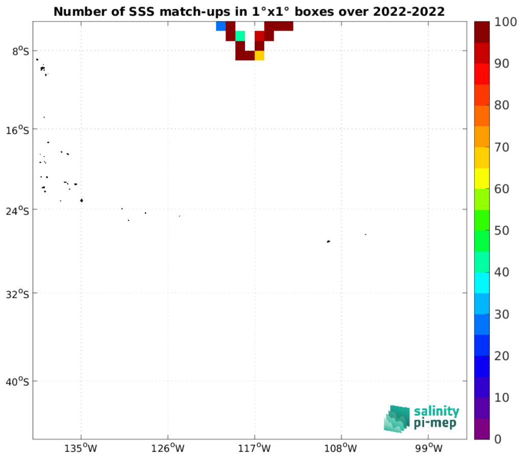
Figure 5: Number of SSS match-ups between Saildrone SSS and the SMOS SSS L4 v1 - Daily (CMEMS-CNR) SSS product for the OTT zone Pi-MEP region over 1°x1° boxes and for the full satellite product period.
