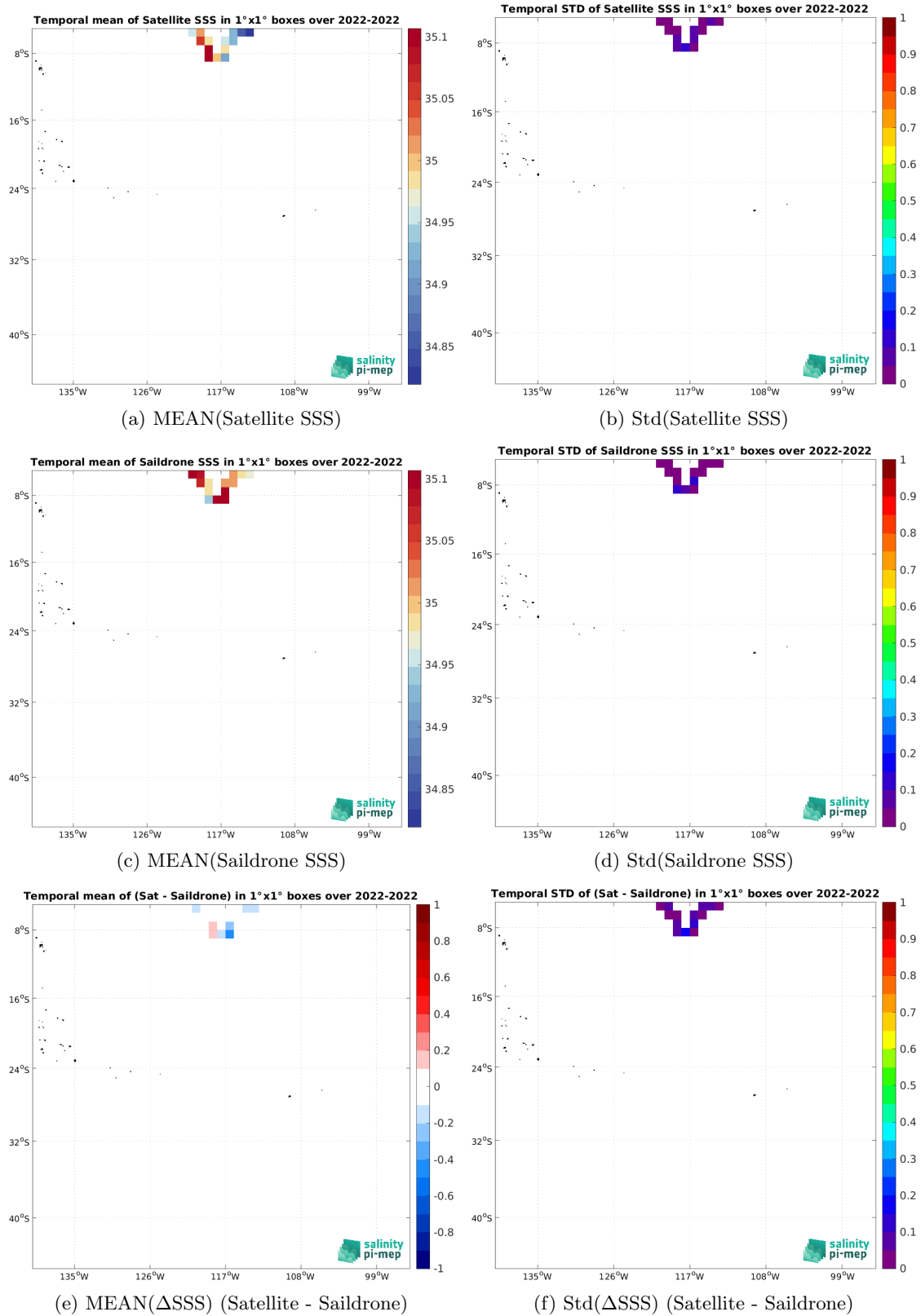
Figure 7: Temporal mean (left) and Std (right) of SSS from SMOS SSS L4 v1 - Daily (CMEMS-CNR) (top), Saildrone (middle), and of \Delta SSS (Satellite - Saildrone). Only match-up pairs are used to generate these maps.
