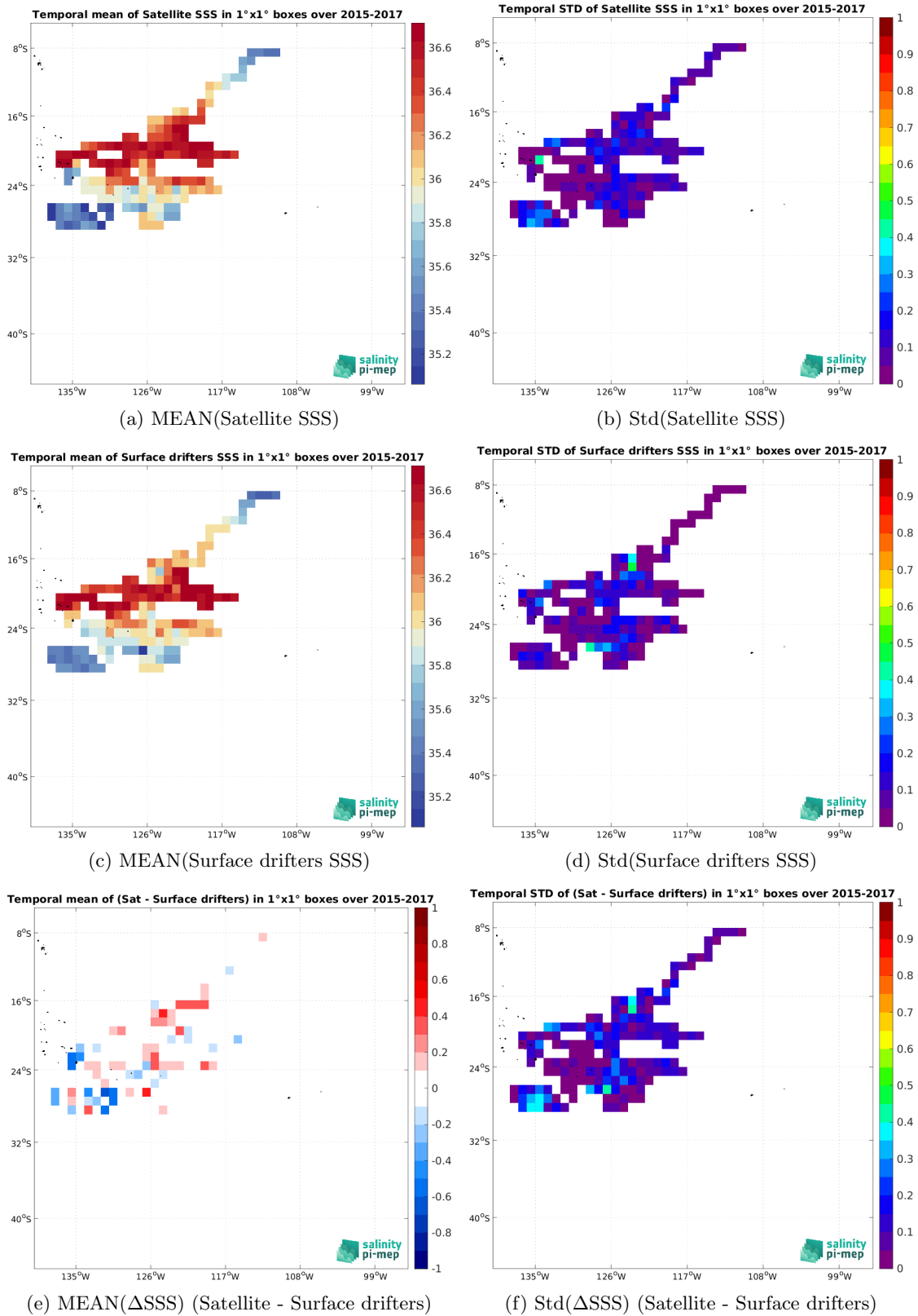
Figure 6: Temporal mean (left) and Std (right) of SSS from SMOS SSS L4 v1 - Daily (CMEMS-CNR) (top), Surface drifters (middle), and of \Delta SSS (Satellite - Surface drifters). Only match-up pairs are used to generate these maps.
