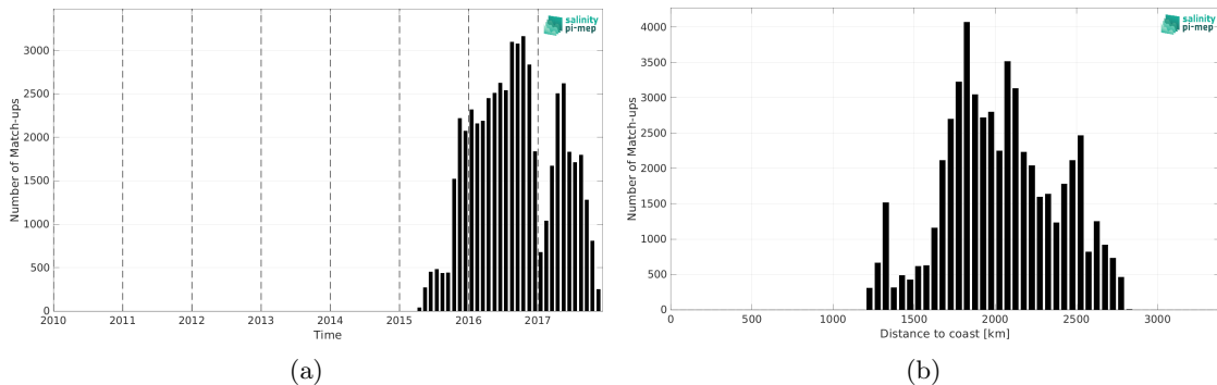
Figure 2: Number of match-ups between Surface drifters and SMOS SSS L4 v1 - Daily (CMEMS-CNR) SSS as a function of time (a) and as function of the distance to coast (b) over the OTT zone Pi-MEP region and for the full satellite product period.
