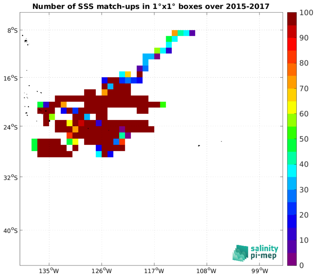
Figure 4: Number of SSS match-ups between Surface drifters SSS and the SMOS SSS L4 v1 - Daily (CMEMS-CNR) SSS product for the OTT zone Pi-MEP region over 1°x1° boxes and for the full satellite product period.
