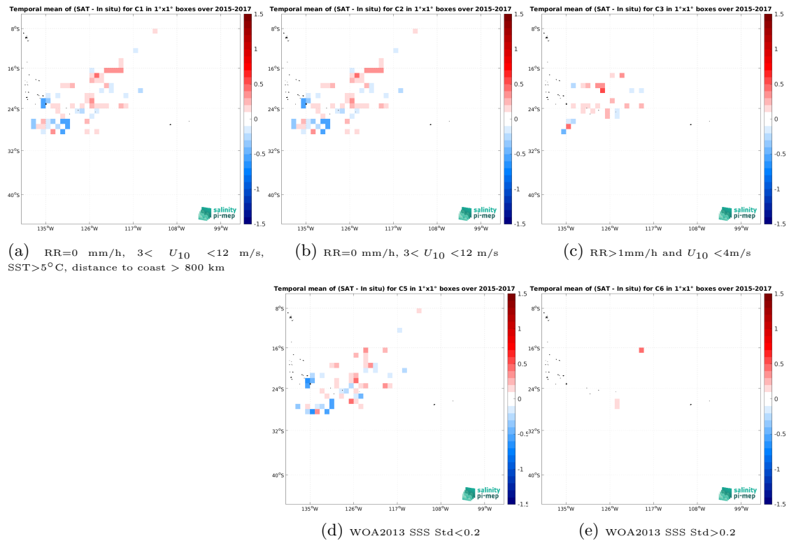
Figure 13: Temporal mean gridded over spatial boxes of size 1^\circ \times 1^\circ of \Delta SSS (SMOS SSS L4 v1 - Daily (CMEMS-CNR) - Surface drifters) for 5 different subdatasets corresponding to:RR=0 mm/h, 3 < U_{10} < 12 m/s, SST >5^\circ C, distance to coast > 800 km (a), RR=0 mm/h, 3 < U_{10} < 12 m/s (b), RR >1 mm/h and U_{10} < 4 m/s (c), WOA2013 SSS Std <0.2 (d), WOA2013 SSS Std >0.2 (e).
