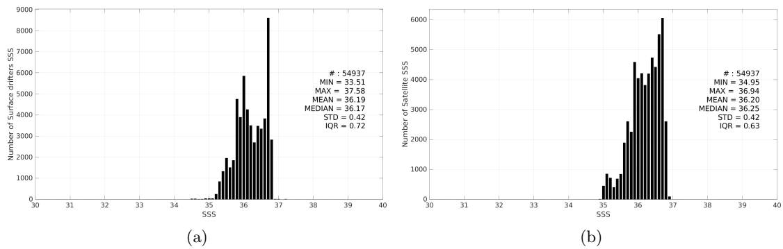
Figure 3: Histograms of SSS from Surface drifters (a) and SMOS SSS L4 v1 - Daily (CMEMS-CNR) (b) considering all match-up pairs per bins of 0.1 over the OTT zone Pi-MEP region and for the full satellite product period.
