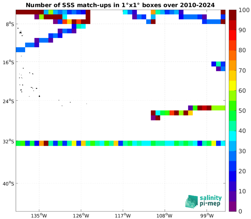
Figure 5: Number of SSS match-ups between TSG (SAMOS) SSS and the SMOS SSS L4 OI v346 - Weekly (CMEMS-CATDS-LOPS) SSS product for the OTT zone Pi-MEP region over 1^\circ \times 1^\circ boxes and for the full satellite product period.
