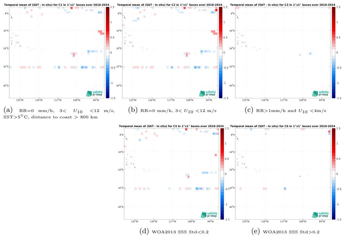
Figure 14: Temporal mean gridded over spatial boxes of size 1^\circ \times 1^\circ of \Delta SSS (SMOS SSS L4 OI v346 - Weekly (CMEMS-CATDS-LOPS) - TSG (SAMOS)) for 5 different subdatasets corresponding to: RR=0 mm/h, 3 < U_{10} < 12 m/s, SST > 5^\circ C , distance to coast > 800 km (a), RR=0 mm/h, 3 < U_{10} < 12 m/s (b), RR > 1 mm/h and U_{10} < 4 m/s (c), WOA2013 SSS Std < 0.2 (d), WOA2013 SSS Std > 0.2 (e).
