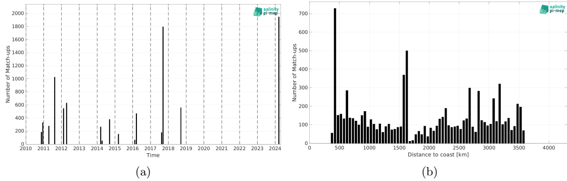
Figure 2: Number of match-ups between TSG (SAMOS) and SMOS SSS L4 OI v346 - Weekly (CMEMS-CATDS-LOPS) SSS as a function of time (a) and as function of the distance to coast (b) over the OTT zone Pi-MEP region and for the full satellite product period.
