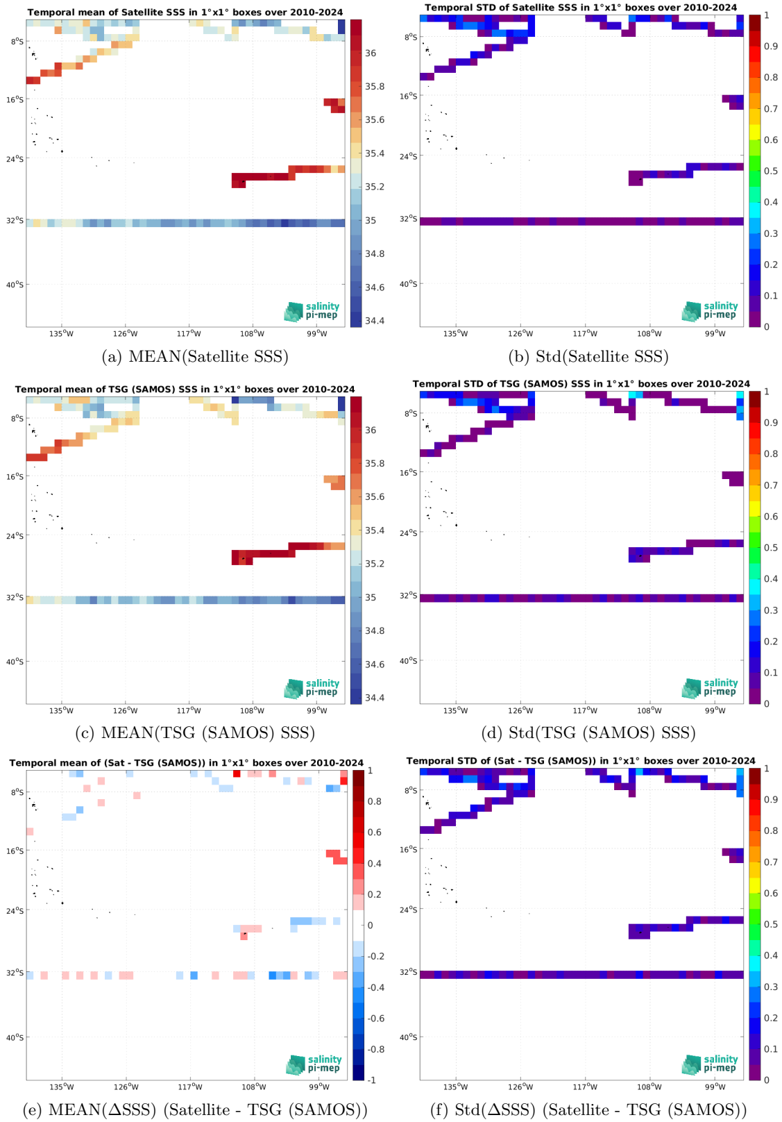
Figure 7: Temporal mean (left) and Std (right) of SSS from SMOS SSS L4 OI v346 - Weekly (CMEMS-CATDS-LOPS) (top), TSG (SAMOS) (middle), and of \Delta SSS (Satellite - TSG (SAMOS)). Only match-up pairs are used to generate these maps.
