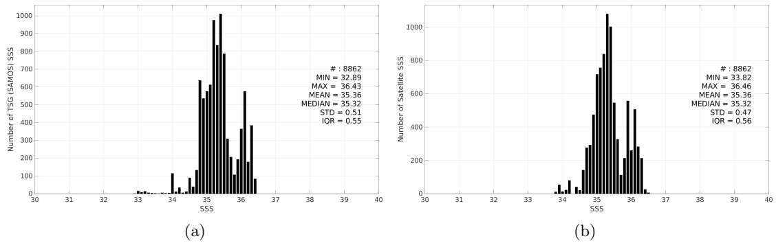
Figure 3: Histograms of SSS from TSG (SAMOS) (a) and SMOS SSS L4 OI v346 - Weekly (CMEMS-CATDS-LOPS) (b) considering all match-up pairs per bins of 0.1 over the OTT zone Pi-MEP region and for the full satellite product period.
