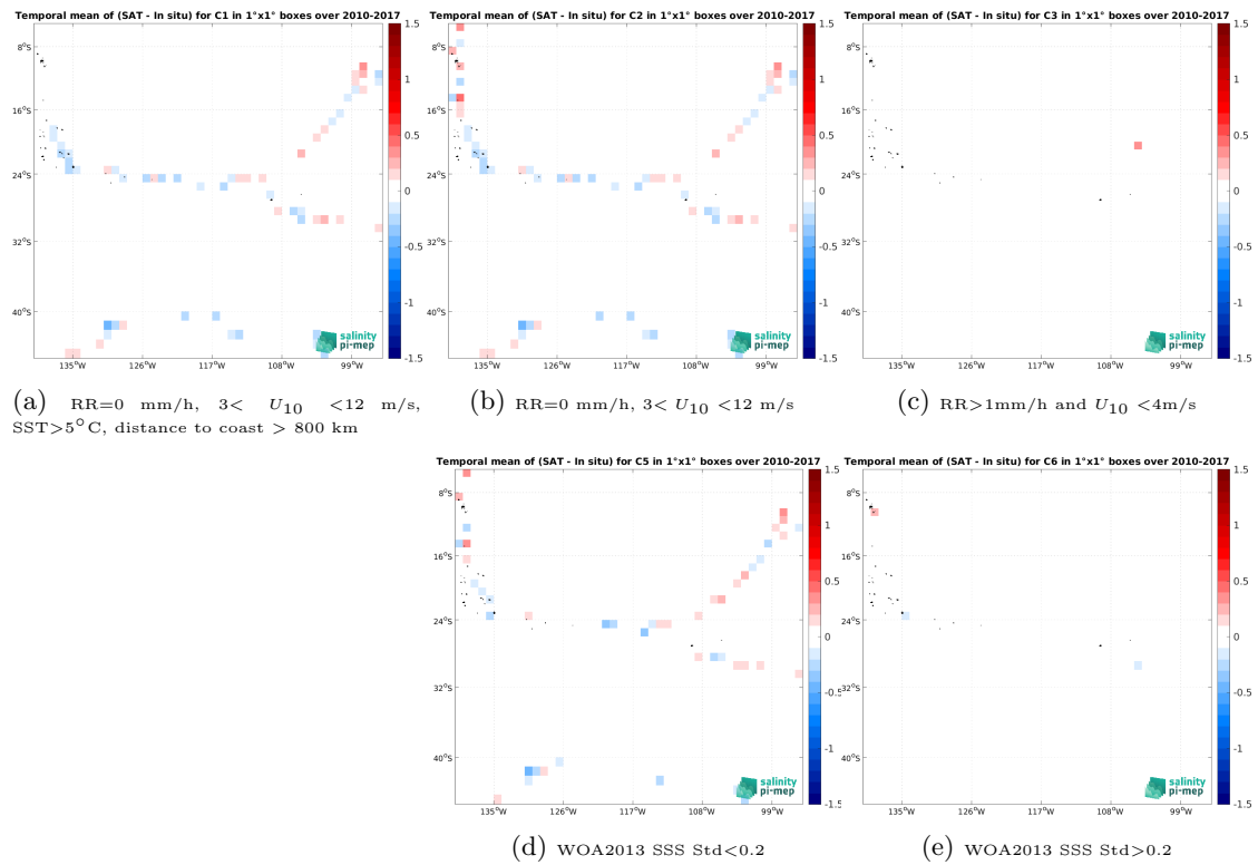
Figure 14: Temporal mean gridded over spatial boxes of size 1^\circ \times 1^\circ of \Delta SSS (SMOS SSS L4 OI v346 - Weekly (CMEMS-CATDS-LOPS) - TSG (GOSUD-Sailing-ship)) for 5 different sub-datasets corresponding to:RR=0 mm/h, 3 < U_{10} < 12 m/s, SST >5^\circ\text{C} , distance to coast > 800 km (a), RR=0 mm/h, 3 < U_{10} < 12 m/s (b), RR >1 mm/h and U_{10} < 4 m/s (c), WOA2013 SSS Std <0.2 (d), WOA2013 SSS Std >0.2 (e).
