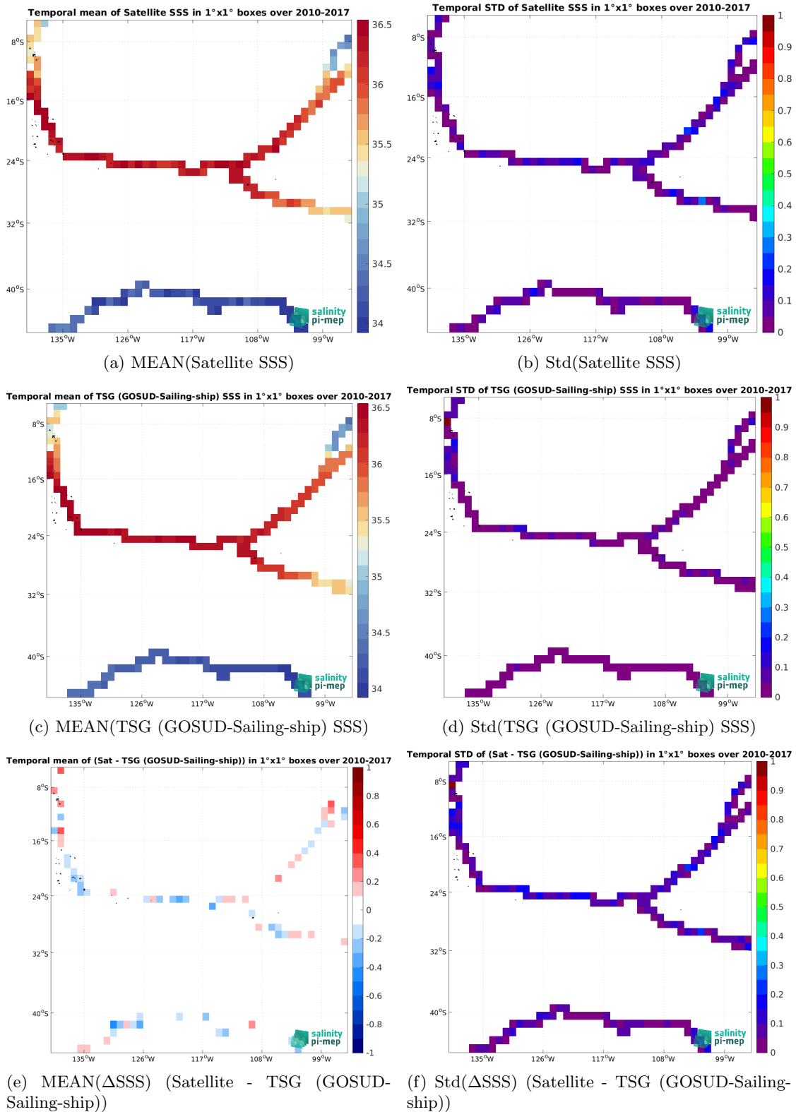
Figure 7: Temporal mean (left) and Std (right) of SSS from SMOS SSS L4 OI v346 - Weekly (CMEMS-CATDS-LOPS) (top), TSG (GOSUD-Sailing-ship) (middle), and of \Delta SSS (Satellite - TSG (GOSUD-Sailing-ship)). Only match-up pairs are used to generate these maps.
