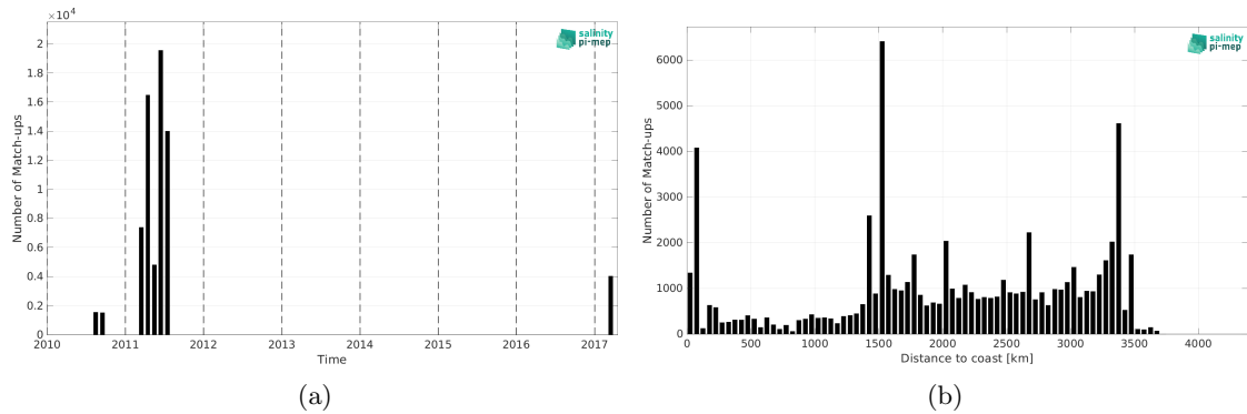
Figure 2: Number of match-ups between TSG (GOSUD-Sailing-ship) and SMOS SSS L4 OI v346 - Weekly (CMEMS-CATDS-LOPS) SSS as a function of time (a) and as function of the distance to coast (b) over the OTT zone Pi-MEP region and for the full satellite product period.
