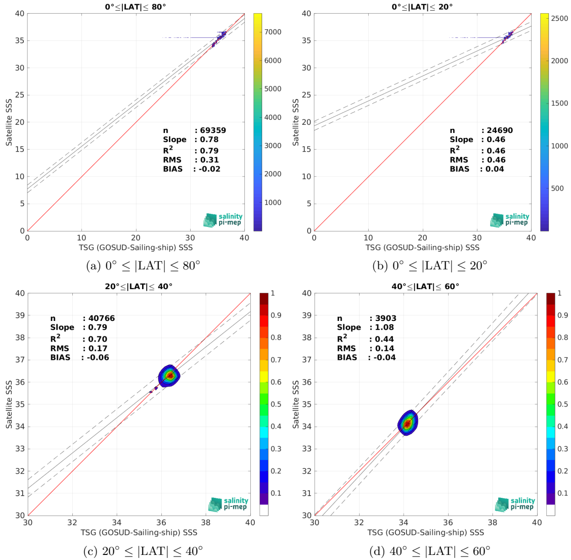
Figure 10: Contour maps of the concentration of SMOS SSS L4 OI v346 - Weekly (CMEMS-CATDS-LOPS) SSS (y-axis) versus TSG (GOSUD-Sailing-ship) SSS (x-axis) at match-up pairs for different latitude bands. For each plot, the red line shows x=y . The black thin and dashed lines indicate a linear fit through the data cloud and the \pm 95\% confidence levels, respectively. The number match-up pairs n , the slope and R^2 coefficient of the linear fit, the root mean square (RMS) and the mean bias between satellite and in situ data are indicated for each latitude band in each plots.
