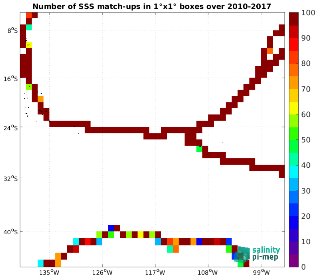
Figure 5: Number of SSS match-ups between TSG (GOSUD-Sailing-ship) SSS and the SMOS SSS L4 OI v346 - Weekly (CMEMS-CATDS-LOPS) SSS product for the OTT zone Pi-MEP region over 1^\circ \times 1^\circ boxes and for the full satellite product period.
