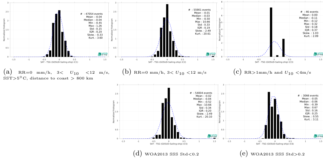
Figure 15: Normalized histogram of \Delta SSS (SMOS SSS L4 OI v346 - Weekly (CMEMS-CATDS-LOPS) - TSG (GOSUD-Sailing-ship)) for 5 different subdatasets corresponding to: RR=0 mm/h, 3 < U_{10} < 12 m/s, SST>5°C, distance to coast > 800 km (a), RR=0 mm/h, 3 < U_{10} < 12 m/s (b), RR>1mm/h and U_{10} < 4 m/s (c), WOA2013 SSS Std<0.2 (d), WOA2013 SSS Std>0.2 (e).
