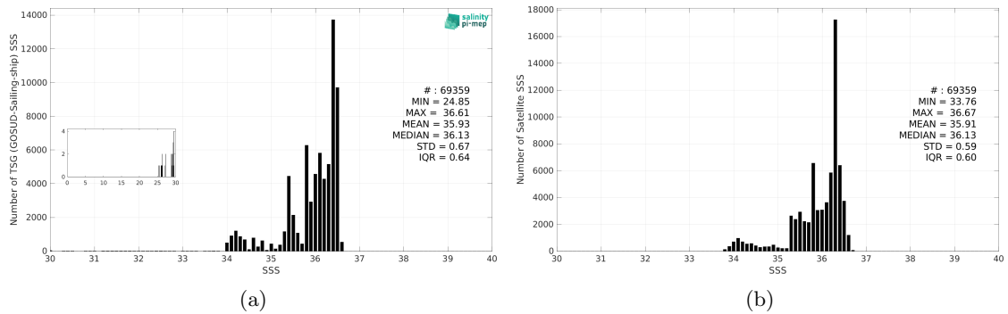
Figure 3: Histograms of SSS from TSG (GOSUD-Sailing-ship) (a) and SMOS SSS L4 OI v346 - Weekly (CMEMS-CATDS-LOPS) (b) considering all match-up pairs per bins of 0.1 over the OTT zone Pi-MEP region and for the full satellite product period.
