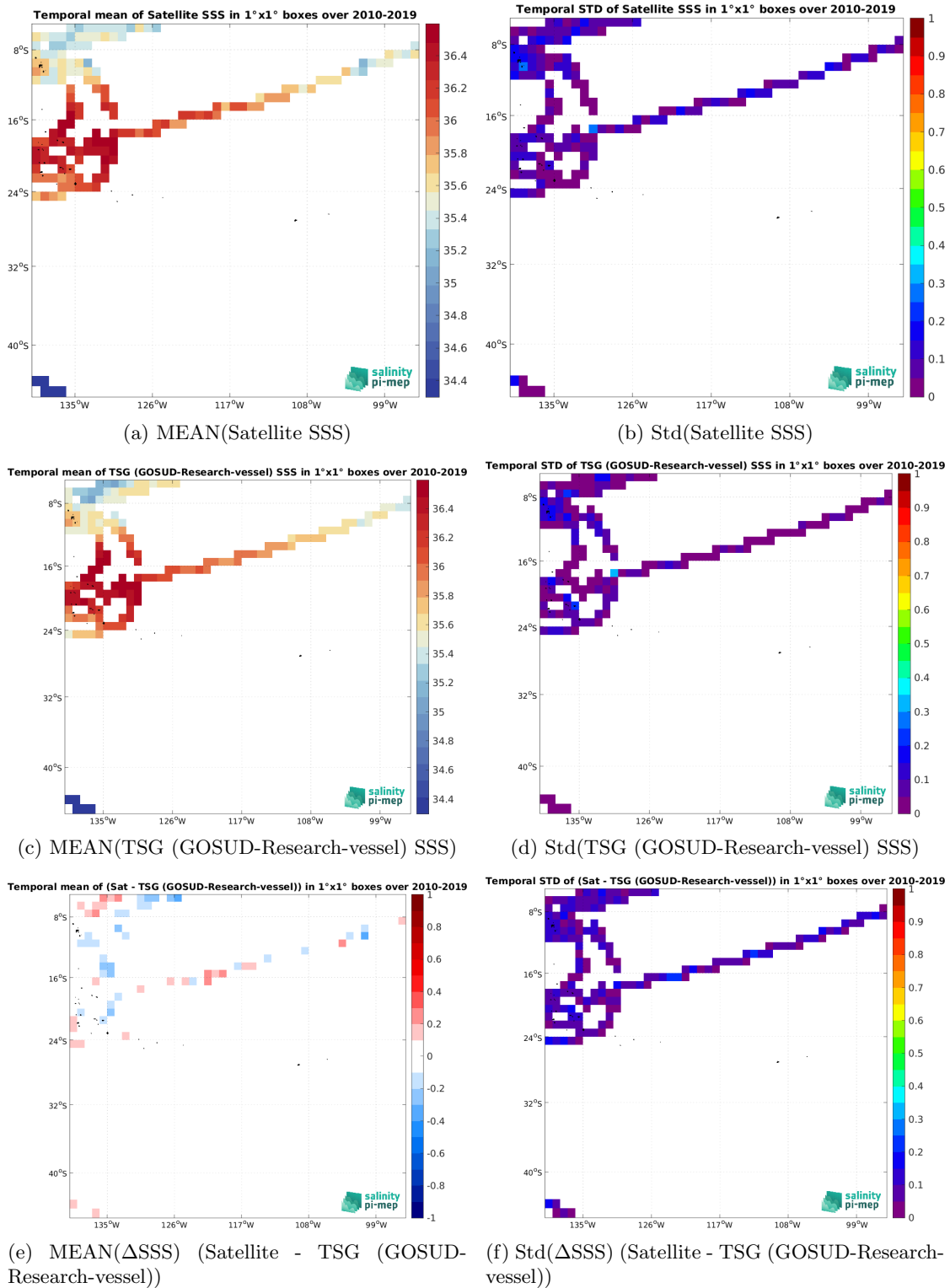
Figure 7: Temporal mean (left) and Std (right) of SSS from SMOS SSS L4 OI v346 - Weekly (CMEMS-CATDS-LOPS) (top), TSG (GOSUD-Research-vessel) (middle), and of \Delta SSS (Satellite - TSG (GOSUD-Research-vessel)). Only match-up pairs are used to generate these maps.
