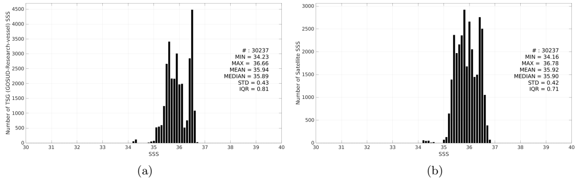
Figure 3: Histograms of SSS from TSG (GOSUD-Research-vessel) (a) and SMOS SSS L4 OI v346 - Weekly (CMEMS-CATDS-LOPS) (b) considering all match-up pairs per bins of 0.1 over the OTT zone Pi-MEP region and for the full satellite product period.
