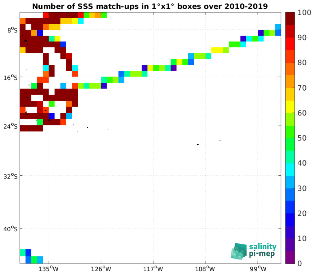
Figure 5: Number of SSS match-ups between TSG (GOSUD-Research-vessel) SSS and the SMOS SSS L4 OI v346 - Weekly (CMEMS-CATDS-LOPS) SSS product for the OTT zone Pi-MEP region over 1^\circ \times 1^\circ boxes and for the full satellite product period.
