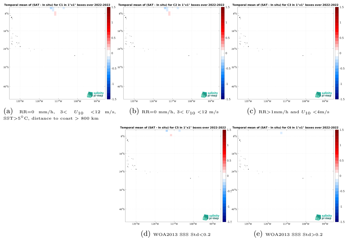
Figure 14: Temporal mean gridded over spatial boxes of size 1^\circ \times 1^\circ of \Delta SSS (SMOS SSS L4 OI v346 - Weekly (CMEMS-CATDS-LOPS) - Saildrone) for 5 different subdatasets corresponding to:RR=0 mm/h, 3 < U_{10} < 12 m/s, SST >5^\circ\text{C} , distance to coast > 800 km (a), RR=0 mm/h, 3 < U_{10} < 12 m/s (b), RR >1 mm/h and U_{10} < 4 m/s (c), WOA2013 SSS Std <0.2 (d), WOA2013 SSS Std >0.2 (e).
