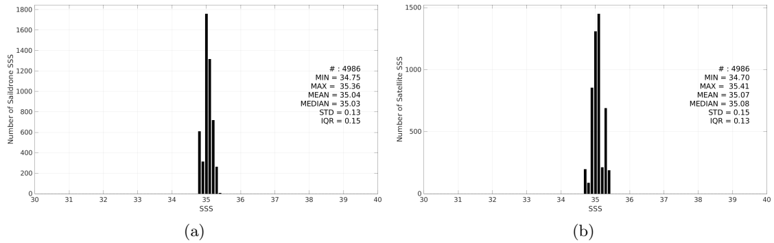
Figure 3: Histograms of SSS from Saildrone (a) and SMOS SSS L4 OI v346 - Weekly (CMEMS-CATDS-LOPS) (b) considering all match-up pairs per bins of 0.1 over the OTT zone Pi-MEP region and for the full satellite product period.
