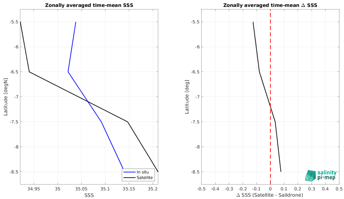
Figure 9: Left panel: Zonal mean SSS from SMOS SSS L4 OI v346 - Weekly (CMEMS-CATDS-LOPS) satellite product (black) and from Sairdrone (blue). Right panel: Zonal mean of \Delta SSS (Satellite - Sairdrone) for all the collected Pi-MEP match-up pairs estimated over the full satellite product period.
