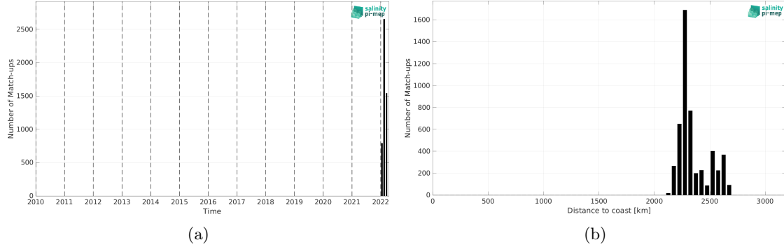
Figure 2: Number of match-ups between Saildrone and SMOS SSS L4 OI v346 - Weekly (CMEMS-CATDS-LOPS) SSS as a function of time (a) and as function of the distance to coast (b) over the OTT zone Pi-MEP region and for the full satellite product period.
