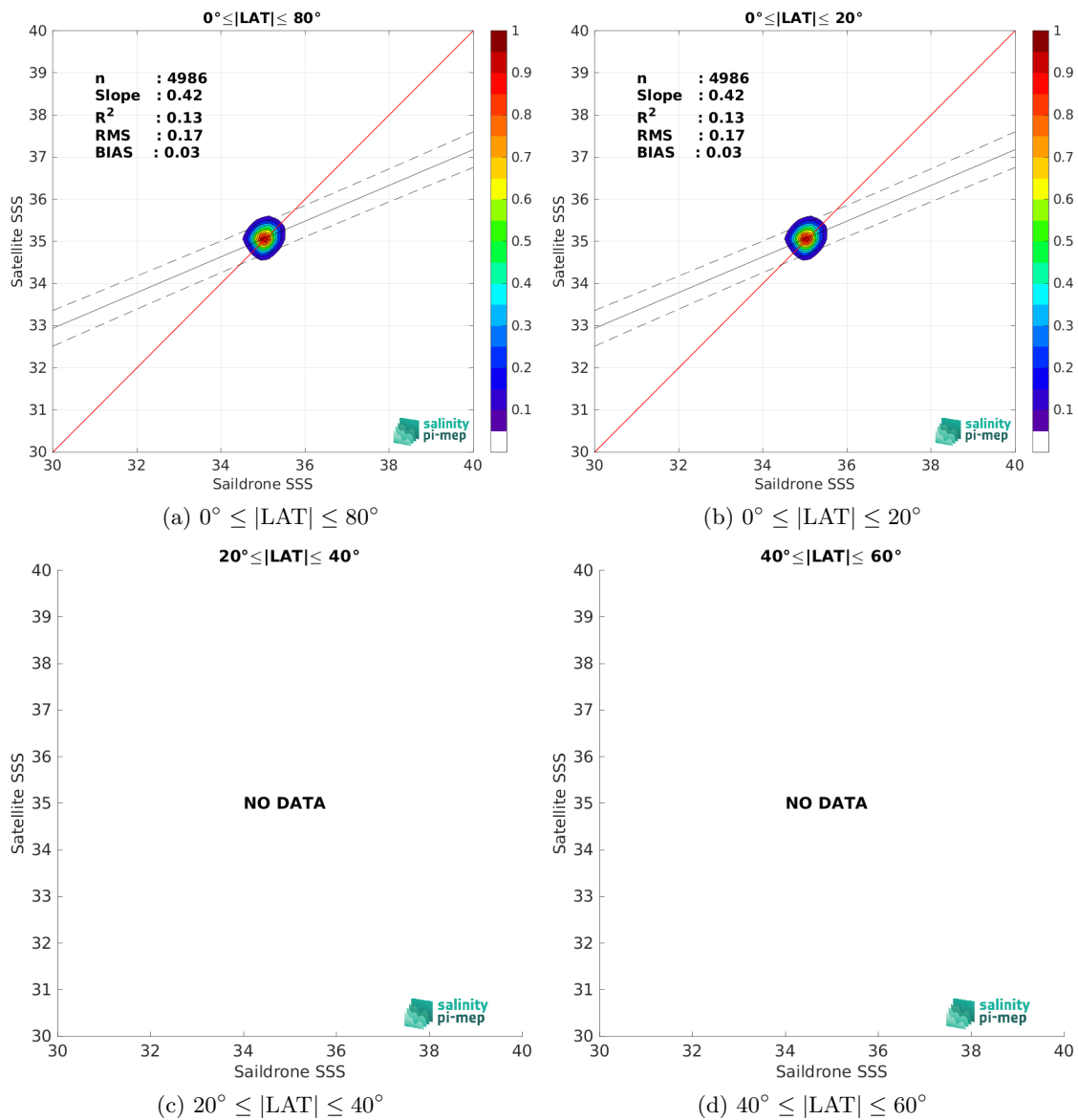
Figure 10: Contour maps of the concentration of SMOS SSS L4 OI v346 - Weekly (CMEMS-CATDS-LOPS) SSS (y-axis) versus Saildrone SSS (x-axis) at match-up pairs for different latitude bands. For each plot, the red line shows x=y . The black thin and dashed lines indicate a linear fit through the data cloud and the \pm 95\% confidence levels, respectively. The number match-up pairs n , the slope and R^2 coefficient of the linear fit, the root mean square (RMS) and the mean bias between satellite and in situ data are indicated for each latitude band in each plots.
