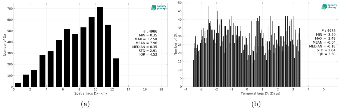
Figure 6: Histograms of the spatial (a) and temporal (b) lags between the location/time of the Saildrone measurement and the date of the corresponding SMOS SSS L4 OI v346 - Weekly (CMEMS-CATDS-LOPS) SSS pixel.
