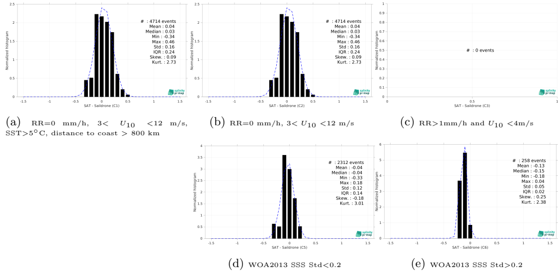
Figure 15: Normalized histogram of \Delta SSS (SMOS SSS L4 OI v346 - Weekly (CMEMS-CATDS-LOPS) - Saildrone) for 5 different subdatasets corresponding to: RR=0 mm/h, 3 < U_{10} < 12 m/s, SST > 5°C, distance to coast > 800 km (a), RR=0 mm/h, 3 < U_{10} < 12 m/s (b), RR > 1mm/h and U_{10} < 4 m/s (c), WOA2013 SSS Std < 0.2 (d), WOA2013 SSS Std > 0.2 (e).
