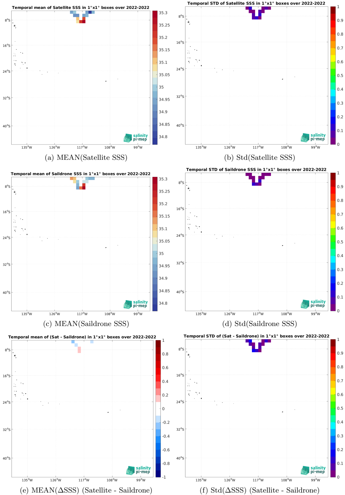
Figure 7: Temporal mean (left) and Std (right) of SSS from SMOS SSS L4 OI v346 - Weekly (CMEMS-CATDS-LOPS) (top), Saildrone (middle), and of \Delta SSS (Satellite - Saildrone). Only match-up pairs are used to generate these maps.
