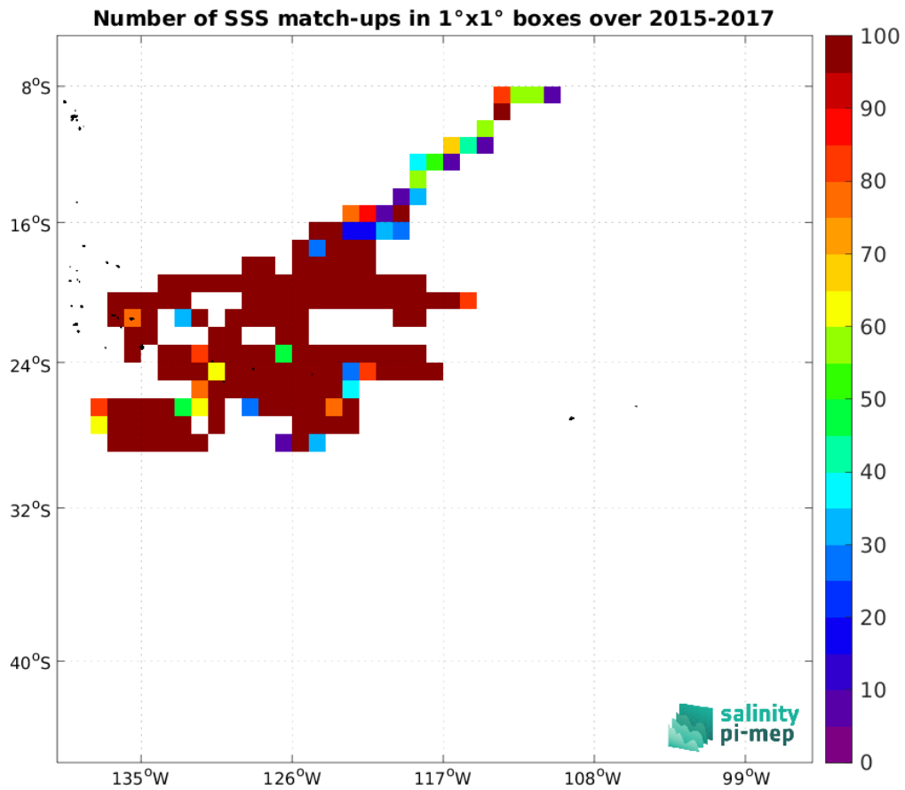
Figure 4: Number of SSS match-ups between Surface drifters SSS and the SMOS SSS L4 OI v346 - Weekly (CMEMS-CATDS-LOPS) SSS product for the OTT zone Pi-MEP region over 1°x1° boxes and for the full satellite product period.
