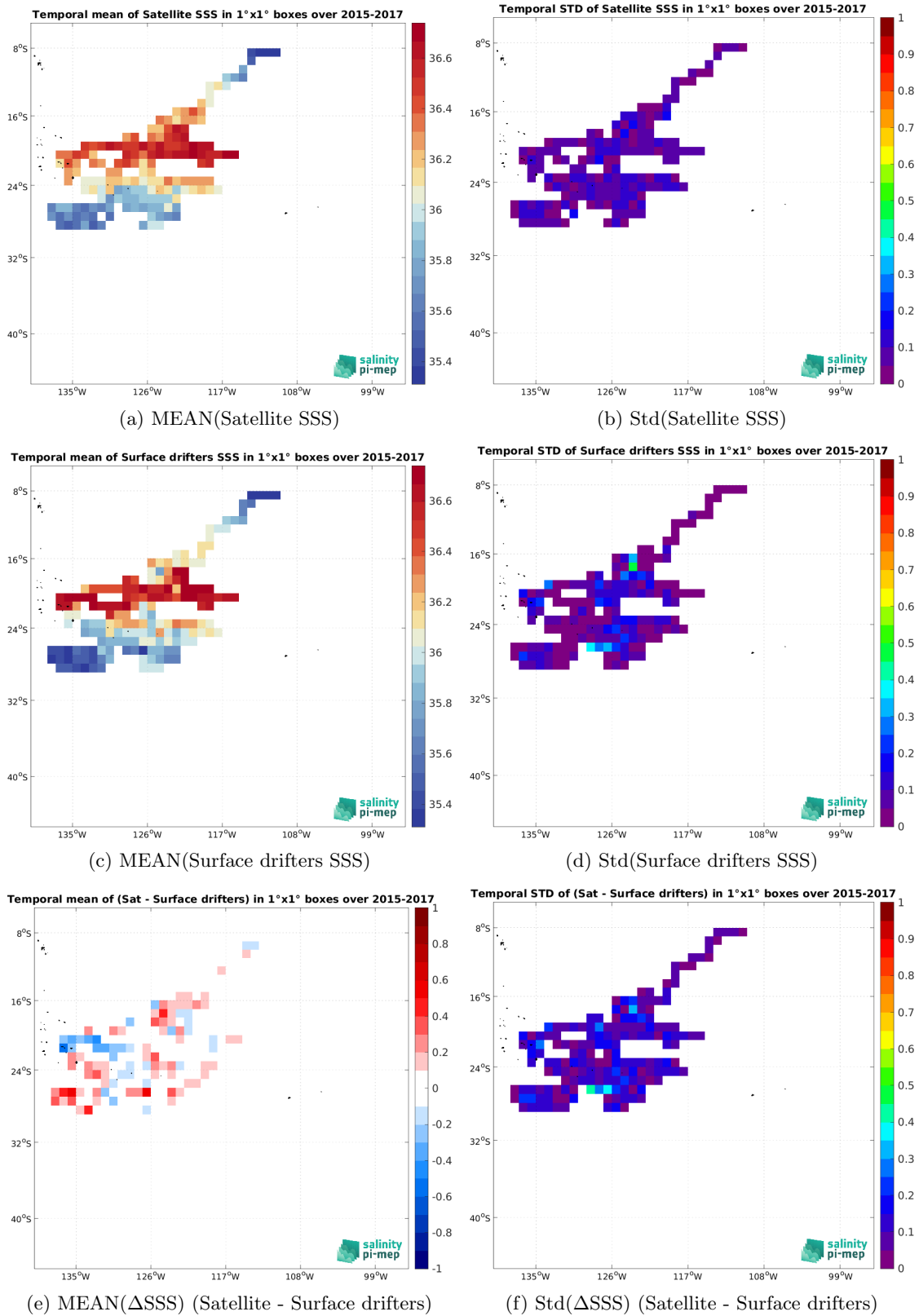
Figure 6: Temporal mean (left) and Std (right) of SSS from SMOS SSS L4 OI v346 - Weekly (CMEMS-CATDS-LOPS) (top), Surface drifters (middle), and of \Delta SSS (Satellite - Surface drifters). Only match-up pairs are used to generate these maps.
