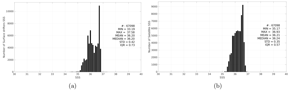
Figure 3: Histograms of SSS from Surface drifters (a) and SMOS SSS L4 OI v346 - Weekly (CMEMS-CATDS-LOPS) (b) considering all match-up pairs per bins of 0.1 over the OTT zone Pi-MEP region and for the full satellite product period.
