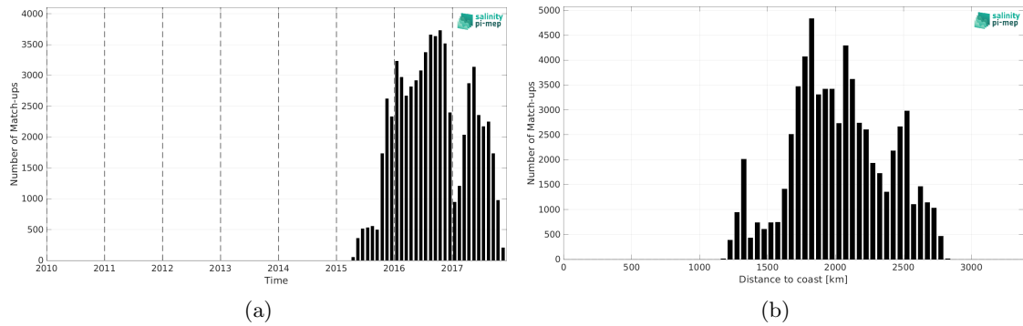
Figure 2: Number of match-ups between Surface drifters and SMOS SSS L4 OI v346 - Weekly (CMEMS-CATDS-LOPS) SSS as a function of time (a) and as function of the distance to coast (b) over the OTT zone Pi-MEP region and for the full satellite product period.
