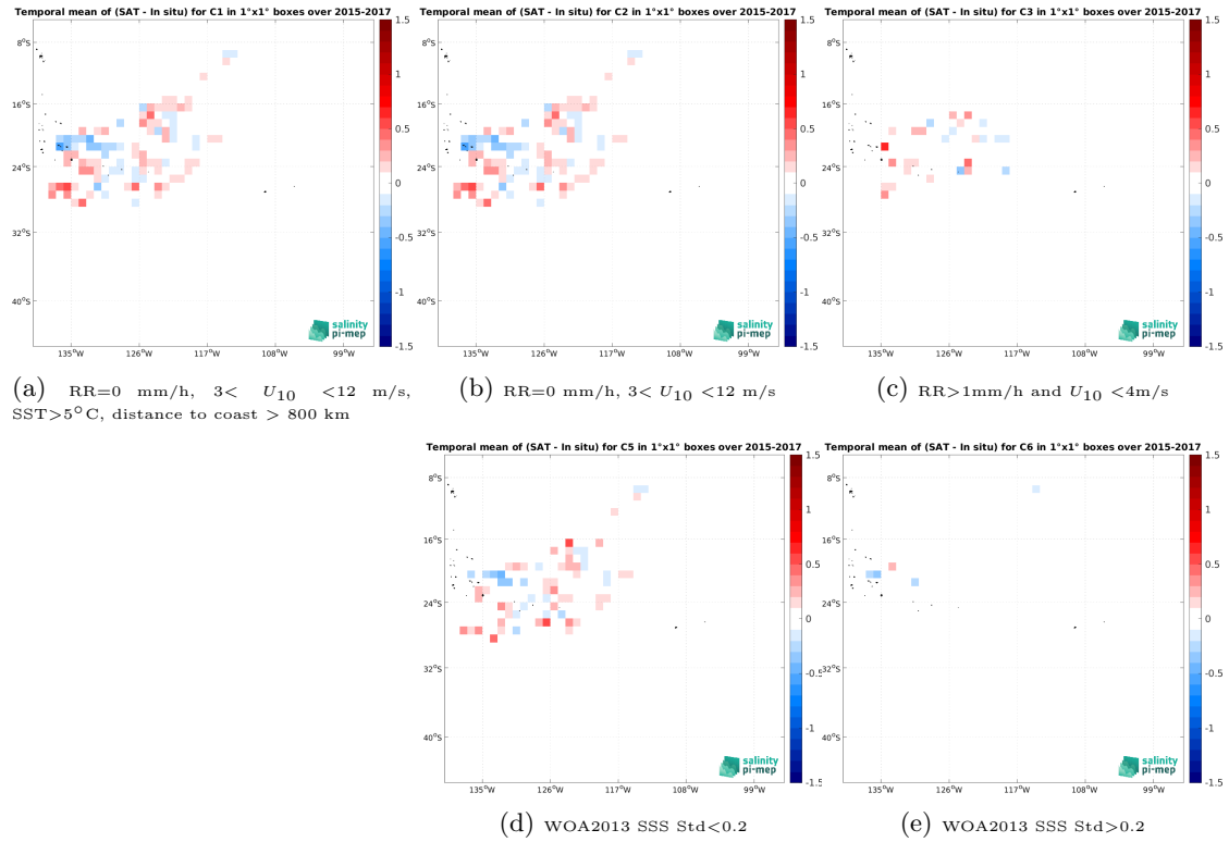
Figure 13: Temporal mean gridded over spatial boxes of size 1^\circ \times 1^\circ of \Delta SSS (SMOS SSS L4 OI v346 - Weekly (CMEMS-CATDS-LOPS) - Surface drifters) for 5 different subdatasets corresponding to: RR=0 mm/h, 3 < U_{10} < 12 m/s, SST > 5^\circ\text{C} , distance to coast > 800 km (a), RR=0 mm/h, 3 < U_{10} < 12 m/s (b), RR > 1 mm/h and U_{10} < 4 m/s (c), WOA2013 SSS Std < 0.2 (d), WOA2013 SSS Std > 0.2 (e).
