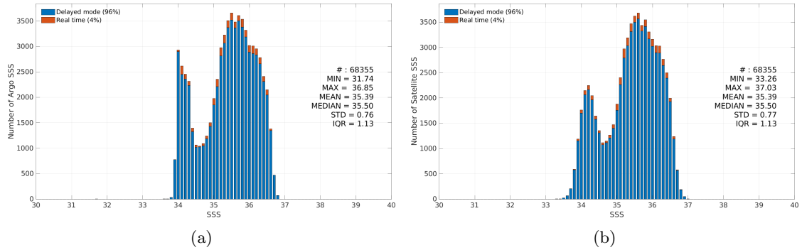
Figure 3: Histograms of SSS from Argo (a) and SMOS SSS L4 OI v346 - Weekly (CMEMS-CATDS-LOPS) (b) considering all match-up pairs per bins of 0.1 over the OTT zone Pi-MEP region and for the full satellite product period.
