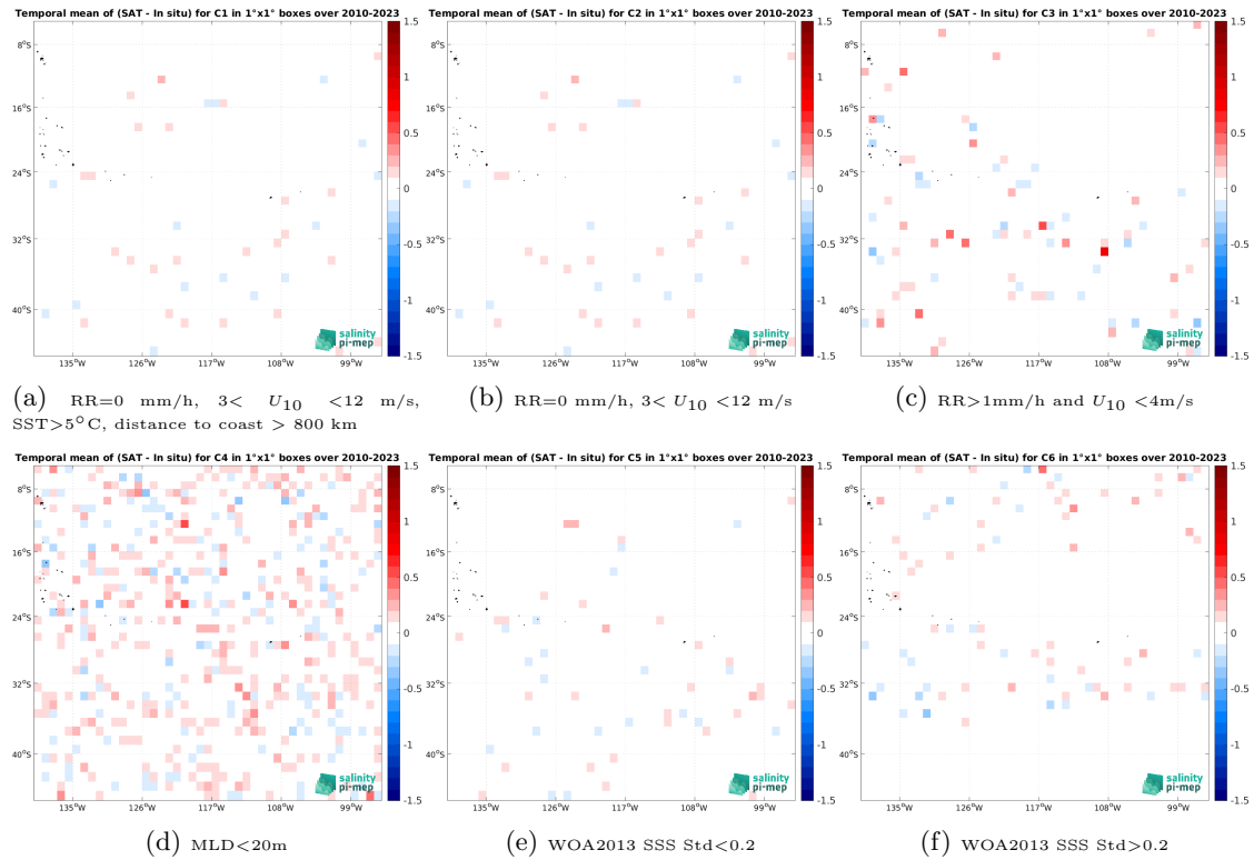
Figure 14: Temporal mean gridded over spatial boxes of size 1^\circ \times 1^\circ of \Delta SSS (SMOS SSS L4 OI v346 - Weekly (CMEMS-CATDS-LOPS) - Argo) for 6 different subdatasets corresponding to: RR=0 mm/h, 3 < U_{10} < 12 m/s, SST > 5^\circ C , distance to coast > 800 km (a), RR=0 mm/h, 3 < U_{10} < 12 m/s (b), RR > 1 mm/h and U_{10} < 4 m/s (c), MLD < 20 m (d), WOA2013 SSS Std < 0.2 (e), WOA2013 SSS Std > 0.2 (f).
