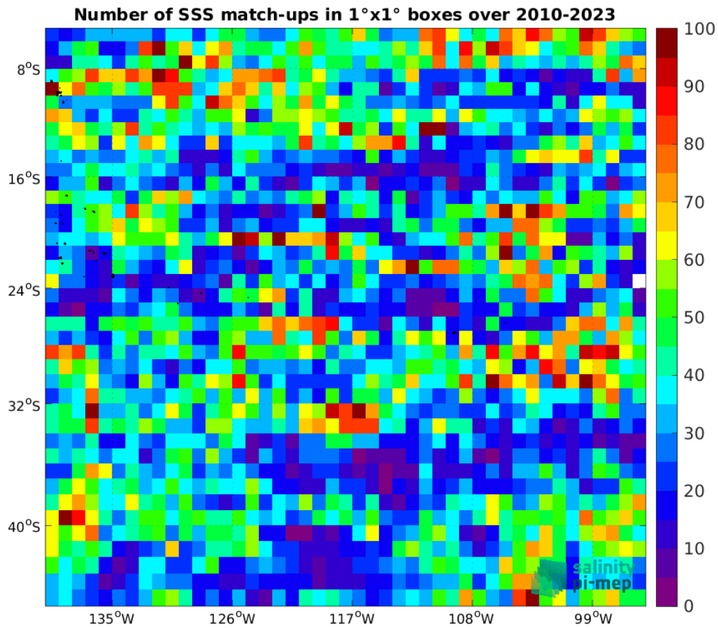
Figure 5: Number of SSS match-ups between Argo SSS and the SMOS SSS L4 OI v346 - Weekly (CMEMS-CATDS-LOPS) SSS product for the OTT zone Pi-MEP region over 1°x1° boxes and for the full satellite product period.
