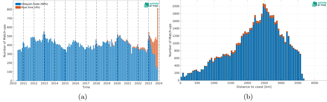
Figure 2: Number of match-ups between Argo and SMOS SSS L4 OI v346 - Weekly (CMEMS-CATDS-LOPS) SSS as a function of time (a) and as function of the distance to coast (b) over the OTT zone Pi-MEP region and for the full satellite product period.
