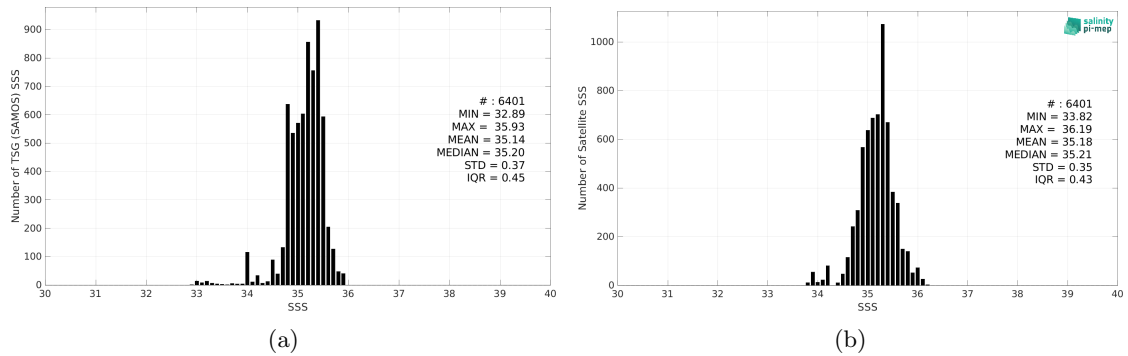
Figure 2: Histograms of SSS from TSG (SAMOS) (a) and SMOS SSS L4 OI v342 - Weekly (CMEMS-CATDS-LOPS) (b) considering all match-up pairs per bins of 0.1 over the OTT zone Pi-MEP region and for the full satellite product period.
