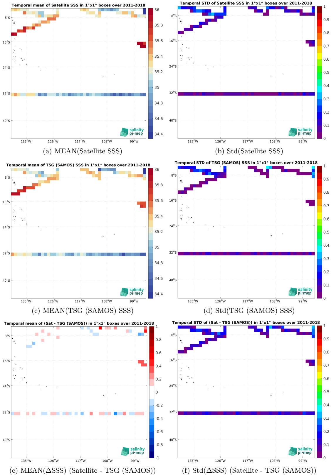
Figure 6: Temporal mean (left) and Std (right) of SSS from SMOS SSS L4 OI v342 - Weekly (CMEMS-CATDS-LOPS) (top), TSG (SAMOS) (middle), and of \Delta SSS (Satellite - TSG (SAMOS)). Only match-up pairs are used to generate these maps.
