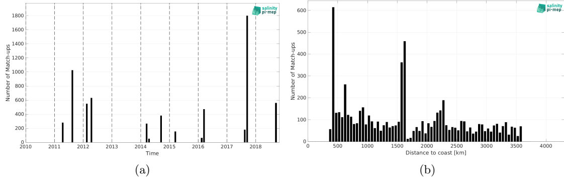
Figure 1: Number of match-ups between TSG (SAMOS) and SMOS SSS L4 OI v342 - Weekly (CMEMS-CATDS-LOPS) SSS as a function of time (a) and as function of the distance to coast (b) over the OTT zone Pi-MEP region and for the full satellite product period.
