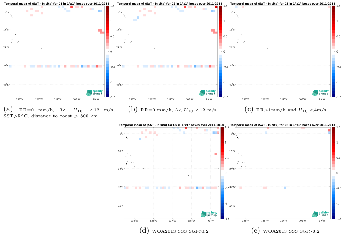
Figure 12: Temporal mean gridded over spatial boxes of size 1^{\circ}\times 1^{\circ} of \Delta\text{SSS} (SMOS SSS L4 OI v342 - Weekly (CMEMS-CATDS-LOPS) - TSG (SAMOS)) for 5 different subdatasets corresponding to: \text{RR}=0 mm/h, 3 < U_{10} < 12 m/s, \text{SST}>5^{\circ}\text{C} , distance to coast > 800 km (a), \text{RR}=0 mm/h, 3 < U_{10} < 12 m/s (b), \text{RR}>1\text{mm/h} and U_{10} < 4\text{m/s} (c), WOA2013 SSS Std < 0.2 (d), WOA2013 SSS Std > 0.2 (e).
