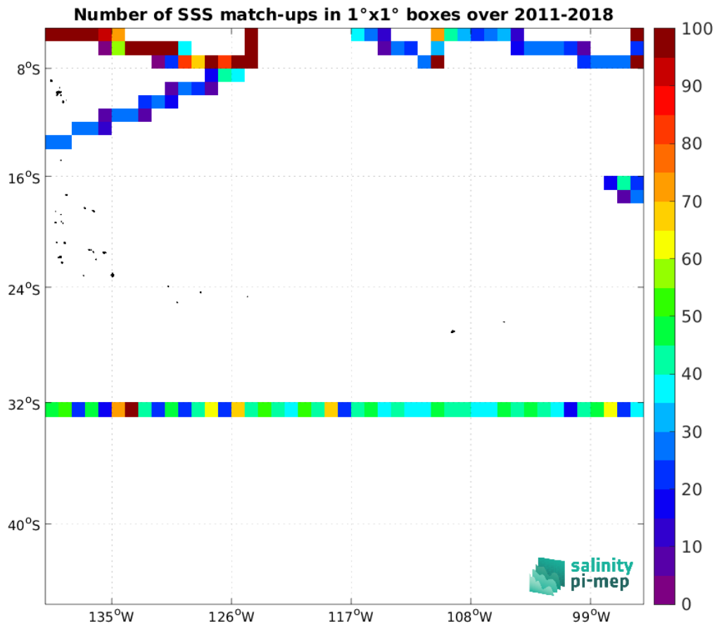
Figure 4: Number of SSS match-ups between TSG (SAMOS) SSS and the SMOS SSS L4 OI v342 - Weekly (CMEMS-CATDS-LOPS) SSS product for the OTT zone Pi-MEP region over 1^\circ \times 1^\circ boxes and for the full satellite product period.
