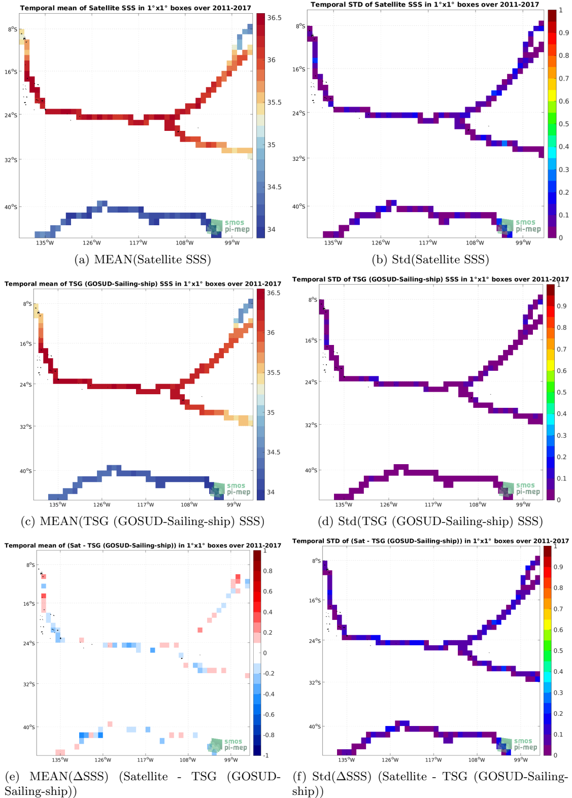
Figure 6: Temporal mean (left) and Std (right) of SSS from SMOS SSS L4 OI v342 - Weekly (CMEMS-CATDS-LOPS) (top), TSG (GOSUD-Sailing-ship) (middle), and of \Delta SSS (Satellite - TSG (GOSUD-Sailing-ship)). Only match-up pairs are used to generate these maps.
