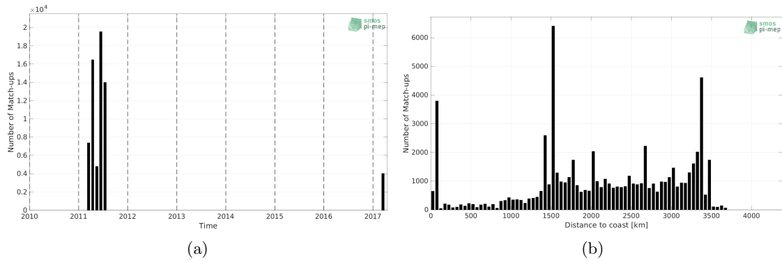
Figure 1: Number of match-ups between TSG (GOSUD-Sailing-ship) and SMOS SSS L4 OI v342 - Weekly (CMEMS-CATDS-LOPS) SSS as a function of time (a) and as function of the distance to coast (b) over the OTT zone Pi-MEP region and for the full satellite product period.
