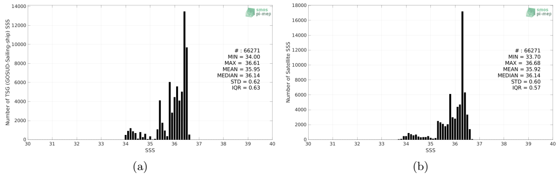
Figure 2: Histograms of SSS from TSG (GOSUD-Sailing-ship) (a) and SMOS SSS L4 OI v342 - Weekly (CMEMS-CATDS-LOPS) (b) considering all match-up pairs per bins of 0.1 over the OTT zone Pi-MEP region and for the full satellite product period.
