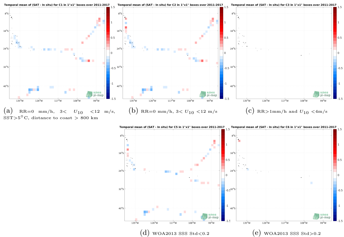
Figure 12: Temporal mean gridded over spatial boxes of size 1^\circ \times 1^\circ of \Delta SSS (SMOS SSS L4 OI v342 - Weekly (CMEMS-CATDS-LOPS) - TSG (GOSUD-Sailing-ship)) for 5 different sub-datasets corresponding to:RR=0 mm/h, 3 < U_{10} < 12 m/s, SST>5°C, distance to coast > 800 km (a), RR=0 mm/h, 3 < U_{10} < 12 m/s (b), RR>1mm/h and U_{10} < 4 m/s (c), WOA2013 SSS Std<0.2 (d), WOA2013 SSS Std>0.2 (e).
