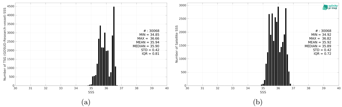
Figure 2: Histograms of SSS from TSG (GOSUD-Research-vessel) (a) and SMOS SSS L4 OI v342 - Weekly (CMEMS-CATDS-LOPS) (b) considering all match-up pairs per bins of 0.1 over the OTT zone Pi-MEP region and for the full satellite product period.
