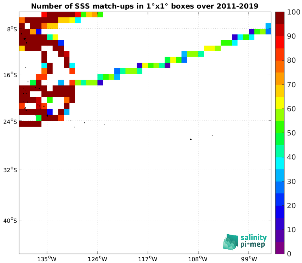
Figure 4: Number of SSS match-ups between TSG (GOSUD-Research-vessel) SSS and the SMOS SSS L4 OI v342 - Weekly (CMEMS-CATDS-LOPS) SSS product for the OTT zone Pi-MEP region over 1^{\circ} \times 1^{\circ} boxes and for the full satellite product period.
