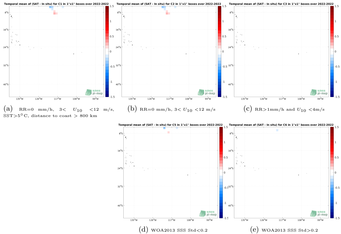
Figure 12: Temporal mean gridded over spatial boxes of size 1^\circ \times 1^\circ of \Delta SSS (SMOS SSS L4 OI v342 - Weekly (CMEMS-CATDS-LOPS) - Saildrone) for 5 different subdatasets corresponding to:RR=0 mm/h, 3 < U_{10} < 12 m/s, SST >5^\circ C, distance to coast > 800 km (a), RR=0 mm/h, 3 < U_{10} < 12 m/s (b), RR >1 mm/h and U_{10} < 4 m/s (c), WOA2013 SSS Std <0.2 (d), WOA2013 SSS Std >0.2 (e).
