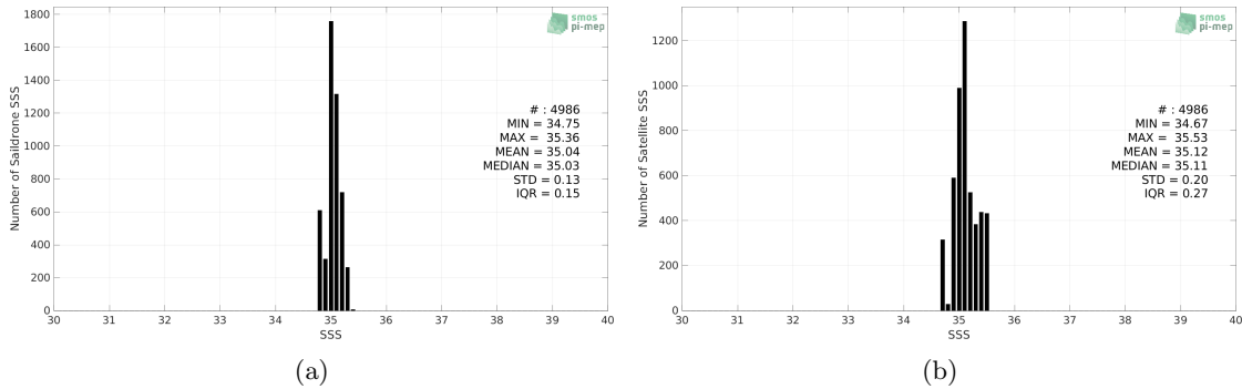
Figure 2: Histograms of SSS from Saildrone (a) and SMOS SSS L4 OI v342 - Weekly (CMEMS-CATDS-LOPS) (b) considering all match-up pairs per bins of 0.1 over the OTT zone Pi-MEP region and for the full satellite product period.
