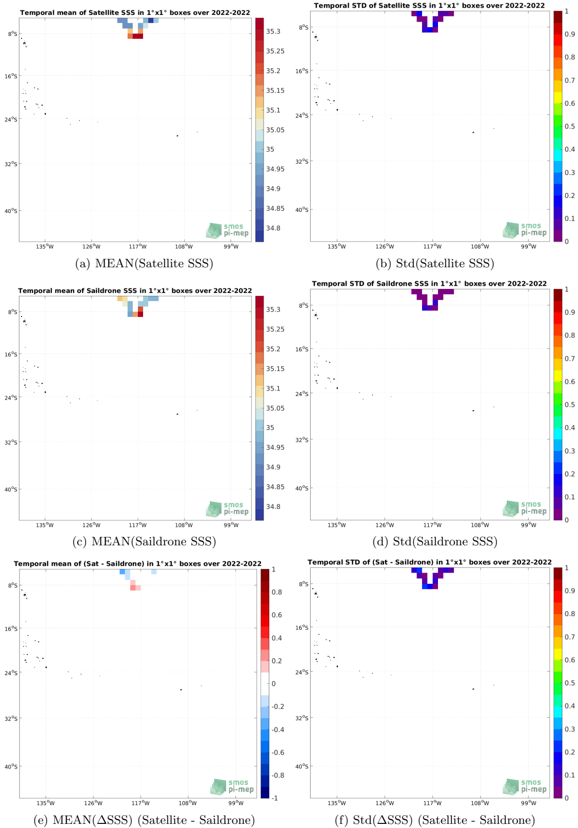
Figure 6: Temporal mean (left) and Std (right) of SSS from SMOS SSS L4 OI v342 - Weekly (CMEMS-CATDS-LOPS) (top), Saildrone (middle), and of \Delta SSS (Satellite - Saildrone). Only match-up pairs are used to generate these maps.
