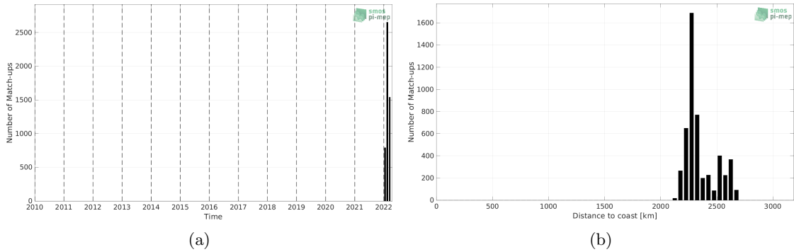
Figure 1: Number of match-ups between Saildrone and SMOS SSS L4 OI v342 - Weekly (CMEMS-CATDS-LOPS) SSS as a function of time (a) and as function of the distance to coast (b) over the OTT zone Pi-MEP region and for the full satellite product period.
