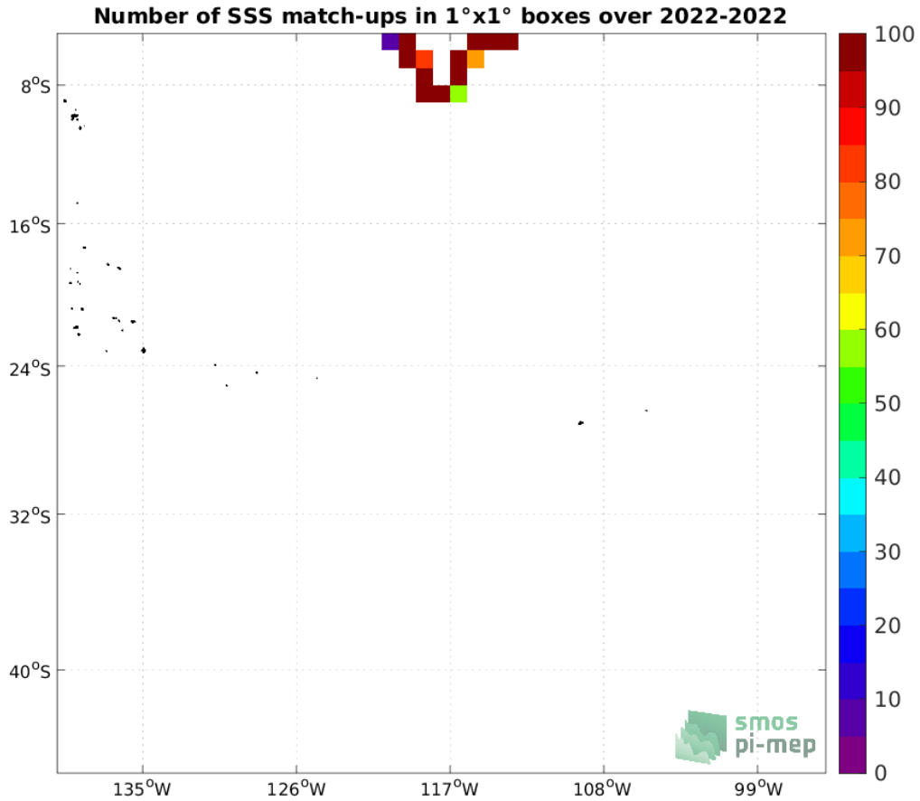
Figure 4: Number of SSS match-ups between Saildrone SSS and the SMOS SSS L4 OI v342 - Weekly (CMEMS-CATDS-LOPS) SSS product for the OTT zone Pi-MEP region over 1°x1° boxes and for the full satellite product period.
