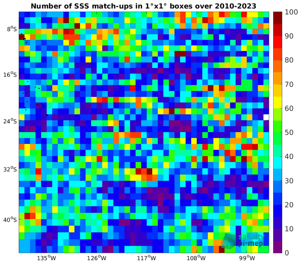
Figure 4: Number of SSS match-ups between Argo SSS and the SMOS SSS L4 OI v342 - Weekly (CMEMS-CATDS-LOPS) SSS product for the OTT zone Pi-MEP region over 1°x1° boxes and for the full satellite product period.
