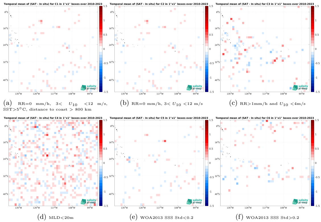
Figure 12: Temporal mean gridded over spatial boxes of size 1^\circ \times 1^\circ of \Delta SSS (SMOS SSS L4 OI v342 - Weekly (CMEMS-CATDS-LOPS) - Argo) for 6 different subdatasets corresponding to:RR=0 mm/h, 3 < U_{10} < 12 m/s, SST >5^\circ\text{C} , distance to coast > 800 km (a), RR=0 mm/h, 3 < U_{10} < 12 m/s (b), RR >1 mm/h and U_{10} < 4 m/s (c),MLD <20 m (d),WOA2013 SSS Std <0.2 (e),WOA2013 SSS Std >0.2 (f).
