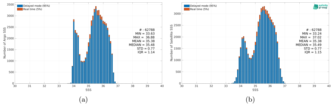
Figure 2: Histograms of SSS from Argo (a) and SMOS SSS L4 OI v342 - Weekly (CMEMS-CATDS-LOPS) (b) considering all match-up pairs per bins of 0.1 over the OTT zone Pi-MEP region and for the full satellite product period.
