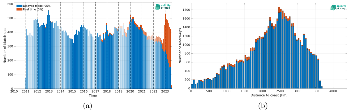
Figure 1: Number of match-ups between Argo and SMOS SSS L4 OI v342 - Weekly (CMEMS-CATDS-LOPS) SSS as a function of time (a) and as function of the distance to coast (b) over the OTT zone Pi-MEP region and for the full satellite product period.
