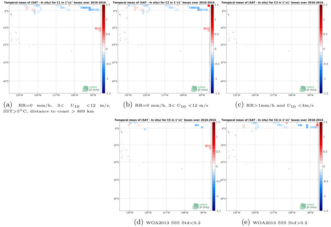
Figure 12: Temporal mean gridded over spatial boxes of size 1^{\circ}\times 1^{\circ} of \Delta\text{SSS} (SMOS L4 v2 Weekly (CATDS-CECOS-IFREMER) - TSG (SAMOS)) for 5 different subdatasets corresponding to:RR=0 mm/h, 3 < U_{10} < 12 m/s, SST >5^{\circ}\text{C} , distance to coast > 800 km (a), RR=0 mm/h, 3 < U_{10} < 12 m/s (b), RR >1 mm/h and U_{10} < 4 m/s (c), WOA2013 SSS Std <0.2 (d), WOA2013 SSS Std >0.2 (e).
