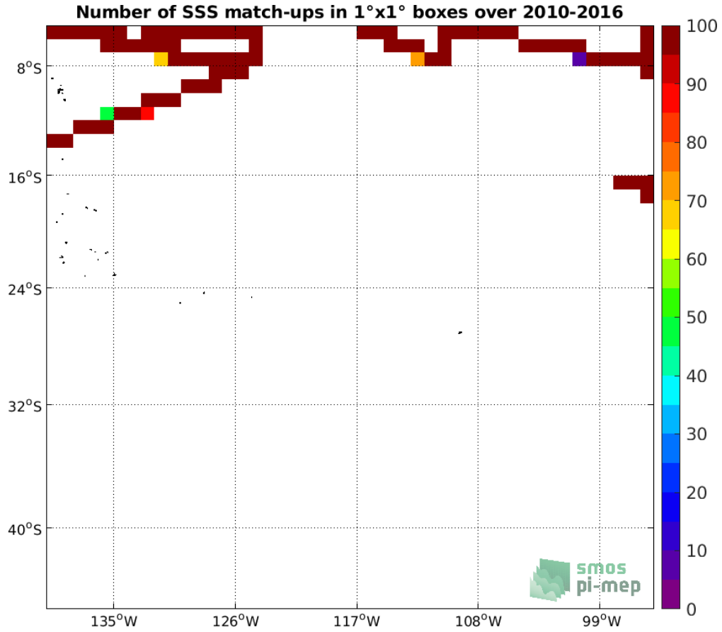
Figure 4: Number of SSS match-ups between TSG (SAMOS) SSS and the SMOS L4 v2 Weekly (CATDS-CECOS-IFREMER) SSS product for the OTT zone Pi-MEP region over 1°x1° boxes and for the full satellite product period.
