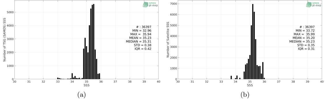
Figure 2: Histograms of SSS from TSG (SAMOS) (a) and SMOS L4 v2 Weekly (CATDS-CECOS-IFREMER) (b) considering all match-up pairs per bins of 0.1 over the OTT zone Pi-MEP region and for the full satellite product period.
