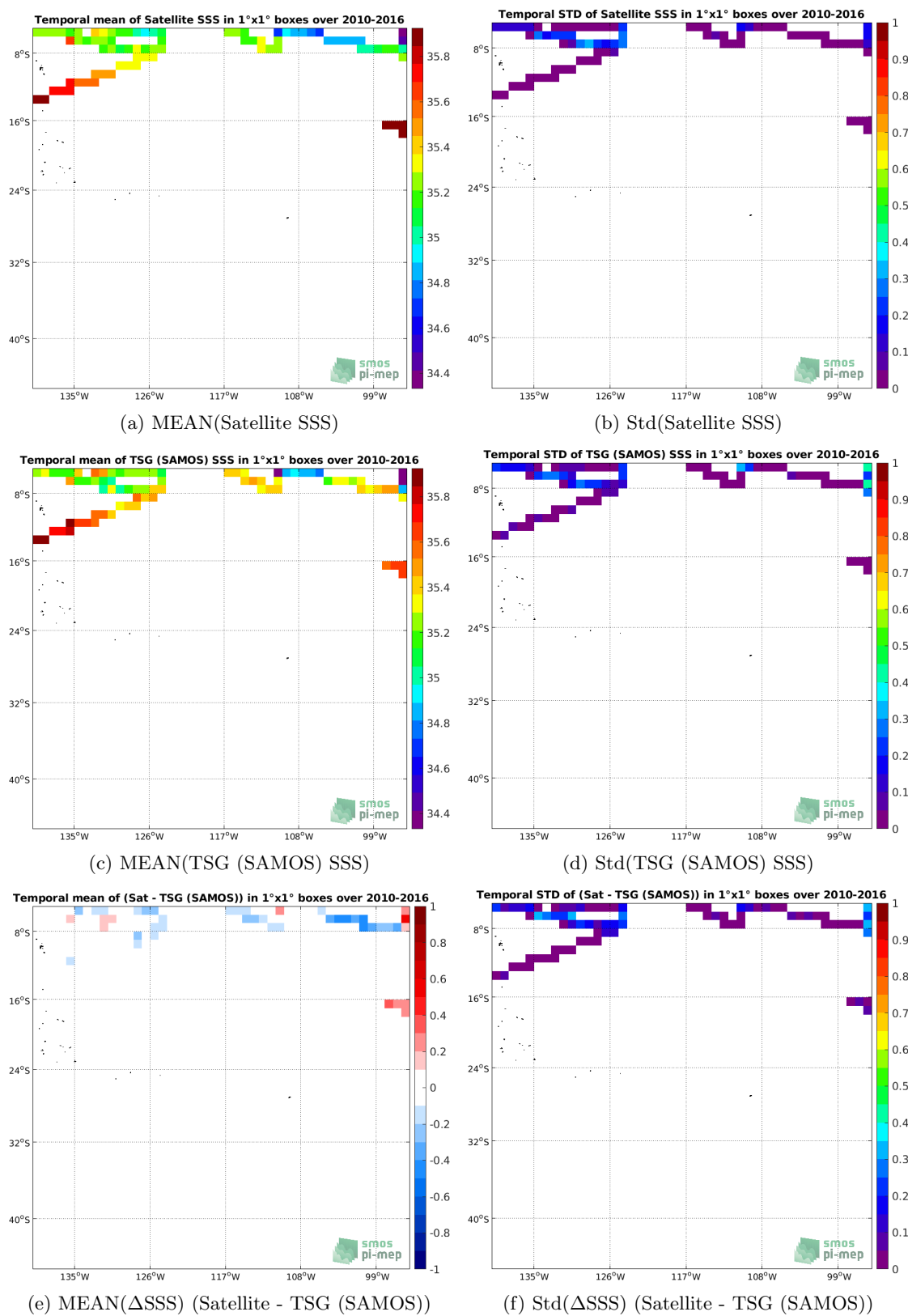
Figure 6: Temporal mean (left) and Std (right) of SSS from SMOS L4 v2 Weekly (CATDS-CECOS-IFREMER) (top), TSG (SAMOS) (middle), and of \Delta SSS (Satellite - TSG (SAMOS)). Only match-up pairs are used to generate these maps.
