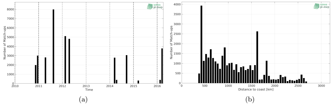
Figure 1: Number of match-ups between TSG (SAMOS) and SMOS L4 v2 Weekly (CATDS-CECOS-IFREMER) SSS as a function of time (a) and as function of the distance to coast (b) over the OTT zone Pi-MEP region and for the full satellite product period.
