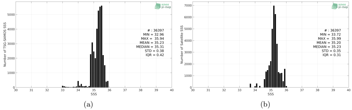
Figure 2: Histograms of SSS from TSG-SAMOS (a) and SMOS-L4-CATDS-CECOS-IFREMER-V2-WEEKLY-0.5DEG (b) considering all match-up pairs per bins of 0.1 over the OTT zone Pi-MEP region and for the full satellite product period.
