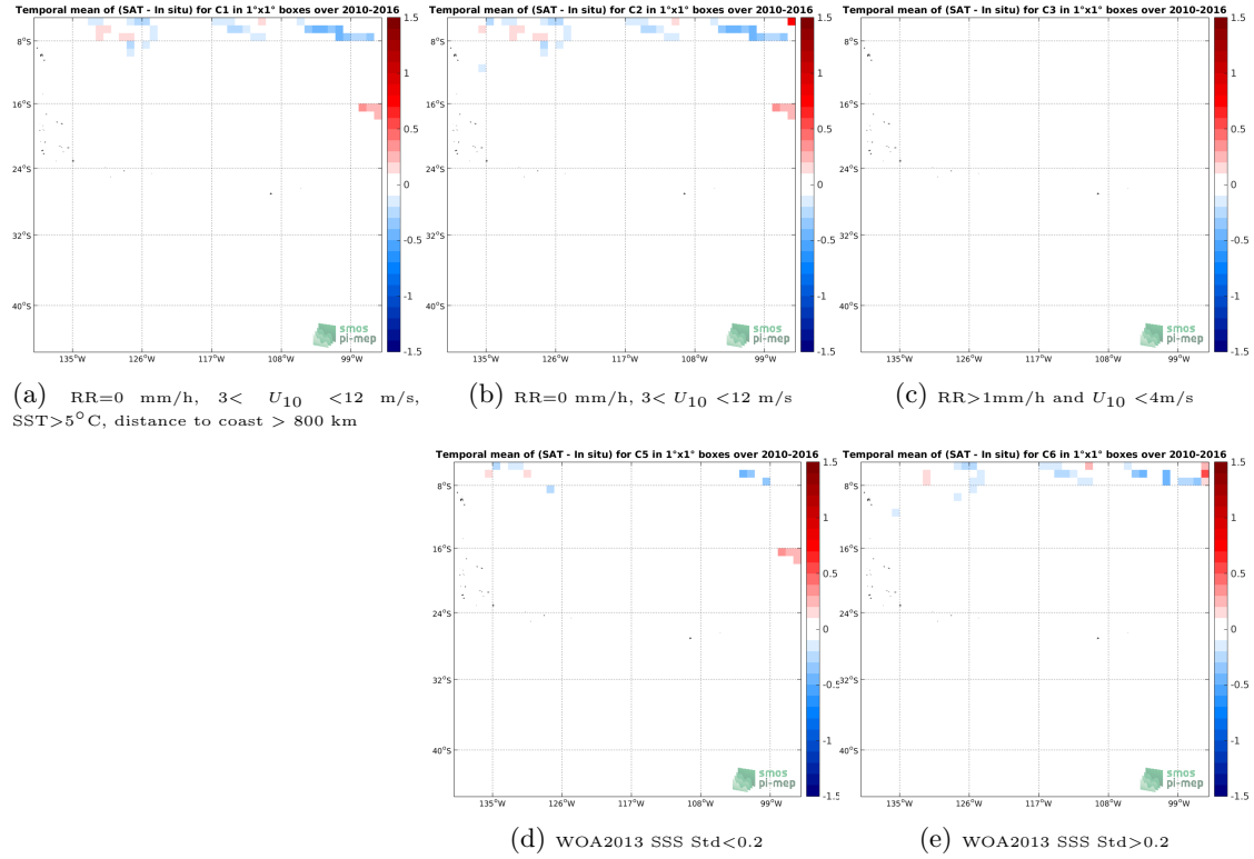
Figure 12: Temporal mean gridded over spatial boxes of size 1^{\circ}\times 1^{\circ} of \Delta\text{SSS} (SMOS-L4-CATDS-CECOS-IFREMER-V2-WEEKLY-0.5DEG - TSG-SAMOS) for 5 different subdatasets corresponding to: \text{RR}=0 mm/h, 3 < U_{10} < 12 m/s, \text{SST} > 5^{\circ}\text{C} , distance to coast > 800 km (a), \text{RR}=0 mm/h, 3 < U_{10} < 12 m/s (b), \text{RR} > 1 mm/h and U_{10} < 4 m/s (c), WOA2013 SSS Std < 0.2 (d), WOA2013 SSS Std > 0.2 (e).
