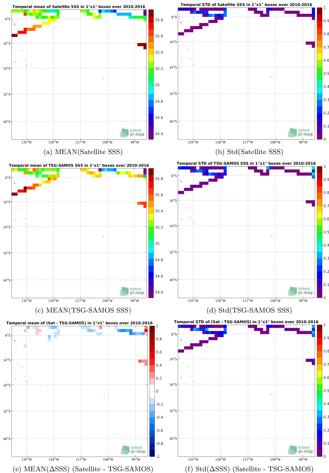
Figure 6: Temporal mean (left) and Std (right) of SSS from SMOS-L4-CATDS-CECOS-IFREMER-V2-WEEKLY-0.5DEG (top), TSG-SAMOS (middle), and of \Delta SSS (Satellite - TSG-SAMOS). Only match-up pairs are used to generate these maps.
