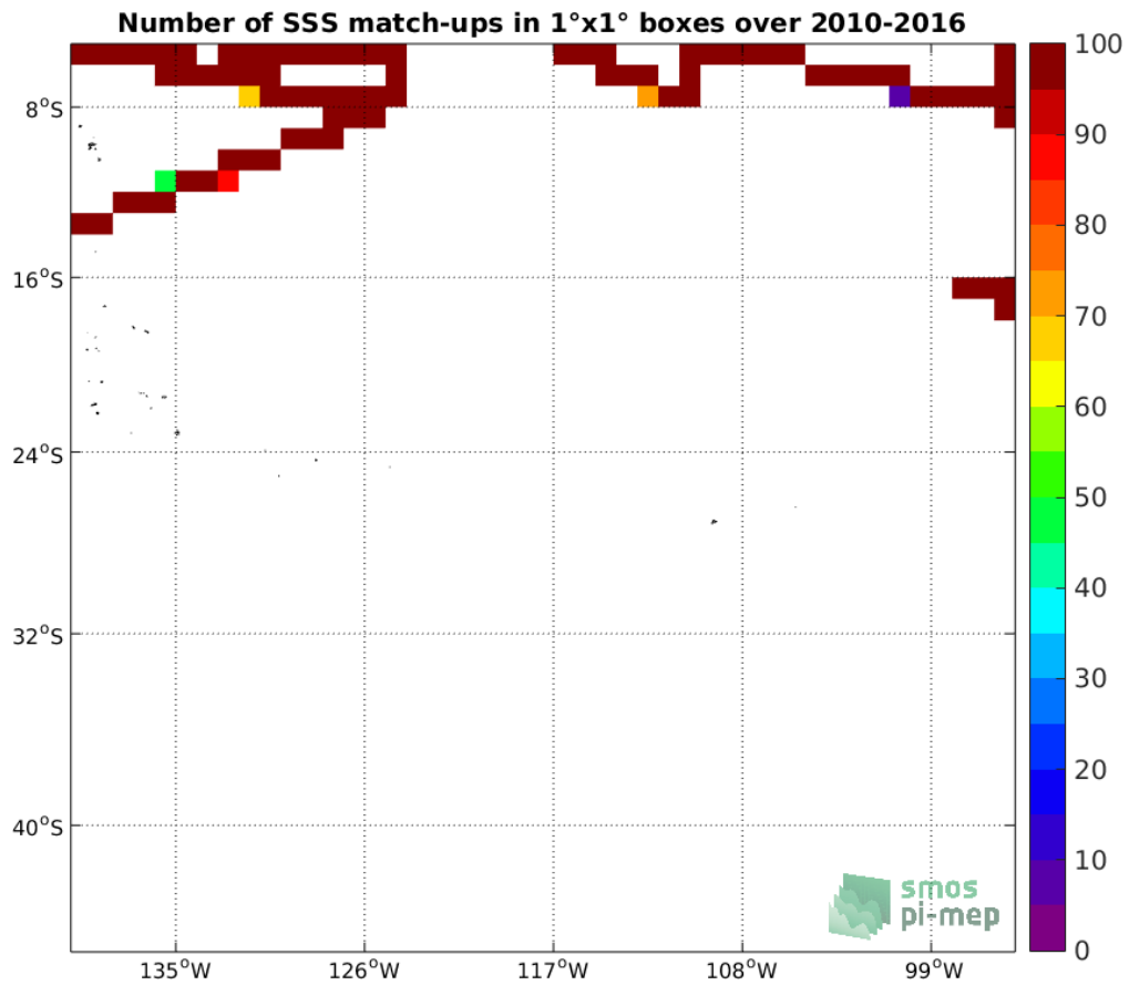
Figure 4: Number of SSS match-ups between TSG-SAMOS SSS and the SMOS-L4-CATDS-CECOS-IFREMER-V2-WEEKLY-0.5DEG SSS product for the OTT zone Pi-MEP region over 1°x1° boxes and for the full satellite product period.
