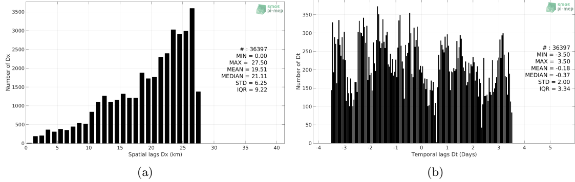
Figure 5: Histograms of the spatial (a) and temporal (b) lags between the time of the TSG-SAMOS measurements and the date of the corresponding SMOS-L4-CATDS-CECOS-IFREMER-V2-WEEKLY-0.5DEG SSS product.
