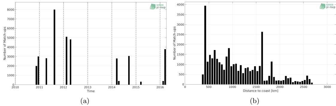
Figure 1: Number of match-ups between TSG-SAMOS and SMOS-L4-CATDS-CECOS-IFREMER-V2-WEEKLY-0.5DEG SSS as a function of time (a) and as function of the distance to coast (b) over the OTT zone Pi-MEP region and for the full satellite product period.
