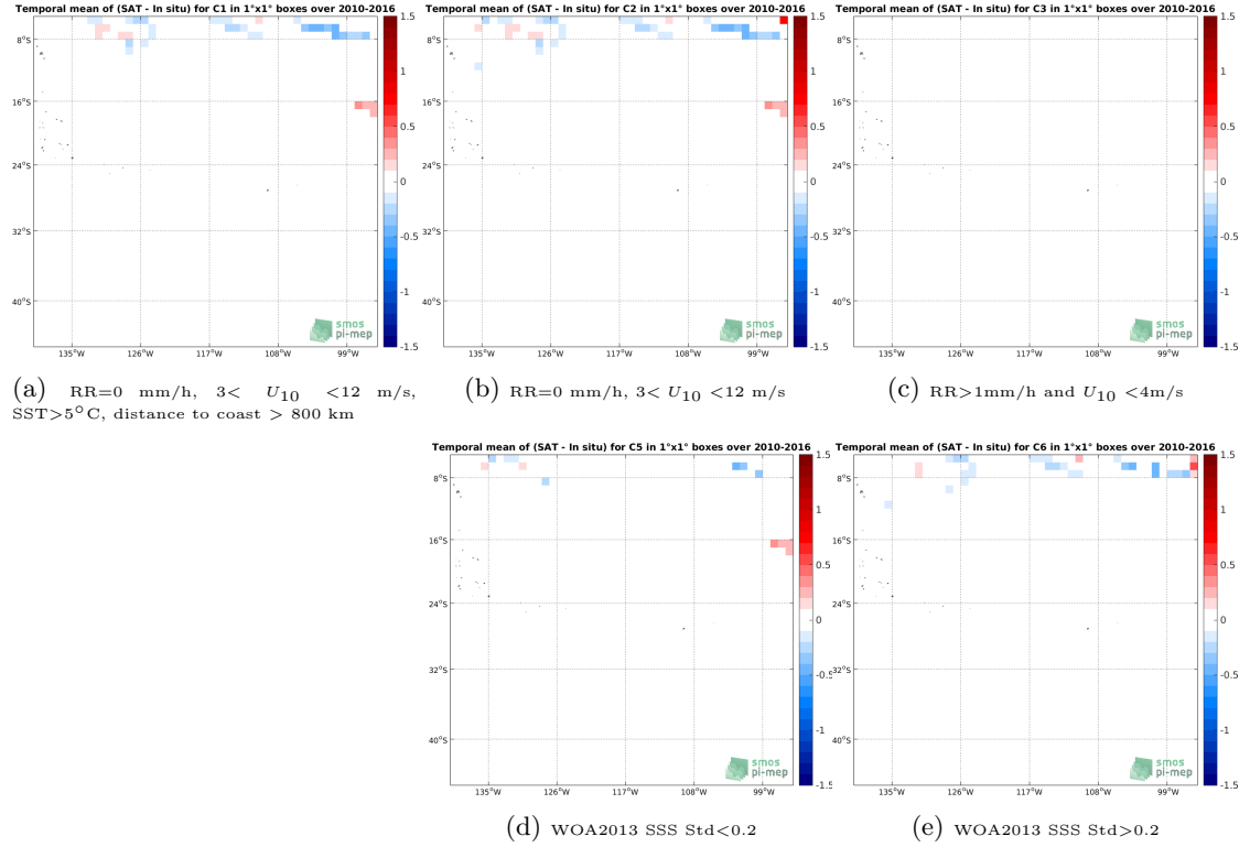
Figure 12: Temporal mean gridded over spatial boxes of size 1^\circ \times 1^\circ of \Delta SSS (SMOS-L4-CATDS-CECOS-IFREMER-V2-WEEKLY-0.5DEG - TSG-SAMOS) for 5 different subdatasets corresponding to: RR=0 mm/h, 3 < U_{10} < 12 m/s, SST > 5^\circ\text{C} , distance to coast > 800 km (a), RR=0 mm/h, 3 < U_{10} < 12 m/s (b), RR > 1 mm/h and U_{10} < 4 m/s (c), WOA2013 SSS Std < 0.2 (d), WOA2013 SSS Std > 0.2 (e).
