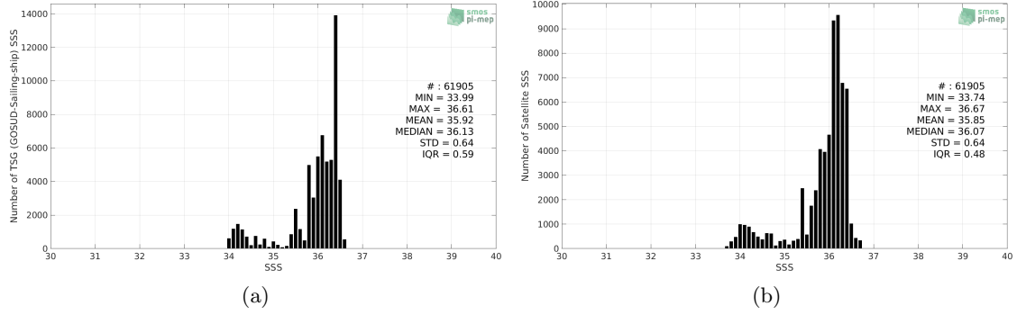
Figure 2: Histograms of SSS from TSG (GOSUD-Sailing-ship) (a) and SMOS L4 v2 Weekly (CATDS-CECOS-IFREMER) (b) considering all match-up pairs per bins of 0.1 over the OTT zone Pi-MEP region and for the full satellite product period.
