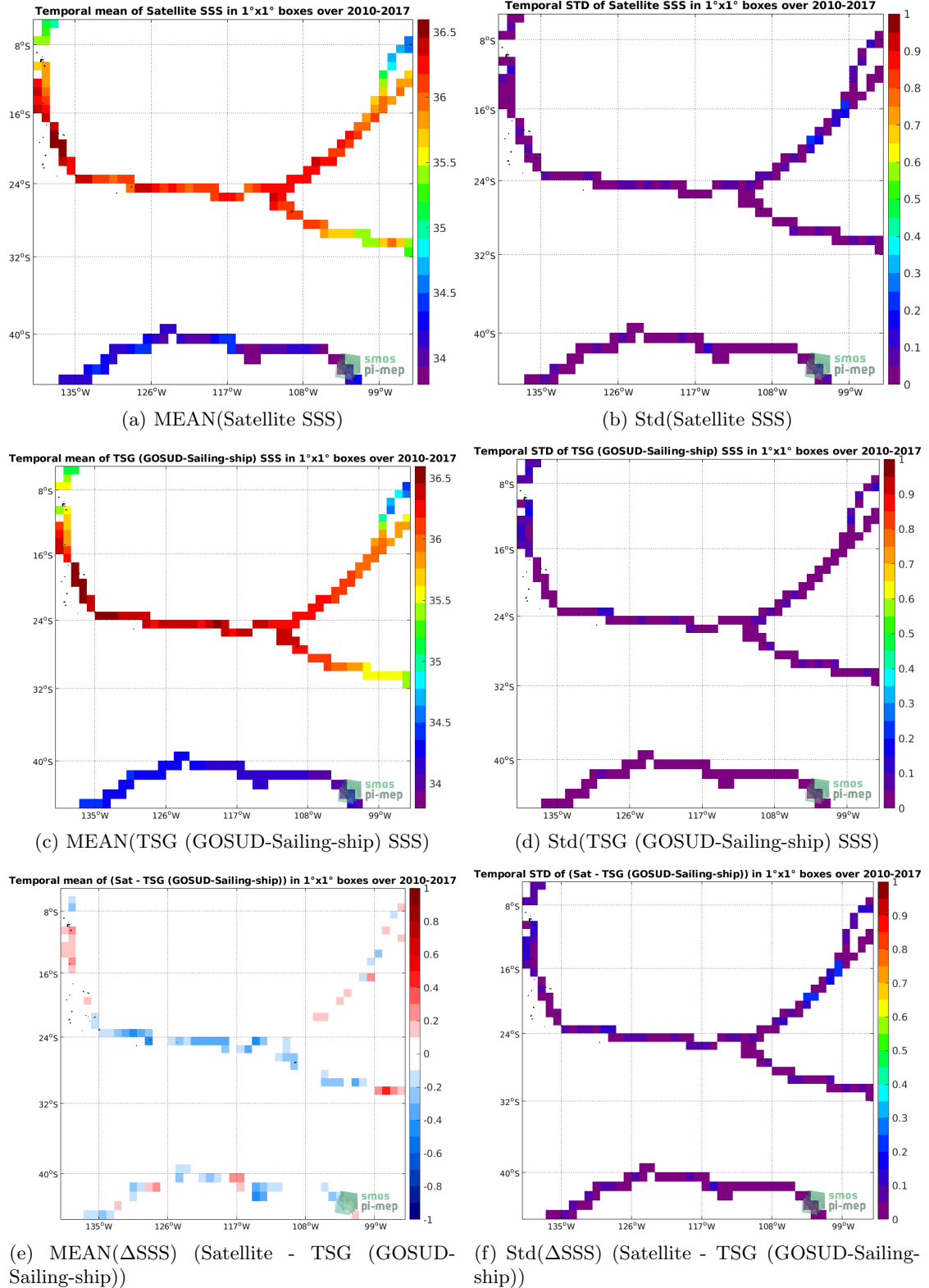
Figure 6: Temporal mean (left) and Std (right) of SSS from SMOS L4 v2 Weekly (CATDS-CECOS-IFREMER) (top), TSG (GOSUD-Sailing-ship) (middle), and of \Delta SSS (Satellite - TSG (GOSUD-Sailing-ship)). Only match-up pairs are used to generate these maps.
