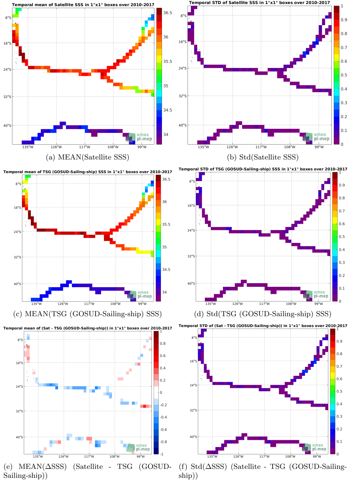
Figure 6: Temporal mean (left) and Std (right) of SSS from SMOS L4 v2 Weekly (CATDS-CECOS-IFREMER) (top), TSG (GOSUD-Sailing-ship) (middle), and of \Delta SSS (Satellite - TSG (GOSUD-Sailing-ship)). Only match-up pairs are used to generate these maps.
