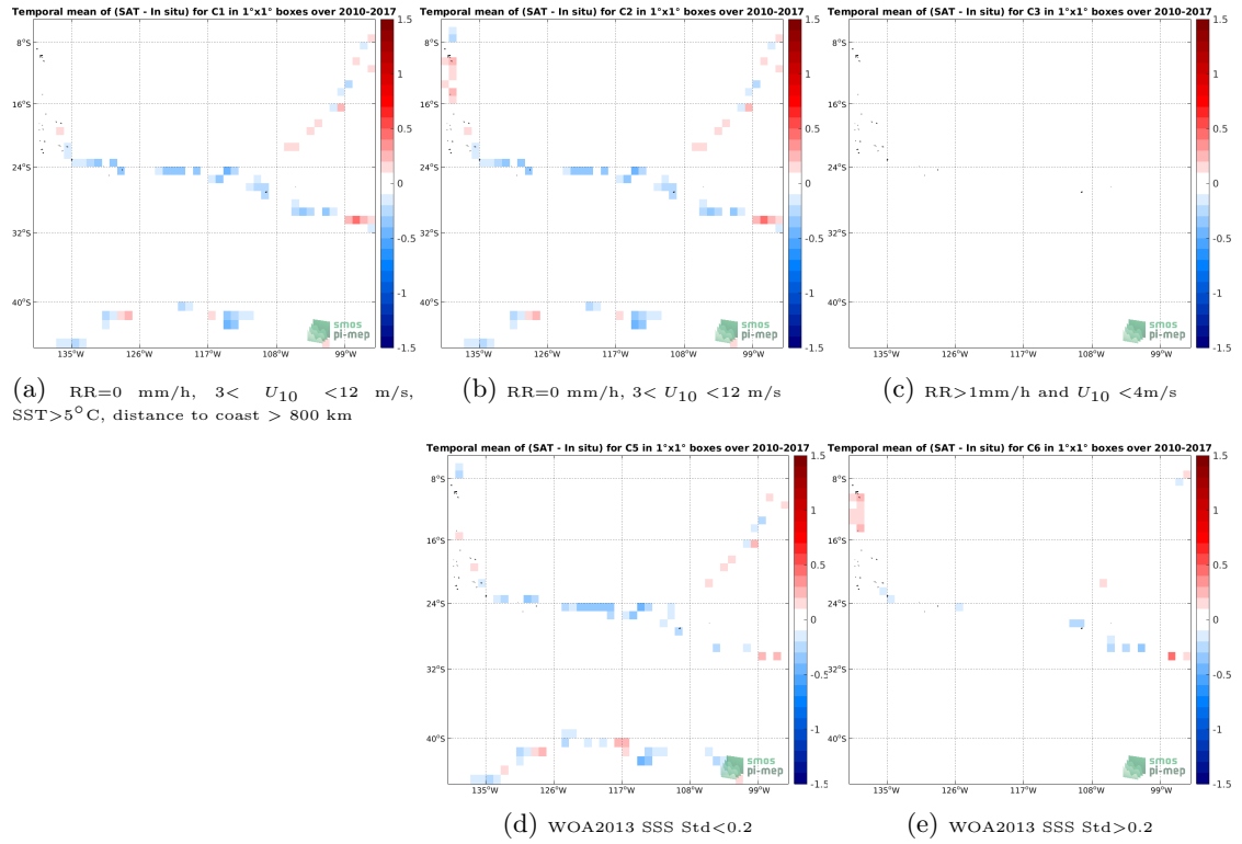
Figure 12: Temporal mean gridded over spatial boxes of size 1^\circ \times 1^\circ of \Delta SSS (SMOS L4 v2 Weekly (CATDS-CECOS-IFREMER) - TSG (GOSUD-Sailing-ship)) for 5 different subdatasets corresponding to: RR=0 mm/h, 3 < U_{10} < 12 m/s, SST > 5^\circ C , distance to coast > 800 km (a), RR=0 mm/h, 3 < U_{10} < 12 m/s (b), RR > 1 mm/h and U_{10} < 4 m/s (c), WOA2013 SSS Std < 0.2 (d), WOA2013 SSS Std > 0.2 (e).
