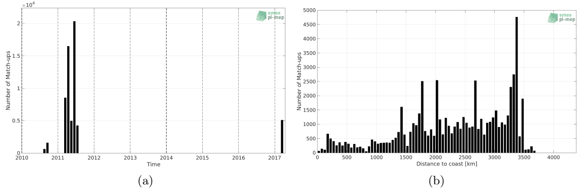
Figure 1: Number of match-ups between TSG (GOSUD-Sailing-ship) and SMOS L4 v2 Weekly (CATDS-CECOS-IFREMER) SSS as a function of time (a) and as function of the distance to coast (b) over the OTT zone Pi-MEP region and for the full satellite product period.
