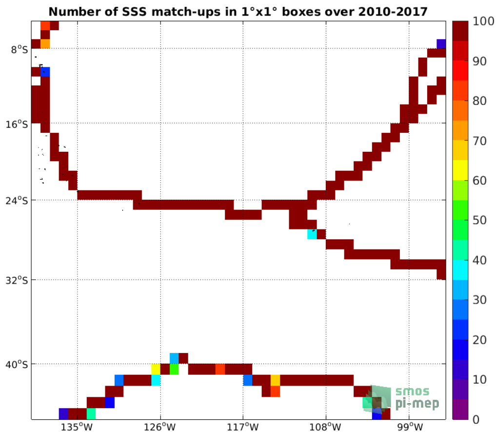
Figure 4: Number of SSS match-ups between TSG (GOSUD-Sailing-ship) SSS and the SMOS L4 v2 Weekly (CATDS-CECOS-IFREMER) SSS product for the OTT zone Pi-MEP region over 1°x1° boxes and for the full satellite product period.
