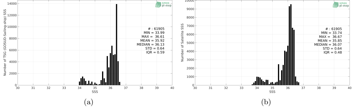
Figure 2: Histograms of SSS from TSG (GOSUD-Sailing-ship) (a) and SMOS L4 v2 Weekly (CATDS-CECOS-IFREMER) (b) considering all match-up pairs per bins of 0.1 over the OTT zone Pi-MEP region and for the full satellite product period.
