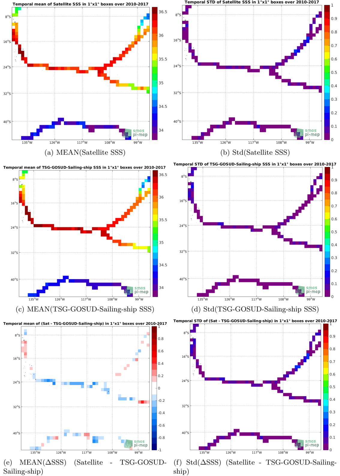
Figure 6: Temporal mean (left) and Std (right) of SSS from SMOS-L4-CATDS-CECOS-IFREMER-V2-WEEKLY-0.5DEG (top), TSG-GOSUD-Sailing-ship (middle), and of \Delta SSS (Satellite - TSG-GOSUD-Sailing-ship). Only match-up pairs are used to generate these maps.
