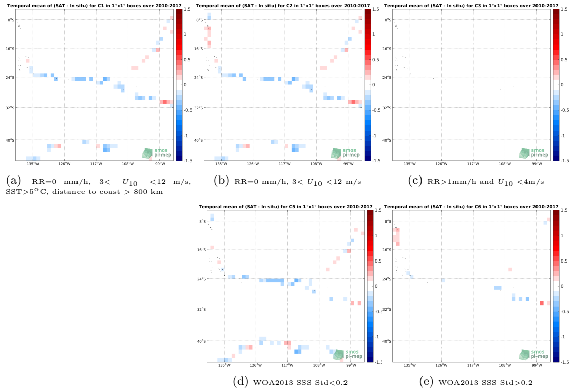
Figure 12: Temporal mean gridded over spatial boxes of size 1^\circ \times 1^\circ of \Delta SSS (SMOS-L4-CATDS-CECOS-IFREMER-V2-WEEKLY-0.5DEG - TSG-GOSUD-Sailing-ship) for 5 different subdatasets corresponding to:RR=0 mm/h, 3 < U_{10} < 12 m/s, SST >5^\circ C, distance to coast > 800 km (a), RR=0 mm/h, 3 < U_{10} < 12 m/s (b), RR >1 mm/h and U_{10} < 4 m/s (c), WOA2013 SSS Std <0.2 (d), WOA2013 SSS Std >0.2 (e).
