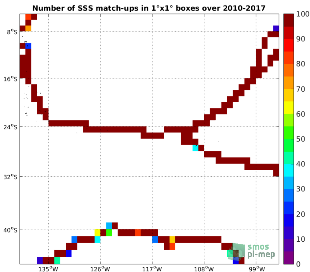
Figure 4: Number of SSS match-ups between TSG-GOSUD-Sailing-ship SSS and the SMOS-L4-CATDS-CECOS-IFREMER-V2-WEEKLY-0.5DEG SSS product for the OTT zone Pi-MEP region over 1°x1° boxes and for the full satellite product period.
