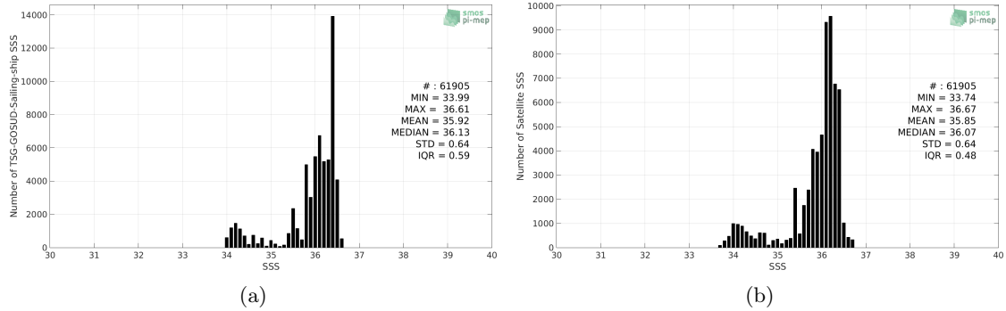
Figure 2: Histograms of SSS from TSG-GOSUD-Sailing-ship (a) and SMOS-L4-CATDS-CECOS-IFREMER-V2-WEEKLY-0.5DEG (b) considering all match-up pairs per bins of 0.1 over the OTT zone Pi-MEP region and for the full satellite product period.
