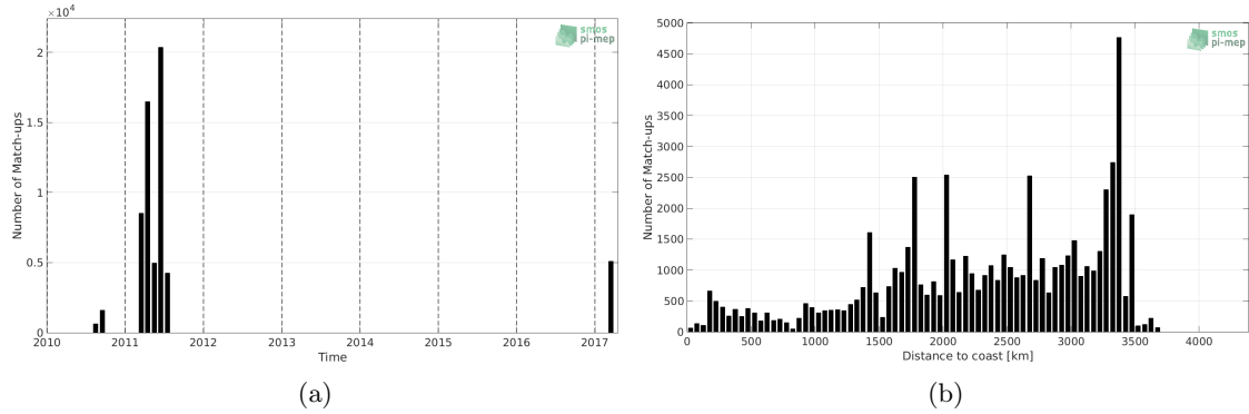
Figure 1: Number of match-ups between TSG-GOSUD-Sailing-ship and SMOS-L4-CATDS-CECOS-IFREMER-V2-WEEKLY-0.5DEG SSS as a function of time (a) and as function of the distance to coast (b) over the OTT zone Pi-MEP region and for the full satellite product period.
