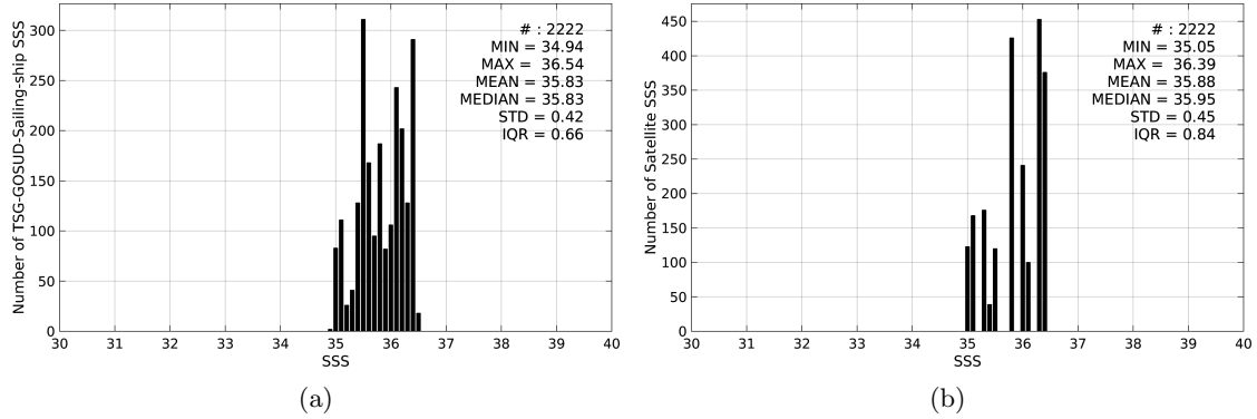
Figure 2: Histograms of SSS from TSG-GOSUD-Sailing-ship (a) and SMOS-L4-CATDS-CECOS-IFREMER-V2-WEEKLY-0.5DEG (b) considering all match-up pairs per bins of 0.1 over the OTT zone Pi-MEP region and for the full satellite product period.
