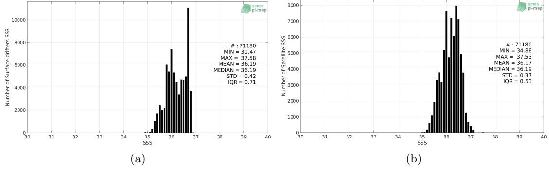
Figure 2: Histograms of SSS from Surface drifters (a) and SMOS L4 v2 Weekly (CATDS-CECOS-IFREMER) (b) considering all match-up pairs per bins of 0.1 over the OTT zone Pi-MEP region and for the full satellite product period.
