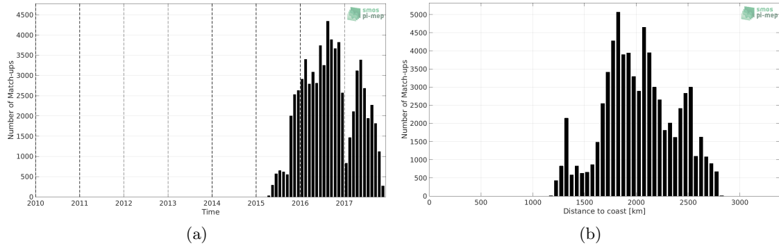
Figure 1: Number of match-ups between Surface drifters and SMOS L4 v2 Weekly (CATDS-CECOS-IFREMER) SSS as a function of time (a) and as function of the distance to coast (b) over the OTT zone Pi-MEP region and for the full satellite product period.
