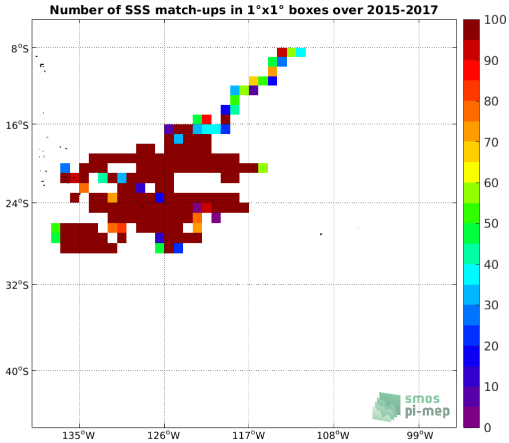
Figure 3: Number of SSS match-ups between Surface drifters SSS and the SMOS L4 v2 Weekly (CATDS-CECOS-IFREMER) SSS product for the OTT zone Pi-MEP region over 1°x1° boxes and for the full satellite product period.
