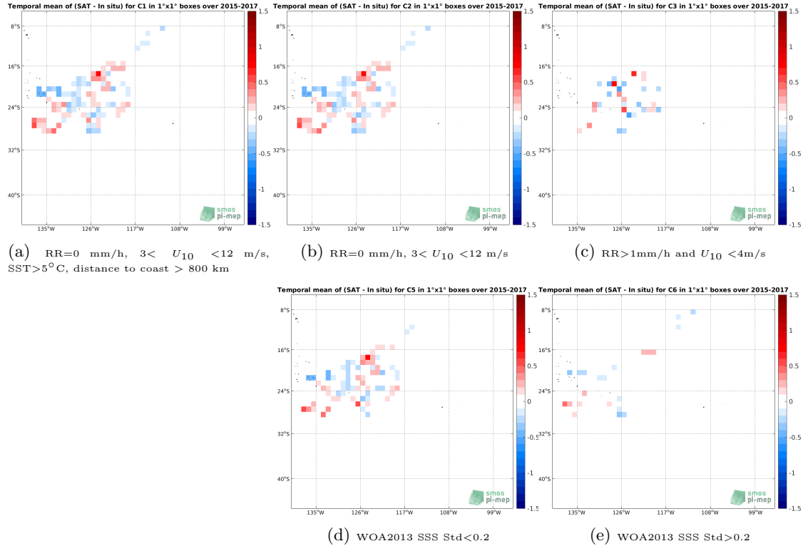
Figure 11: Temporal mean gridded over spatial boxes of size 1^{\circ}\times 1^{\circ} of \Delta\text{SSS} (SMOS L4 v2 Weekly (CATDS-CECOS-IFREMER) - Surface drifters) for 5 different subdatasets corresponding to:RR=0 mm/h, 3 < U_{10} < 12 m/s, SST >5^{\circ}\text{C} , distance to coast > 800 km (a), RR=0 mm/h, 3 < U_{10} < 12 m/s (b), RR >1 mm/h and U_{10} < 4 m/s (c), WOA2013 SSS Std <0.2 (d), WOA2013 SSS Std >0.2 (e).
