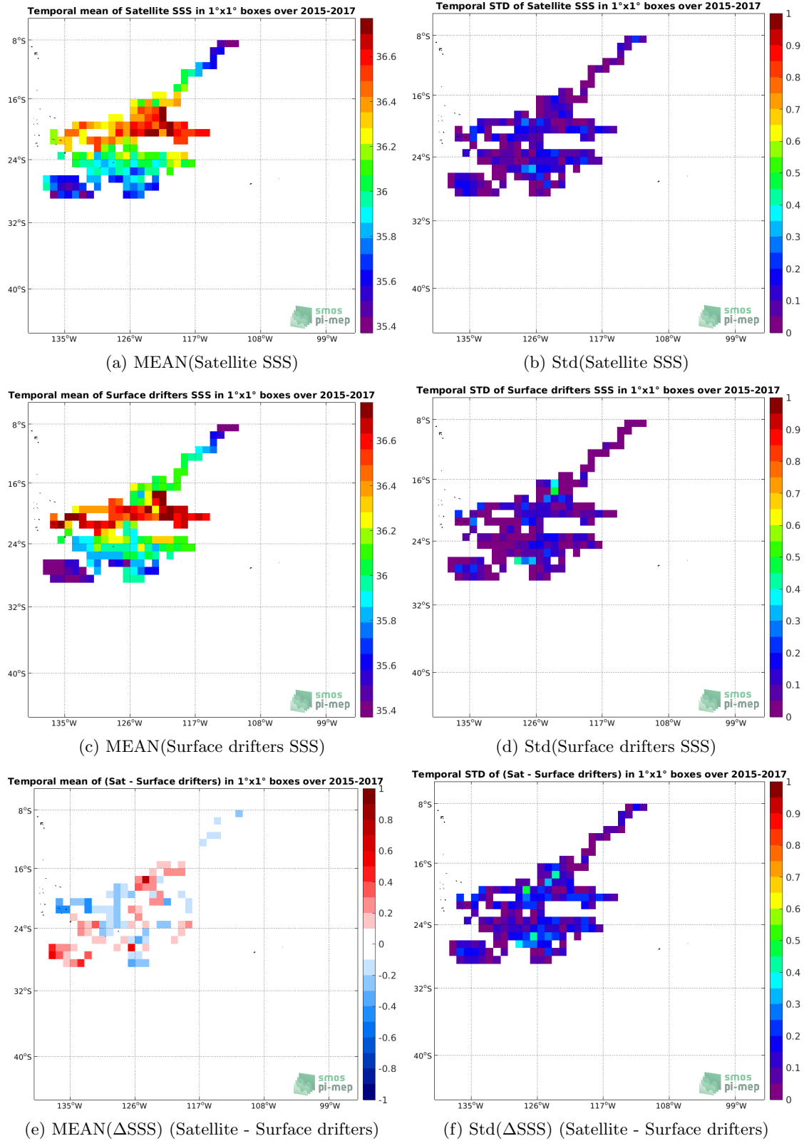
Figure 5: Temporal mean (left) and Std (right) of SSS from SMOS L4 v2 Weekly (CATDS-CECOS-IFREMER) (top), Surface drifters (middle), and of \Delta SSS (Satellite - Surface drifters). Only match-up pairs are used to generate these maps.
