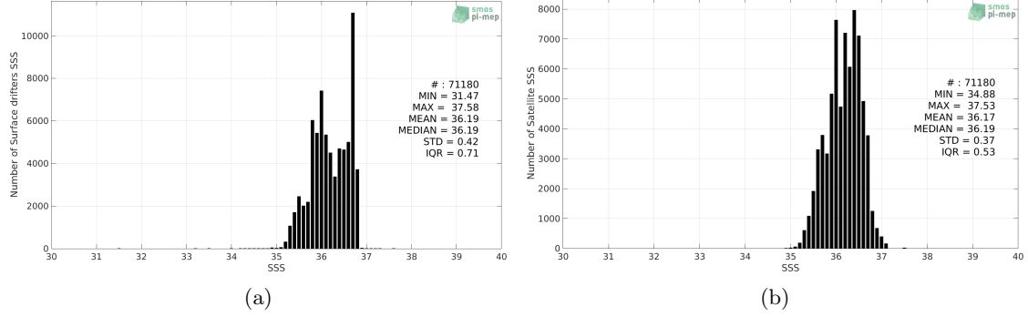
Figure 2: Histograms of SSS from Surface drifters (a) and SMOS L4 v2 Weekly (CATDS-CECOS-IFREMER) (b) considering all match-up pairs per bins of 0.1 over the OTT zone Pi-MEP region and for the full satellite product period.
