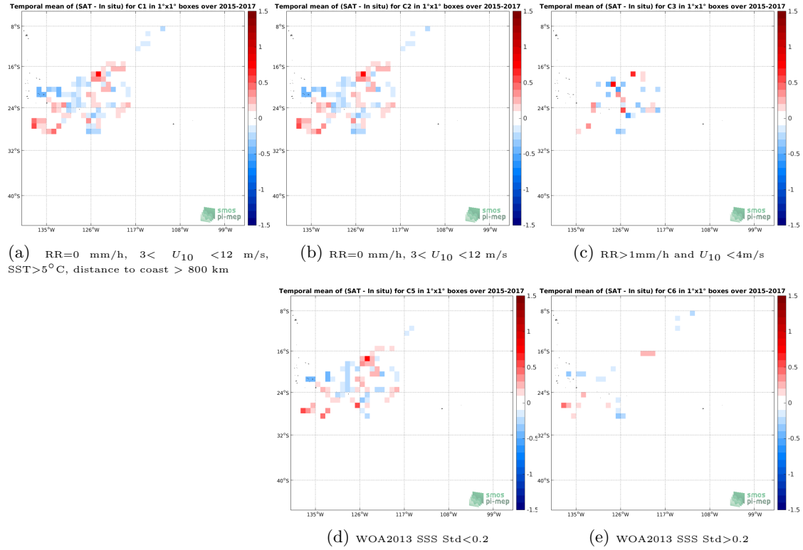
Figure 11: Temporal mean gridded over spatial boxes of size 1^{\circ}\times 1^{\circ} of \Delta\text{SSS} (SMOS-L4-CATDS-CECOS-IFREMER-V2-WEEKLY-0.5DEG - Surface drifters) for 5 different subdatasets corresponding to: \text{RR}=0 mm/h, 3 < U_{10} < 12 m/s, \text{SST} > 5^{\circ}\text{C} , distance to coast > 800 km (a), \text{RR}=0 mm/h, 3 < U_{10} < 12 m/s (b), \text{RR} > 1 mm/h and U_{10} < 4 m/s (c), WOA2013 SSS Std < 0.2 (d), WOA2013 SSS Std > 0.2 (e).
