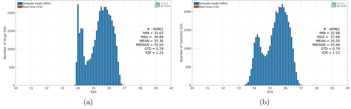
Figure 2: Histograms of SSS from Argo (a) and SMOS L4 v2 Weekly (CATDS-CECOS-IFREMER) (b) considering all match-up pairs per bins of 0.1 over the OTT zone Pi-MEP region and for the full satellite product period.
