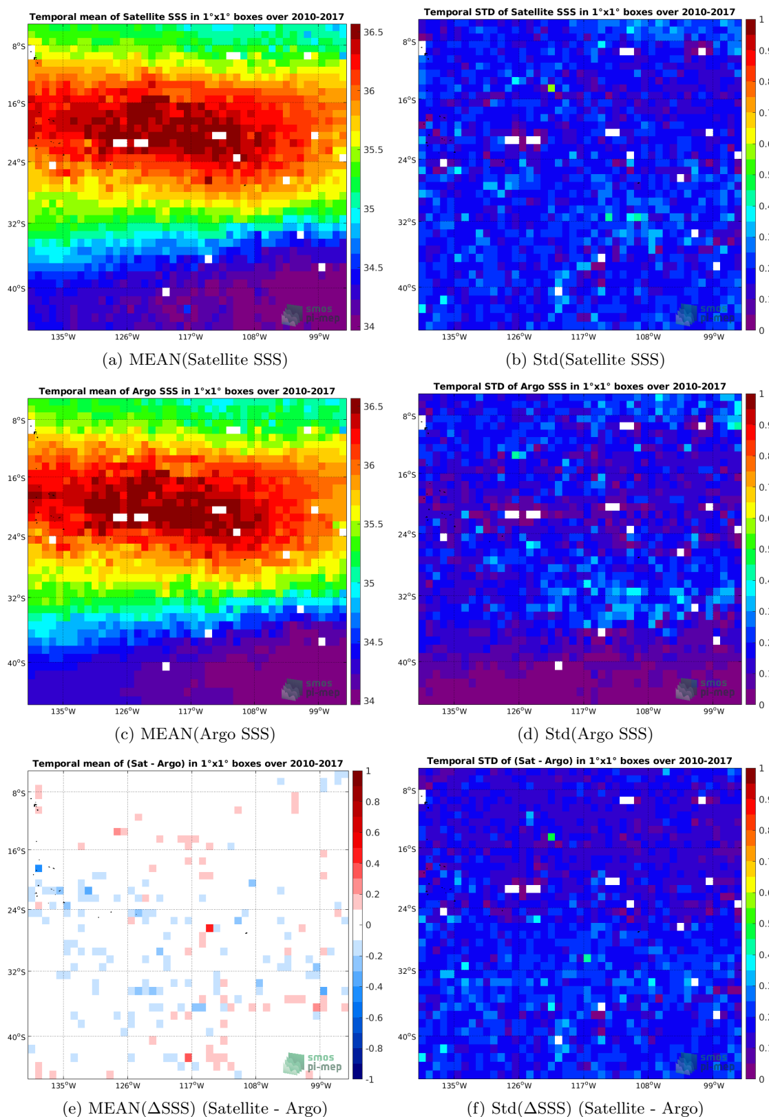
Figure 6: Temporal mean (left) and Std (right) of SSS from SMOS L4 v2 Weekly (CATDS-CECOS-IFREMER) (top), Argo (middle), and of \Delta SSS (Satellite - Argo). Only match-up pairs are used to generate these maps.
