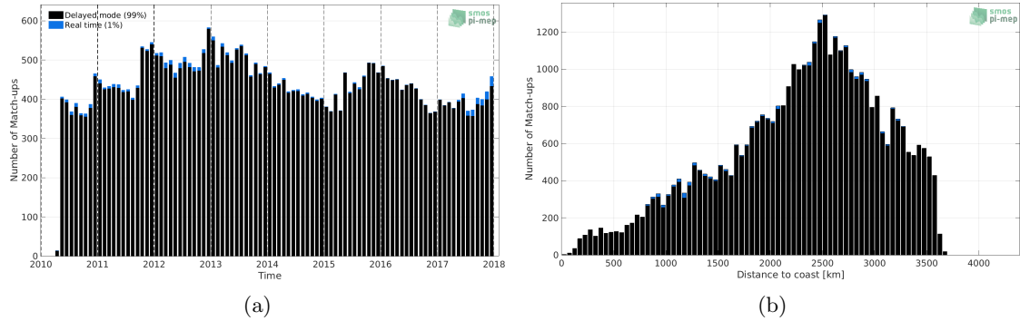
Figure 1: Number of match-ups between Argo and SMOS L4 v2 Weekly (CATDS-CECOS-IFREMER) SSS as a function of time (a) and as function of the distance to coast (b) over the OTT zone Pi-MEP region and for the full satellite product period.
