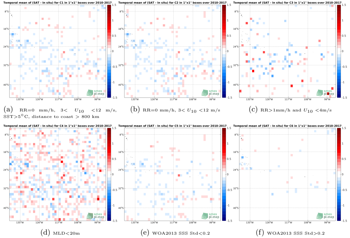
Figure 12: Temporal mean gridded over spatial boxes of size 1^\circ \times 1^\circ of \Delta SSS (SMOS L4 v2 Weekly (CATDS-CECOS-IFREMER) - Argo) for 6 different subdatasets corresponding to: RR=0 mm/h, 3 < U_{10} < 12 m/s, SST > 5^\circ C , distance to coast > 800 km (a), RR=0 mm/h, 3 < U_{10} < 12 m/s (b), RR > 1 mm/h and U_{10} < 4 m/s (c), MLD < 20 m (d), WOA2013 SSS Std < 0.2 (e), WOA2013 SSS Std > 0.2 (f).
