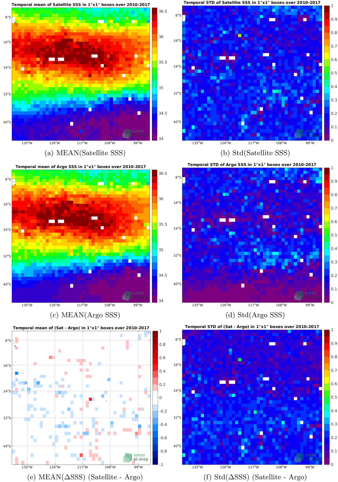
Figure 6: Temporal mean (left) and Std (right) of SSS from SMOS L4 v2 Weekly (CATDS-CECOS-IFREMER) (top), Argo (middle), and \Delta SSS (Satellite - Argo). Only match-up pairs are used to generate these maps.
