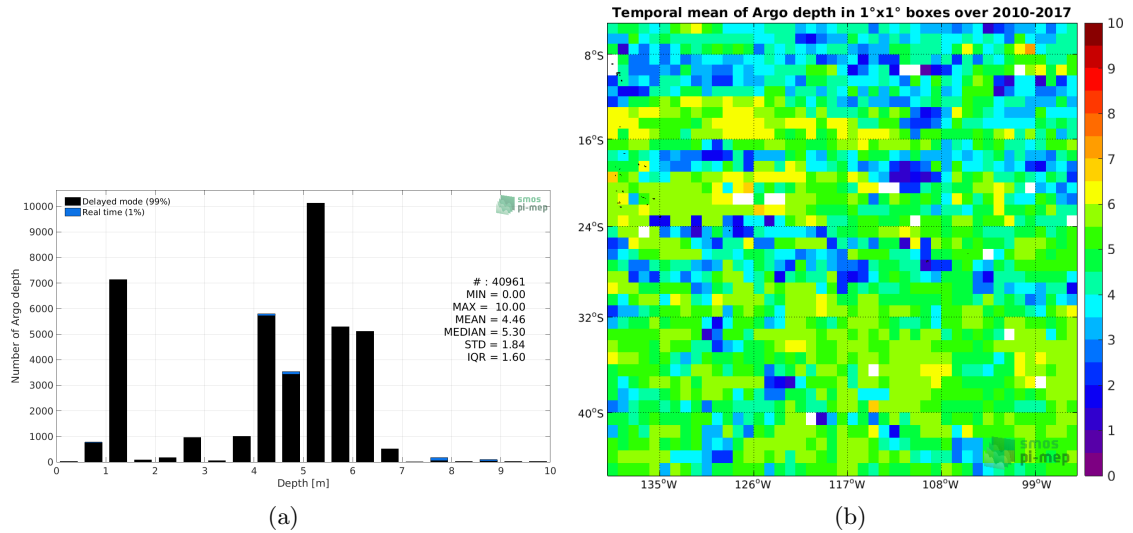
Figure 3: Histograms of the depth of the upper level SSS measurements from Argos in the Match-up DataBase for the OTT zone Pi-MEP region (a) and temporal mean spatial distribution of pressure of the in situ SSS data over 1°x1° boxes and for the full satellite product period (b).
