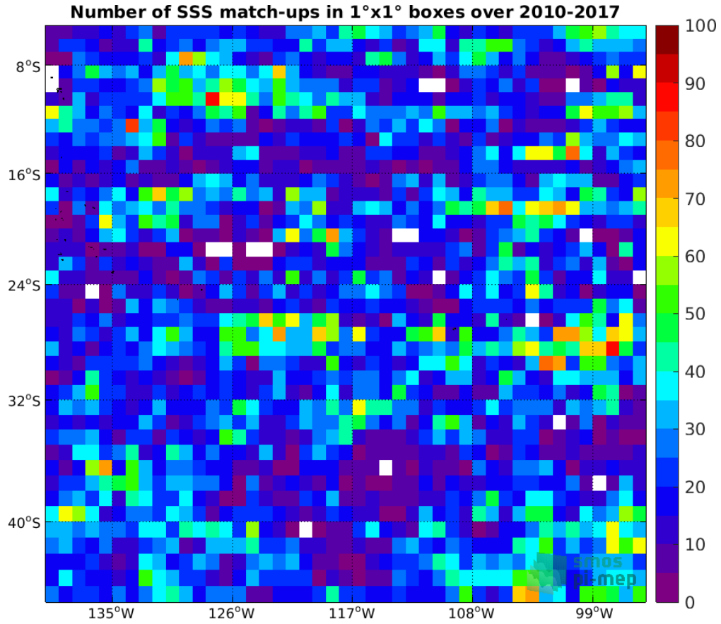
Figure 4: Number of SSS match-ups between Argo SSS and the SMOS L4 v2 Weekly (CATDS-CECOS-IFREMER) SSS product for the OTT zone Pi-MEP region over 1°x1° boxes and for the full satellite product period.
