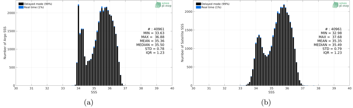
Figure 2: Histograms of SSS from Argos (a) and SMOS L4 v2 Weekly (CATDS-CECOS-IFREMER) (b) considering all match-up pairs per bins of 0.1 over the OTT zone Pi-MEP region and for the full satellite product period.
