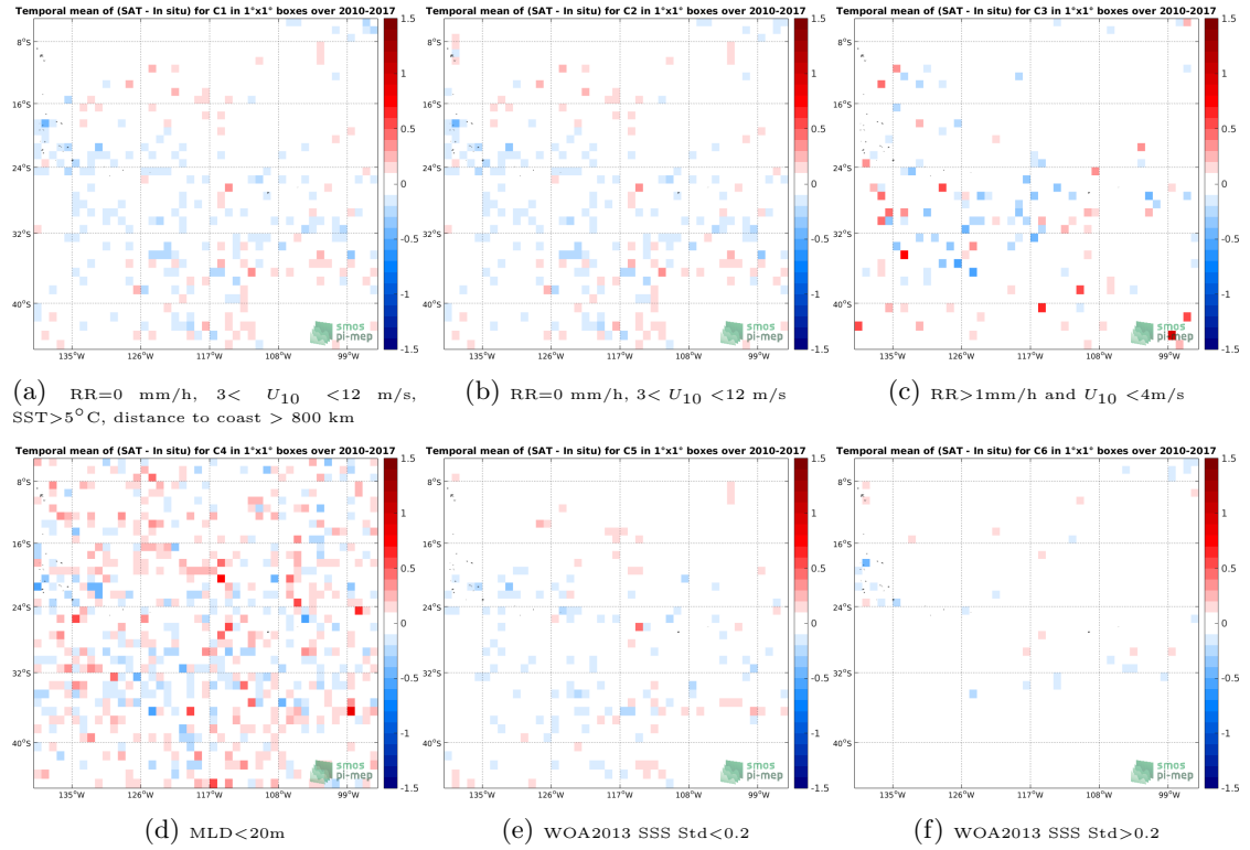
Figure 12: Temporal mean gridded over spatial boxes of size 1^\circ \times 1^\circ of \Delta SSS (SMOS-L4-CATDS-CECOS-IFREMER-V2-WEEKLY-0.5DEG - Argo) for 6 different subdatasets corresponding to: RR=0 mm/h, 3 < U_{10} < 12 m/s, SST >5^\circ C, distance to coast > 800 km (a), RR=0 mm/h, 3 < U_{10} < 12 m/s (b), RR >1 mm/h and U_{10} < 4 m/s (c),MLD <20 m (d),WOA2013 SSS Std <0.2 (e),WOA2013 SSS Std >0.2 (f).
