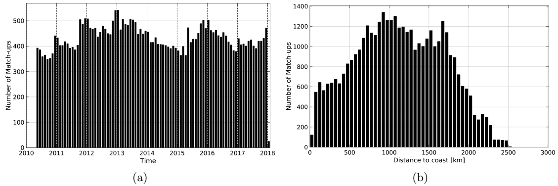
Figure 1: Number of match-ups between Argo and SMOS-L4-CATDS-CECOS-IFREMER-V2-WEEKLY-0.5DEG SSS as a function of time (a) and as function of the distance to coast (b) over the OTT zone Pi-MEP region and for the full satellite product period.
