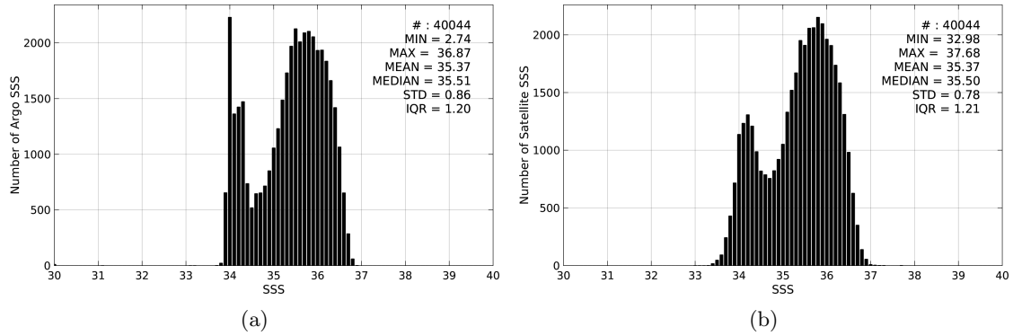
Figure 2: Histograms of SSS from Argo (a) and SMOS-L4-CATDS-CECOS-IFREMER-V2-WEEKLY-0.5DEG (b) considering all match-up pairs per bins of 0.1 over the OTT zone Pi-MEP region and for the full satellite product period.
