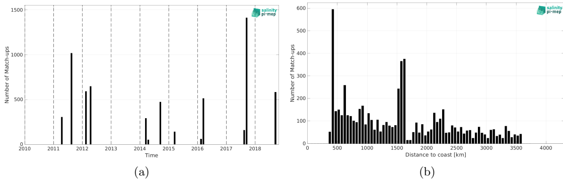
Figure 2: Number of match-ups between TSG (SAMOS) and SMOS SSS L4 v2 - Daily (BEC) SSS as a function of time (a) and as function of the distance to coast (b) over the OTT zone Pi-MEP region and for the full satellite product period.
