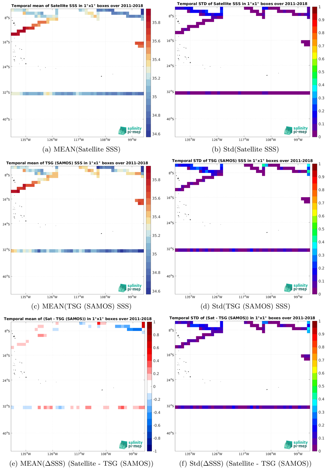
Figure 7: Temporal mean (left) and Std (right) of SSS from SMOS SSS L4 v2 - Daily (BEC) (top), TSG (SAMOS) (middle), and of \Delta SSS (Satellite - TSG (SAMOS)). Only match-up pairs are used to generate these maps.
