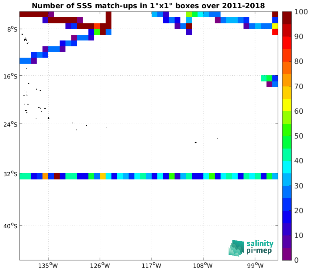
Figure 5: Number of SSS match-ups between TSG (SAMOS) SSS and the SMOS SSS L4 v2 - Daily (BEC) SSS product for the OTT zone Pi-MEP region over 1^\circ \times 1^\circ boxes and for the full satellite product period.
