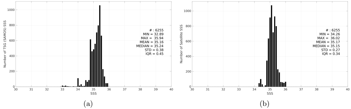
Figure 3: Histograms of SSS from TSG (SAMOS) (a) and SMOS SSS L4 v2 - Daily (BEC) (b) considering all match-up pairs per bins of 0.1 over the OTT zone Pi-MEP region and for the full satellite product period.
