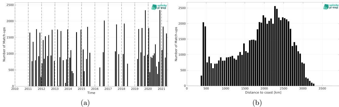
Figure 2: Number of match-ups between TSG (LEGOS-DM) and SMOS SSS L4 v2 - Daily (BEC) SSS as a function of time (a) and as function of the distance to coast (b) over the OTT zone Pi-MEP region and for the full satellite product period.
