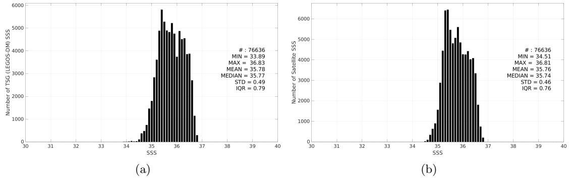
Figure 3: Histograms of SSS from TSG (LEGOS-DM) (a) and SMOS SSS L4 v2 - Daily (BEC) (b) considering all match-up pairs per bins of 0.1 over the OTT zone Pi-MEP region and for the full satellite product period.
