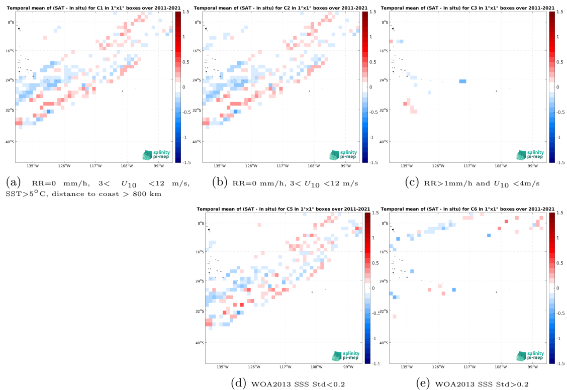
Figure 14: Temporal mean gridded over spatial boxes of size 1^\circ \times 1^\circ of \Delta SSS (SMOS SSS L4 v2 - Daily (BEC) - TSG (LEGOS-DM)) for 5 different subdatasets corresponding to:RR=0 mm/h, 3 < U_{10} < 12 m/s, SST > 5^\circ\text{C} , distance to coast > 800 km (a), RR=0 mm/h, 3 < U_{10} < 12 m/s (b), RR > 1 mm/h and U_{10} < 4 m/s (c), WOA2013 SSS Std < 0.2 (d), WOA2013 SSS Std > 0.2 (e).
