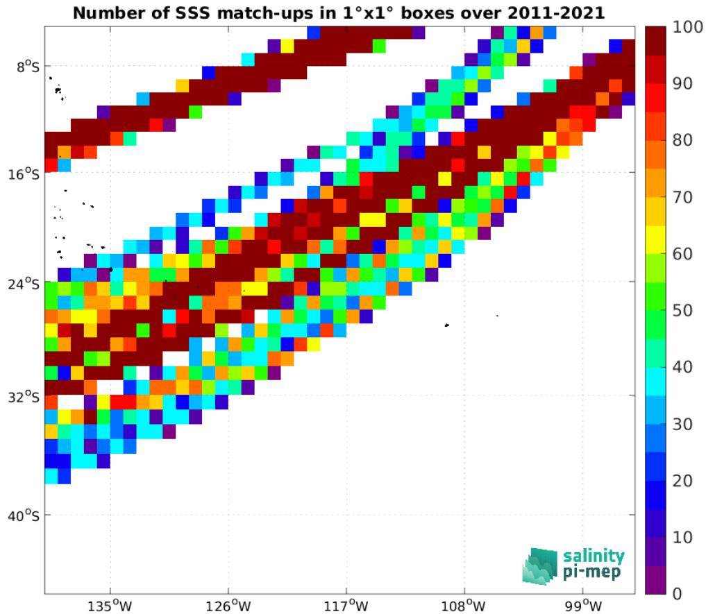
Figure 5: Number of SSS match-ups between TSG (LEGOS-DM) SSS and the SMOS SSS L4 v2 - Daily (BEC) SSS product for the OTT zone Pi-MEP region over 1^\circ \times 1^\circ boxes and for the full satellite product period.
