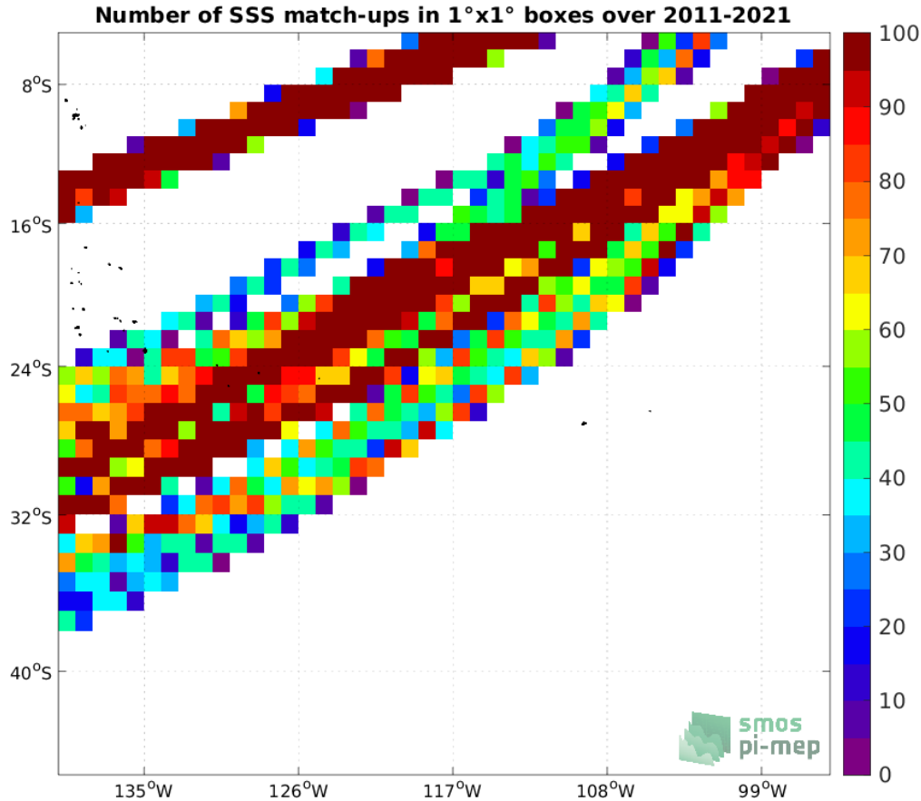
Figure 4: Number of SSS match-ups between TSG (LEGOS-DM) SSS and the SMOS SSS L4 v2 - Daily (BEC) SSS product for the OTT zone Pi-MEP region over 1^\circ \times 1^\circ boxes and for the full satellite product period.
