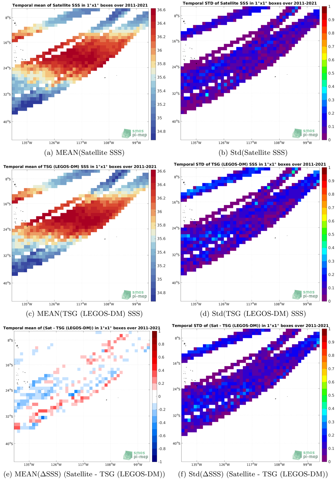
Figure 6: Temporal mean (left) and Std (right) of SSS from SMOS SSS L4 v2 - Daily (BEC) (top), TSG (LEGOS-DM) (middle), and of \Delta SSS (Satellite - TSG (LEGOS-DM)). Only match-up pairs are used to generate these maps.
