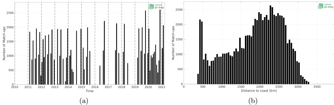
Figure 1: Number of match-ups between TSG (LEGOS-DM) and SMOS SSS L4 v2 - Daily (BEC) SSS as a function of time (a) and as function of the distance to coast (b) over the OTT zone Pi-MEP region and for the full satellite product period.
