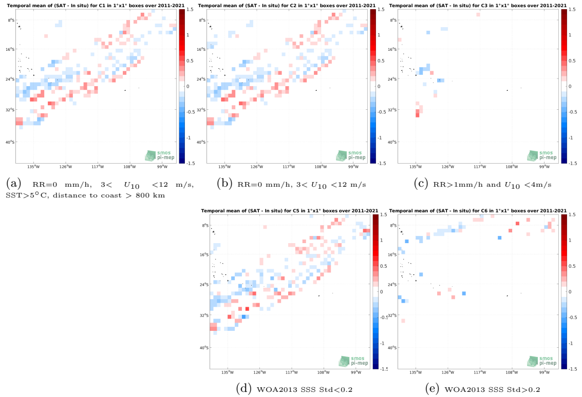
Figure 12: Temporal mean gridded over spatial boxes of size 1^\circ \times 1^\circ of \Delta SSS (SMOS SSS L4 v2 - Daily (BEC) - TSG (LEGOS-DM)) for 5 different subdatasets corresponding to:RR=0 mm/h, 3 < U_{10} < 12 m/s, SST > 5^\circ\text{C} , distance to coast > 800 km (a), RR=0 mm/h, 3 < U_{10} < 12 m/s (b), RR > 1 mm/h and U_{10} < 4 m/s (c), WOA2013 SSS Std < 0.2 (d), WOA2013 SSS Std > 0.2 (e).
