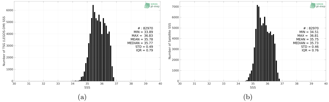
Figure 2: Histograms of SSS from TSG (LEGOS-DM) (a) and SMOS SSS L4 v2 - Daily (BEC) (b) considering all match-up pairs per bins of 0.1 over the OTT zone Pi-MEP region and for the full satellite product period.
