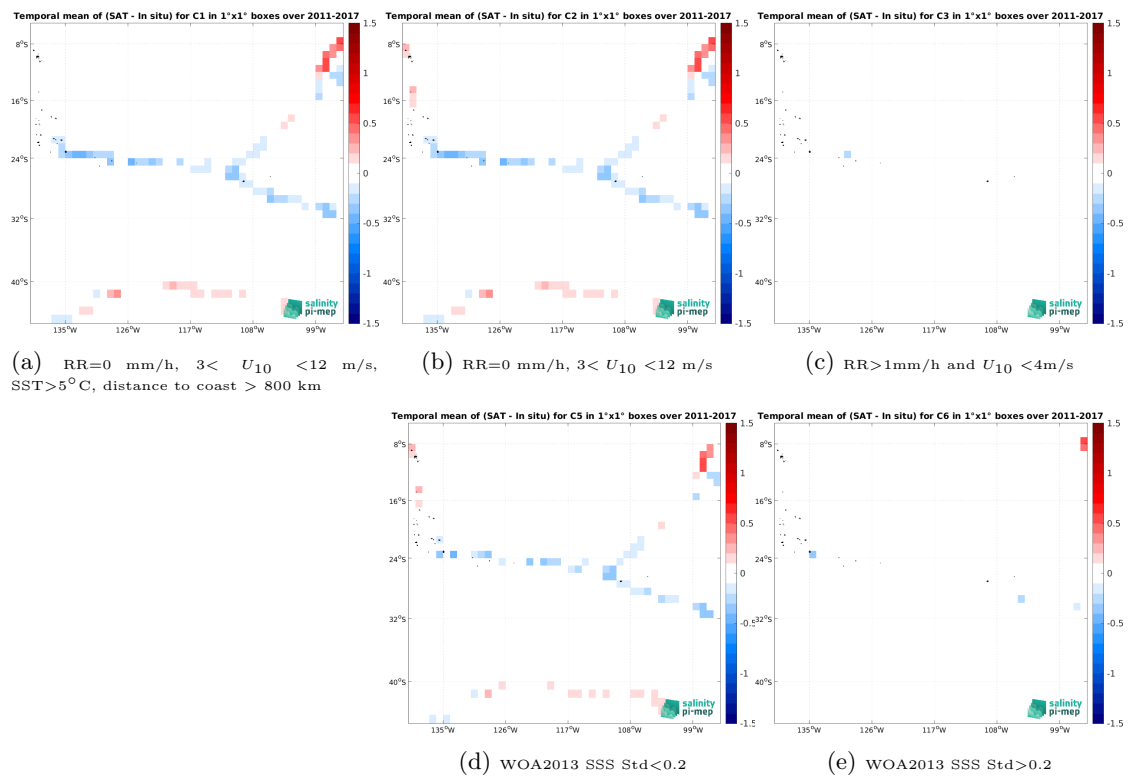
Figure 14: Temporal mean gridded over spatial boxes of size 1^\circ \times 1^\circ of \Delta SSS (SMOS SSS L4 v2 - Daily (BEC) - TSG (GOSUD-Sailing-ship)) for 5 different subdatasets corresponding to:RR=0 mm/h, 3 < U_{10} < 12 m/s, SST >5^\circ\text{C} , distance to coast > 800 km (a), RR=0 mm/h, 3 < U_{10} < 12 m/s (b), RR >1 mm/h and U_{10} < 4 m/s (c), WOA2013 SSS Std <0.2 (d), WOA2013 SSS Std >0.2 (e).
