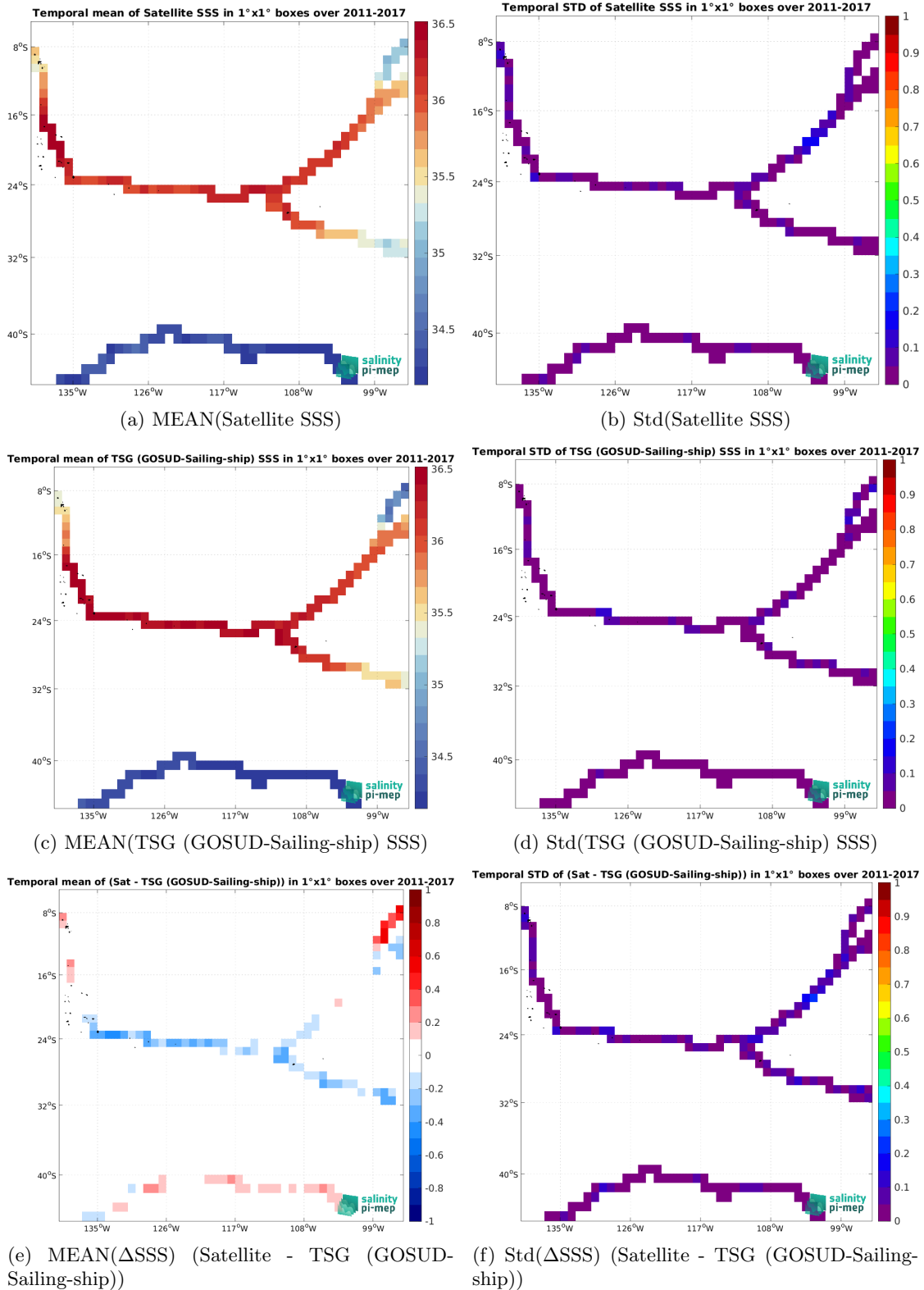
Figure 7: Temporal mean (left) and Std (right) of SSS from SMOS SSS L4 v2 - Daily (BEC) (top), TSG (GOSUD-Sailing-ship) (middle), and of \Delta SSS (Satellite - TSG (GOSUD-Sailing-ship)). Only match-up pairs are used to generate these maps.
