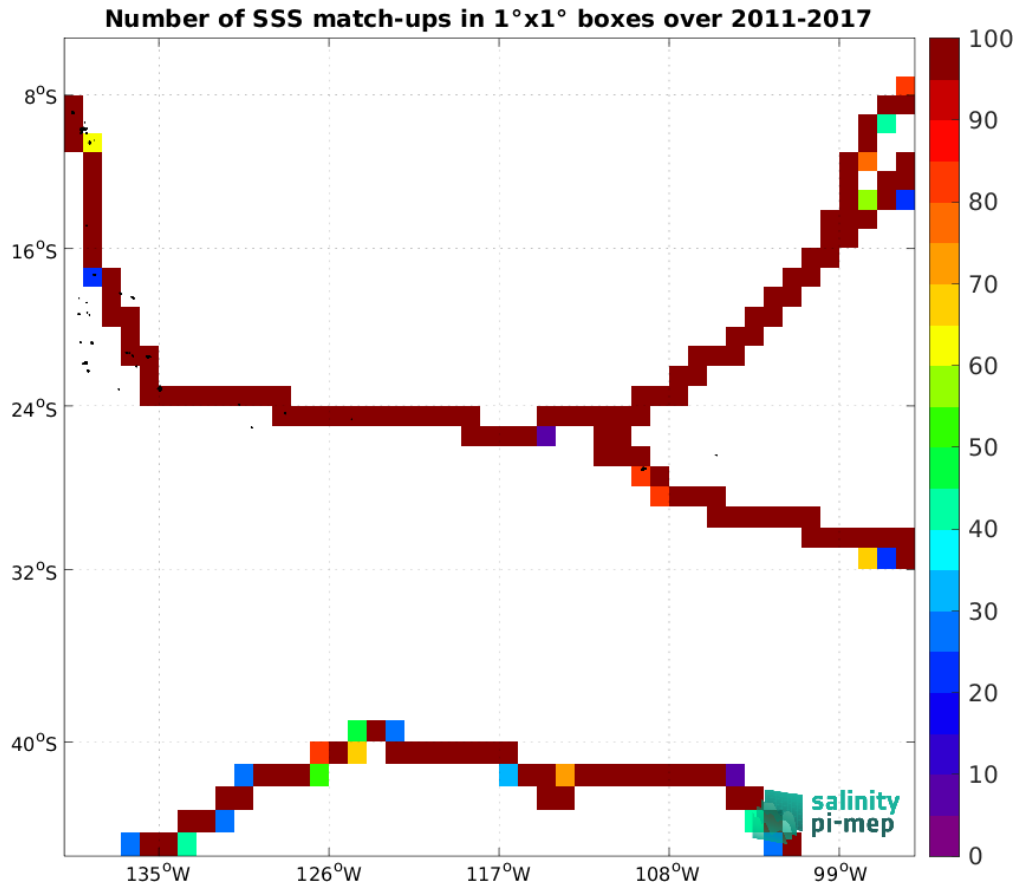
Figure 5: Number of SSS match-ups between TSG (GOSUD-Sailing-ship) SSS and the SMOS SSS L4 v2 - Daily (BEC) SSS product for the OTT zone Pi-MEP region over 1^\circ \times 1^\circ boxes and for the full satellite product period.
