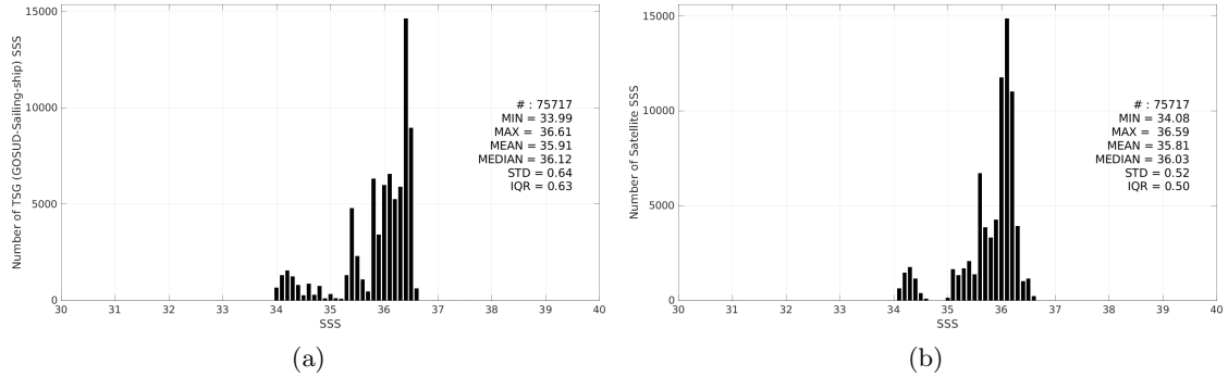
Figure 3: Histograms of SSS from TSG (GOSUD-Sailing-ship) (a) and SMOS SSS L4 v2 - Daily (BEC) (b) considering all match-up pairs per bins of 0.1 over the OTT zone Pi-MEP region and for the full satellite product period.
