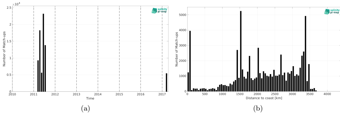
Figure 2: Number of match-ups between TSG (GOSUD-Sailing-ship) and SMOS SSS L4 v2 - Daily (BEC) SSS as a function of time (a) and as function of the distance to coast (b) over the OTT zone Pi-MEP region and for the full satellite product period.
