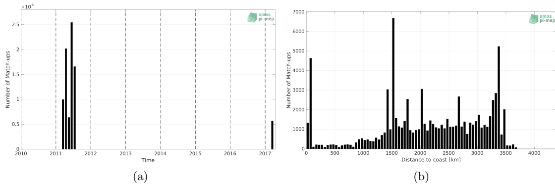
Figure 1: Number of match-ups between TSG (GOSUD-Sailing-ship) and SMOS SSS L4 v2 - Daily (BEC) SSS as a function of time (a) and as function of the distance to coast (b) over the OTT zone Pi-MEP region and for the full satellite product period.
