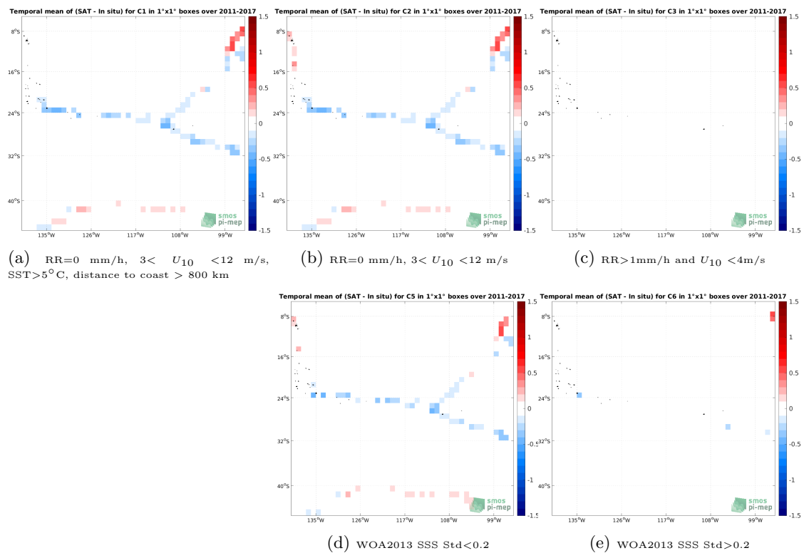
Figure 12: Temporal mean gridded over spatial boxes of size 1^\circ \times 1^\circ of \Delta SSS (SMOS SSS L4 v2 - Daily (BEC) - TSG (GOSUD-Sailing-ship)) for 5 different subdatasets corresponding to: RR=0 mm/h, 3 < U_{10} < 12 m/s, SST > 5^\circ C , distance to coast > 800 km (a), RR=0 mm/h, 3 < U_{10} < 12 m/s (b), RR > 1 mm/h and U_{10} < 4 m/s (c), WOA2013 SSS Std < 0.2 (d), WOA2013 SSS Std > 0.2 (e).
