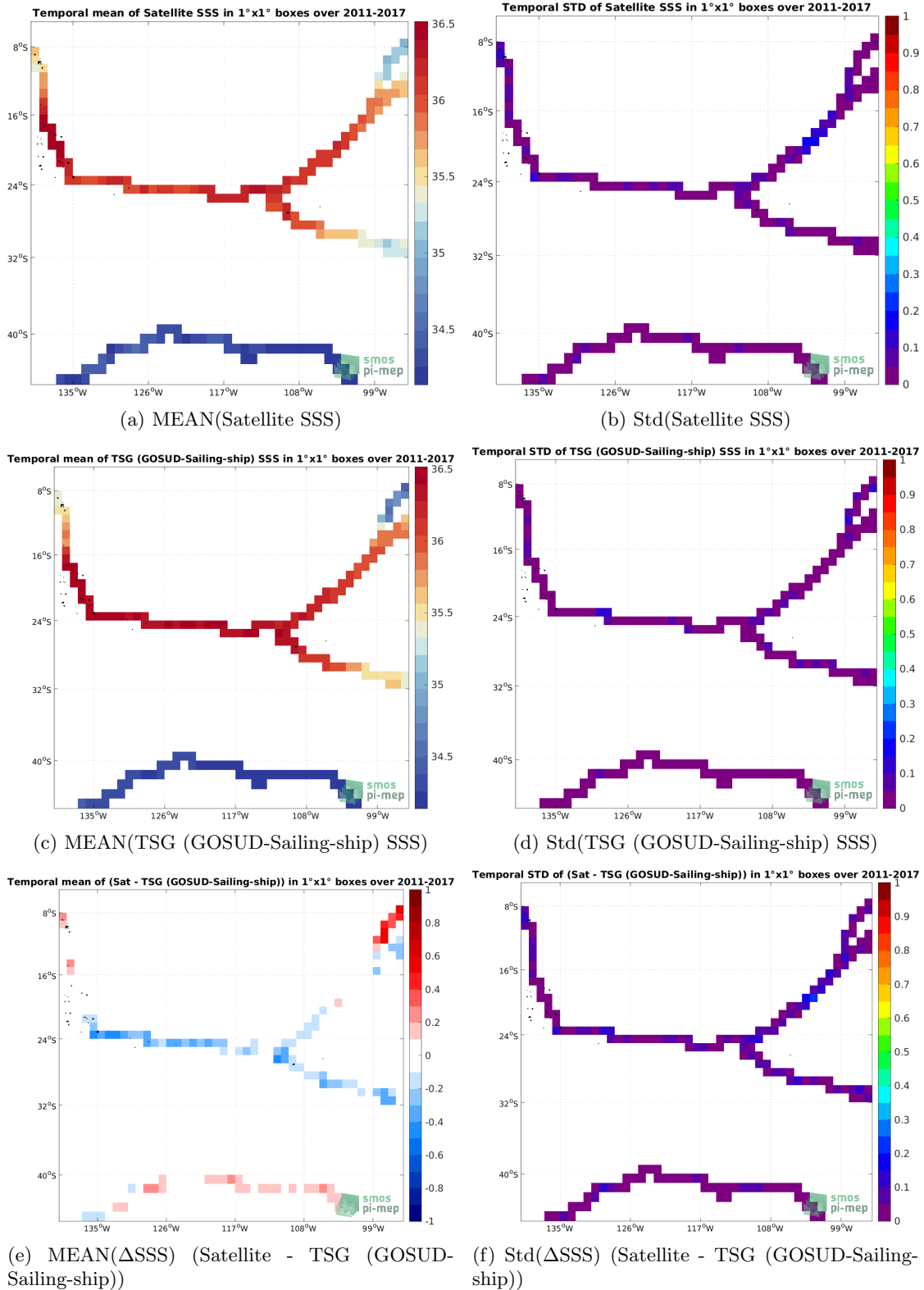
Figure 6: Temporal mean (left) and Std (right) of SSS from SMOS SSS L4 v2 - Daily (BEC) (top), TSG (GOSUD-Sailing-ship) (middle), and of \Delta SSS (Satellite - TSG (GOSUD-Sailing-ship)). Only match-up pairs are used to generate these maps.
