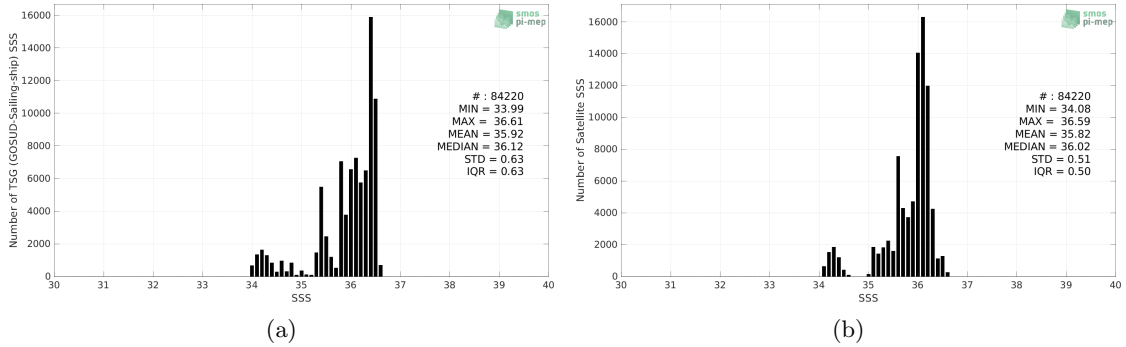
Figure 2: Histograms of SSS from TSG (GOSUD-Sailing-ship) (a) and SMOS SSS L4 v2 - Daily (BEC) (b) considering all match-up pairs per bins of 0.1 over the OTT zone Pi-MEP region and for the full satellite product period.
