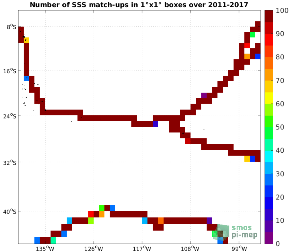
Figure 4: Number of SSS match-ups between TSG (GOSUD-Sailing-ship) SSS and the SMOS SSS L4 v2 - Daily (BEC) SSS product for the OTT zone Pi-MEP region over 1^\circ \times 1^\circ boxes and for the full satellite product period.
