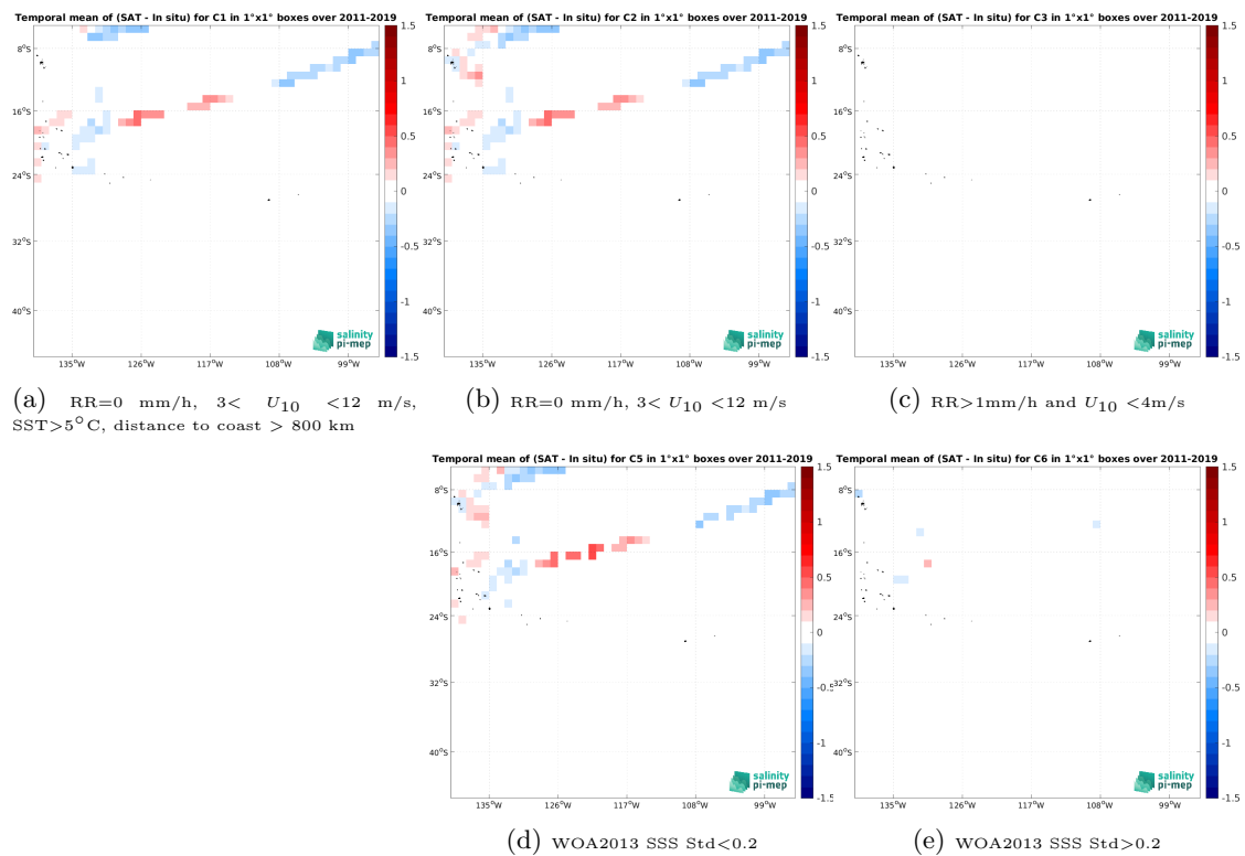
Figure 14: Temporal mean gridded over spatial boxes of size 1^\circ \times 1^\circ of \Delta SSS (SMOS SSS L4 v2 - Daily (BEC) - TSG (GOSUD-Research-vessel)) for 5 different subdatasets corresponding to:RR=0 mm/h, 3 < U_{10} < 12 m/s, SST >5^\circ\text{C} , distance to coast > 800 km (a), RR=0 mm/h, 3 < U_{10} < 12 m/s (b), RR >1 mm/h and U_{10} < 4 m/s (c), WOA2013 SSS Std <0.2 (d), WOA2013 SSS Std >0.2 (e).
