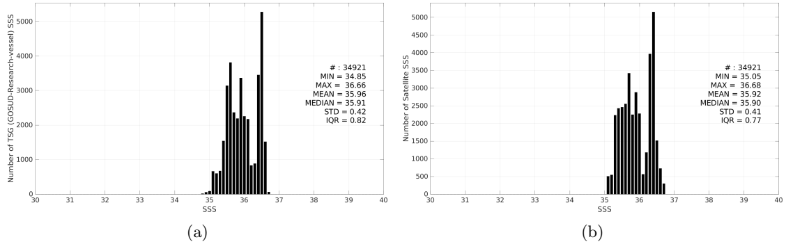
Figure 3: Histograms of SSS from TSG (GOSUD-Research-vessel) (a) and SMOS SSS L4 v2 - Daily (BEC) (b) considering all match-up pairs per bins of 0.1 over the OTT zone Pi-MEP region and for the full satellite product period.
