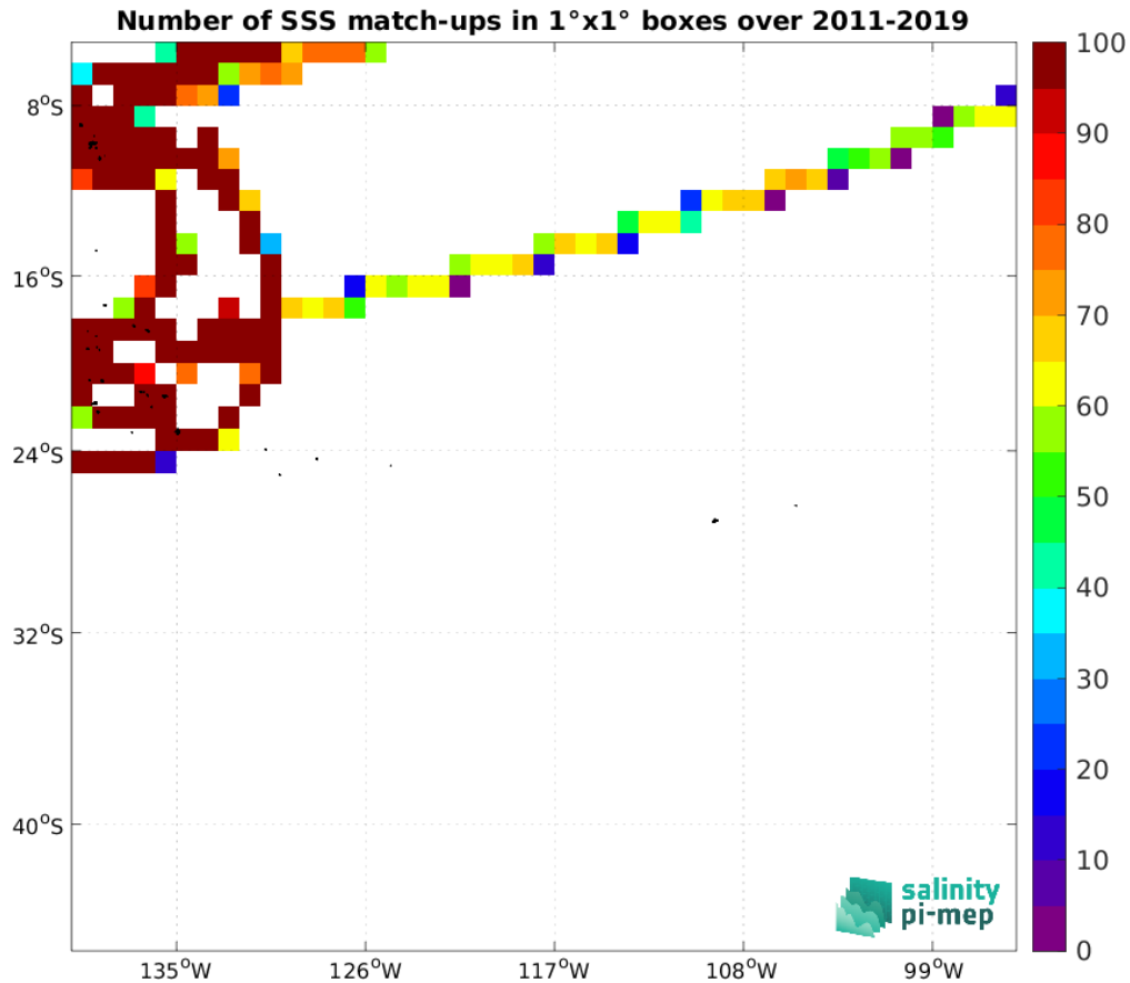
Figure 5: Number of SSS match-ups between TSG (GOSUD-Research-vessel) SSS and the SMOS SSS L4 v2 - Daily (BEC) SSS product for the OTT zone Pi-MEP region over 1^\circ \times 1^\circ boxes and for the full satellite product period.
