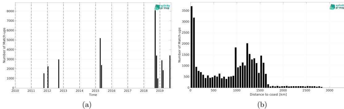
Figure 2: Number of match-ups between TSG (GOSUD-Research-vessel) and SMOS SSS L4 v2 - Daily (BEC) SSS as a function of time (a) and as function of the distance to coast (b) over the OTT zone Pi-MEP region and for the full satellite product period.
