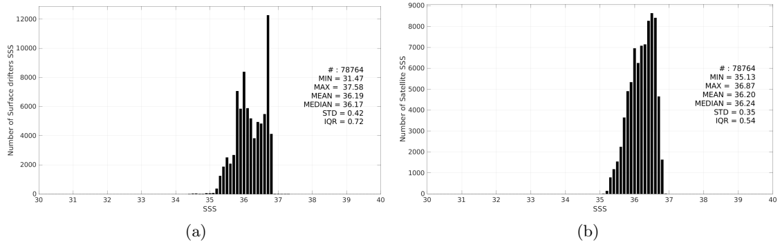
Figure 3: Histograms of SSS from Surface drifters (a) and SMOS SSS L4 v2 - Daily (BEC) (b) considering all match-up pairs per bins of 0.1 over the OTT zone Pi-MEP region and for the full satellite product period.
