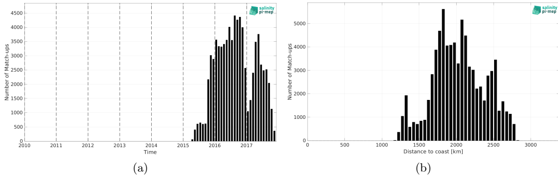
Figure 2: Number of match-ups between Surface drifters and SMOS SSS L4 v2 - Daily (BEC) SSS as a function of time (a) and as function of the distance to coast (b) over the OTT zone Pi-MEP region and for the full satellite product period.
