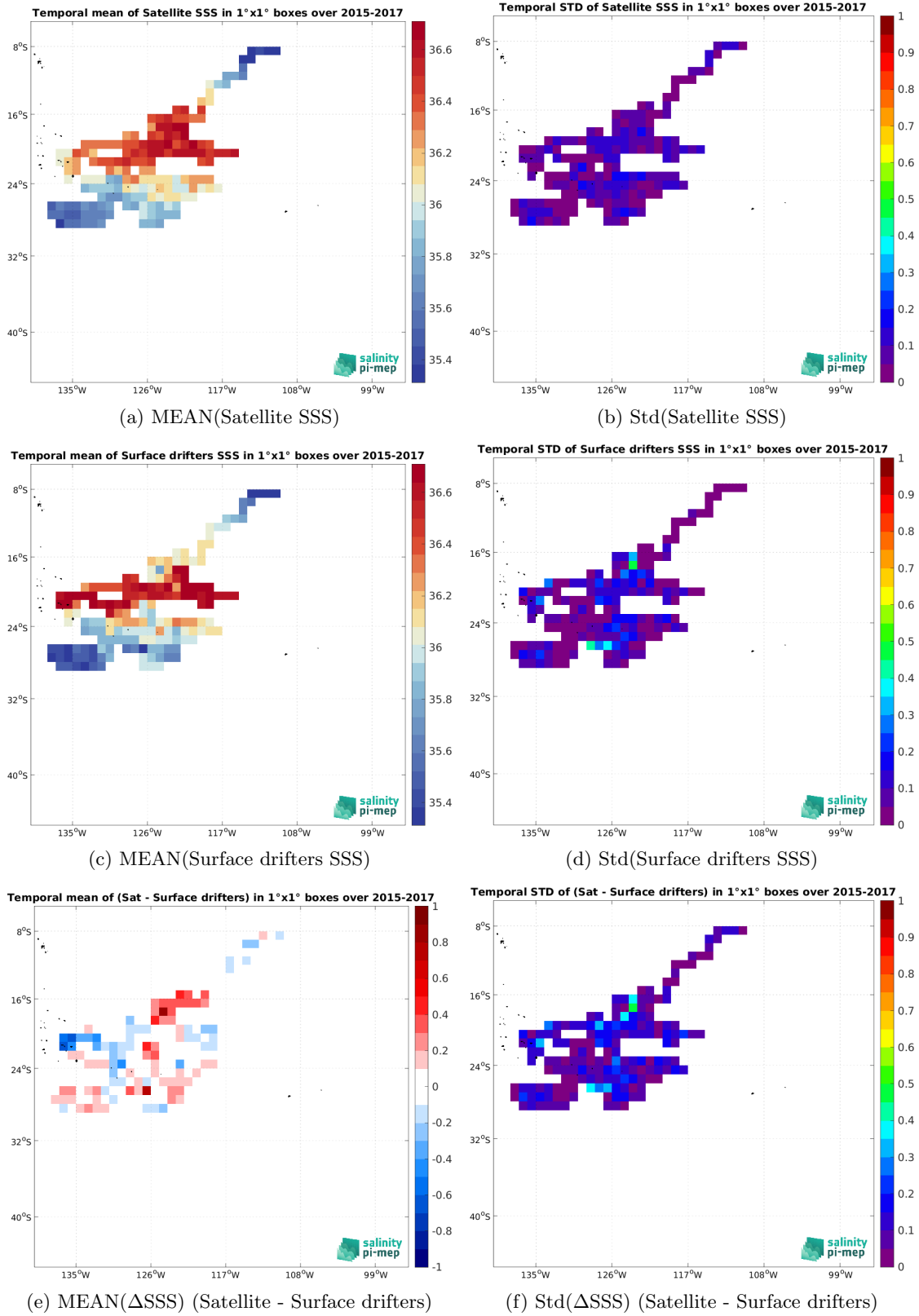
Figure 6: Temporal mean (left) and Std (right) of SSS from SMOS SSS L4 v2 - Daily (BEC) (top), Surface drifters (middle), and of \Delta SSS (Satellite - Surface drifters). Only match-up pairs are used to generate these maps.
