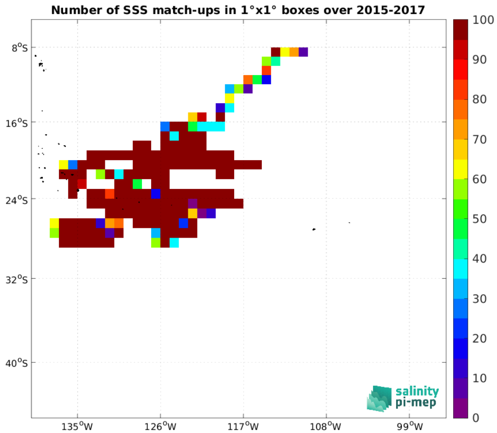
Figure 4: Number of SSS match-ups between Surface drifters SSS and the SMOS SSS L4 v2 - Daily (BEC) SSS product for the OTT zone Pi-MEP region over 1^\circ \times 1^\circ boxes and for the full satellite product period.
