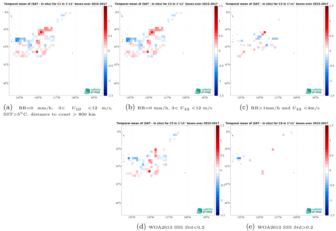
Figure 13: Temporal mean gridded over spatial boxes of size 1^\circ \times 1^\circ of \Delta SSS (SMOS SSS L4 v2 - Daily (BEC) - Surface drifters) for 5 different subdatasets corresponding to:RR=0 mm/h, 3 < U_{10} < 12 m/s, SST > 5^\circ\text{C} , distance to coast > 800 km (a), RR=0 mm/h, 3 < U_{10} < 12 m/s (b), RR > 1 mm/h and U_{10} < 4 m/s (c), WOA2013 SSS Std < 0.2 (d), WOA2013 SSS Std > 0.2 (e).
