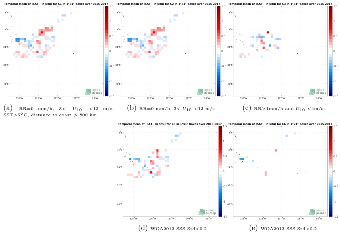
Figure 11: Temporal mean gridded over spatial boxes of size 1^\circ \times 1^\circ of \Delta SSS (SMOS SSS L4 v2 - Daily (BEC) - Surface drifters) for 5 different subdatasets corresponding to:RR=0 mm/h, 3 < U_{10} < 12 m/s, SST >5^\circ C, distance to coast > 800 km (a), RR=0 mm/h, 3 < U_{10} < 12 m/s (b), RR >1 mm/h and U_{10} < 4 m/s (c), WOA2013 SSS Std <0.2 (d), WOA2013 SSS Std >0.2 (e).
