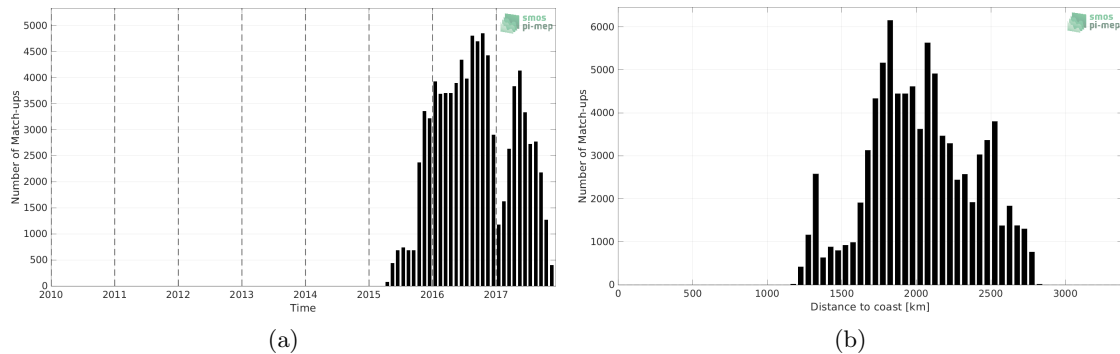
Figure 1: Number of match-ups between Surface drifters and SMOS SSS L4 v2 - Daily (BEC) SSS as a function of time (a) and as function of the distance to coast (b) over the OTT zone Pi-MEP region and for the full satellite product period.
