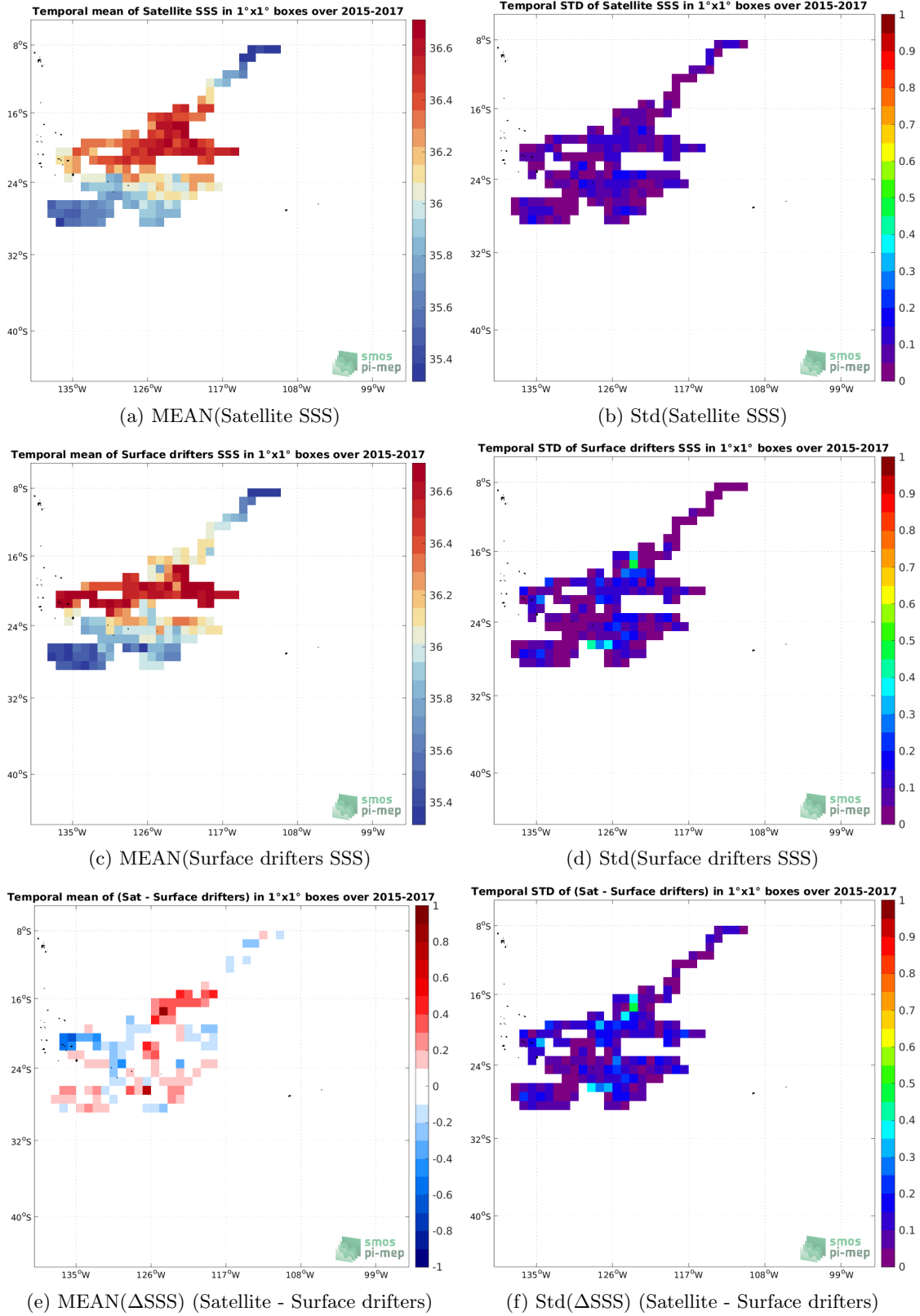
Figure 5: Temporal mean (left) and Std (right) of SSS from SMOS SSS L4 v2 - Daily (BEC) (top), Surface drifters (middle), and of \Delta SSS (Satellite - Surface drifters). Only match-up pairs are used to generate these maps.
