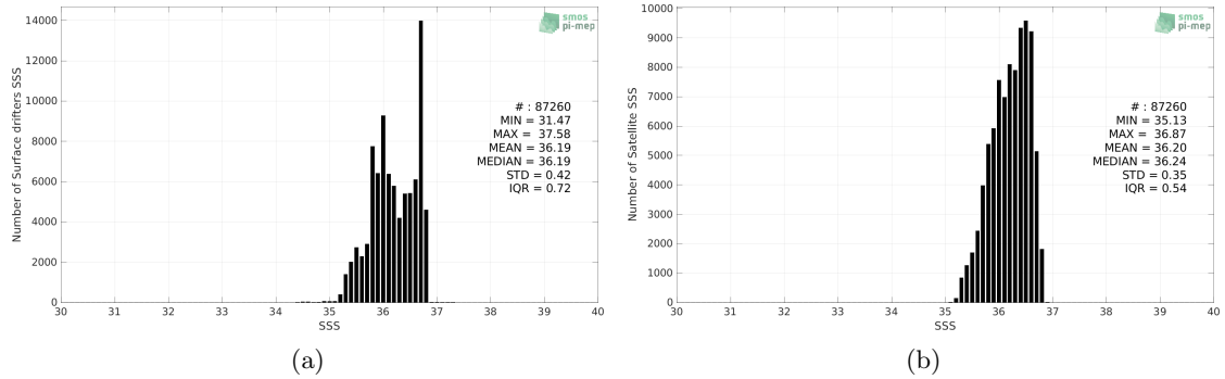
Figure 2: Histograms of SSS from Surface drifters (a) and SMOS SSS L4 v2 - Daily (BEC) (b) considering all match-up pairs per bins of 0.1 over the OTT zone Pi-MEP region and for the full satellite product period.
