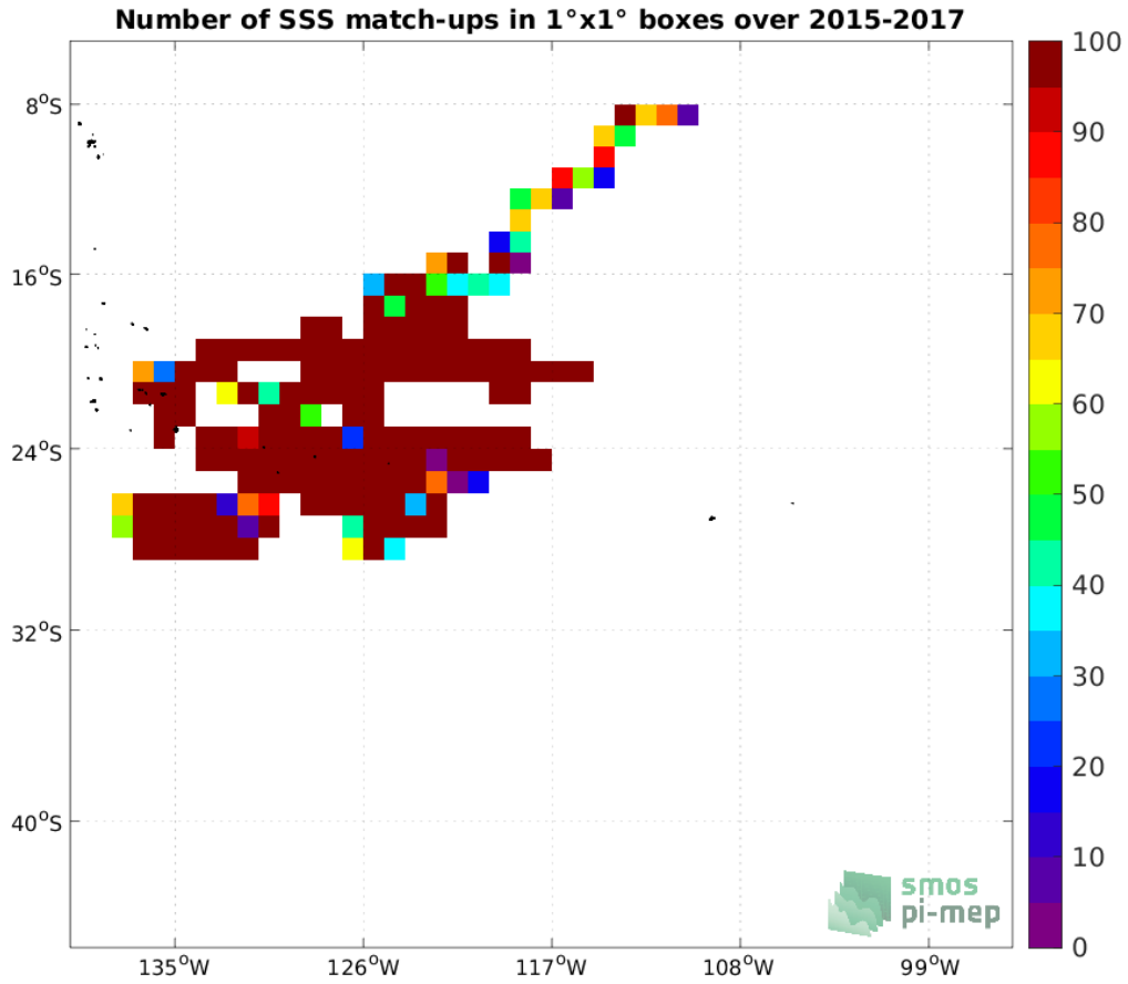
Figure 3: Number of SSS match-ups between Surface drifters SSS and the SMOS SSS L4 v2 - Daily (BEC) SSS product for the OTT zone Pi-MEP region over 1^\circ \times 1^\circ boxes and for the full satellite product period.
