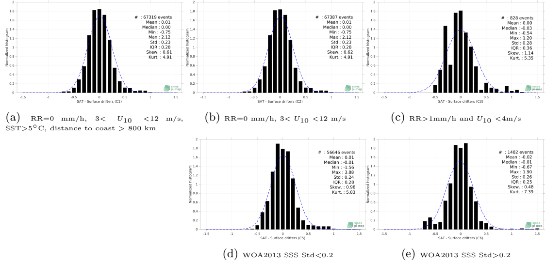
Figure 12: Normalized histogram of \Delta SSS (SMOS SSS L4 v2 - Daily (BEC) - Surface drifters) for 5 different subdatasets corresponding to: RR=0 mm/h, 3 < U_{10} < 12 m/s, SST>5°C, distance to coast > 800 km (a), RR=0 mm/h, 3 < U_{10} < 12 m/s (b), RR>1mm/h and U_{10} < 4 m/s (c), WOA2013 SSS Std<0.2 (d), WOA2013 SSS Std>0.2 (e).
