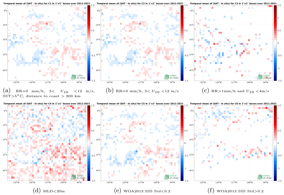
Figure 12: Temporal mean gridded over spatial boxes of size 1^\circ \times 1^\circ of \Delta SSS (SMOS SSS L4 v2 - Daily (BEC) - Argo) for 6 different subdatasets corresponding to:RR=0 mm/h, 3 < U_{10} < 12 m/s, SST >5^\circ C, distance to coast > 800 km (a), RR=0 mm/h, 3 < U_{10} < 12 m/s (b), RR >1 mm/h and U_{10} < 4 m/s (c),MLD <20 m (d),WOA2013 SSS Std <0.2 (e),WOA2013 SSS Std >0.2 (f).
