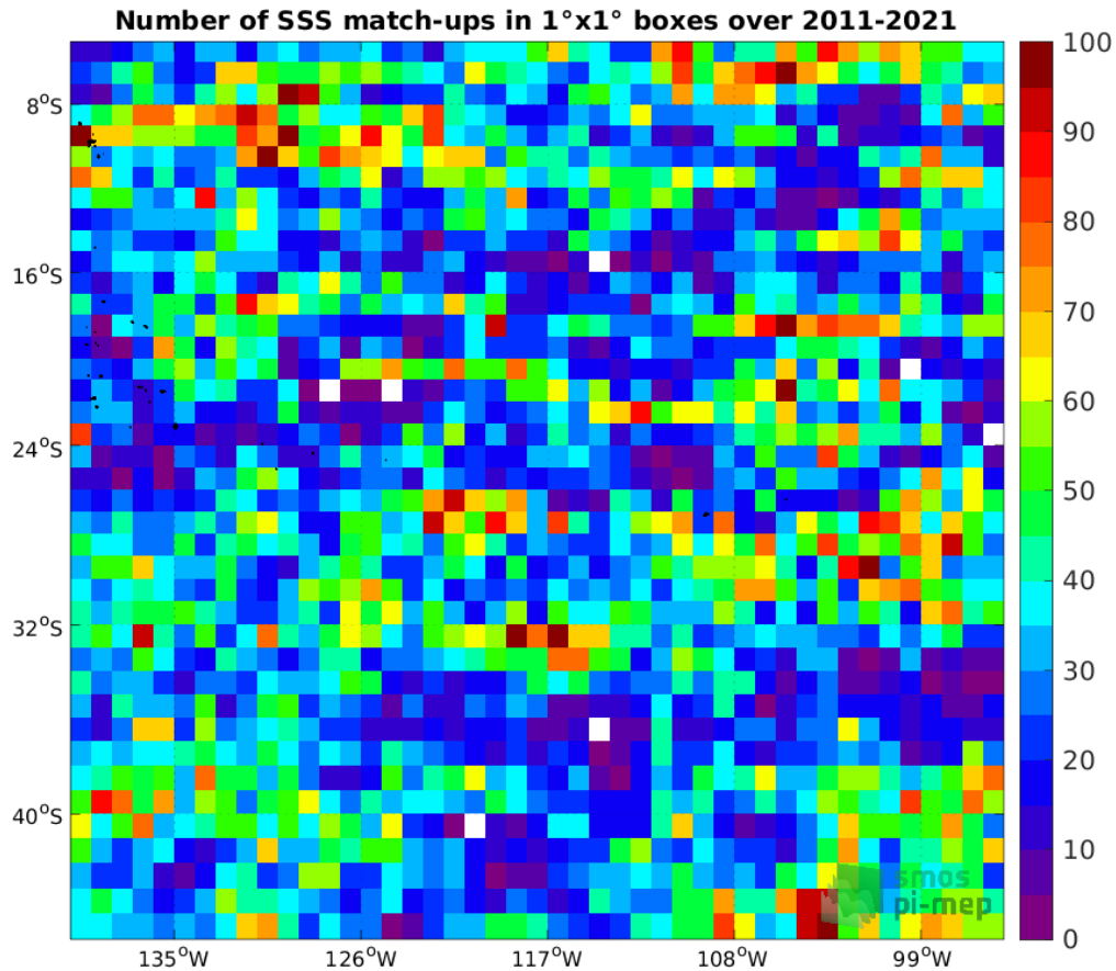
Figure 4: Number of SSS match-ups between Argo SSS and the SMOS SSS L4 v2 - Daily (BEC) SSS product for the OTT zone Pi-MEP region over 1^\circ \times 1^\circ boxes and for the full satellite product period.
