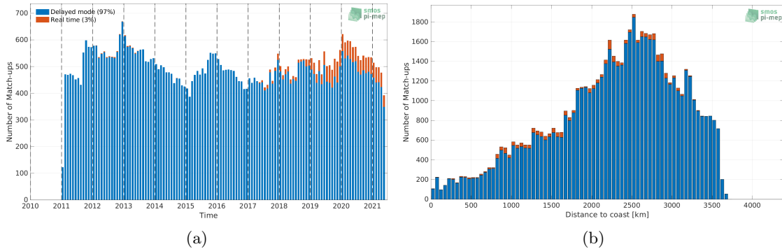
Figure 1: Number of match-ups between Argo and SMOS SSS L4 v2 - Daily (BEC) SSS as a function of time (a) and as function of the distance to coast (b) over the OTT zone Pi-MEP region and for the full satellite product period.
