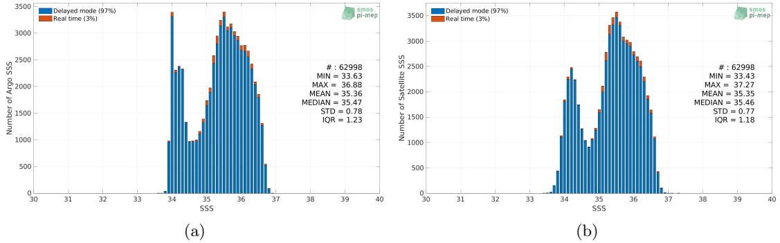
Figure 2: Histograms of SSS from Argo (a) and SMOS SSS L4 v2 - Daily (BEC) (b) considering all match-up pairs per bins of 0.1 over the OTT zone Pi-MEP region and for the full satellite product period.
