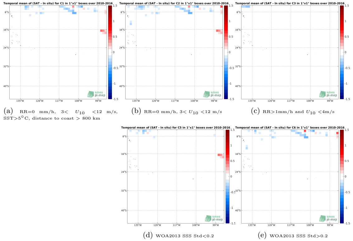
Figure 12: Temporal mean gridded over spatial boxes of size 1^\circ \times 1^\circ of \Delta SSS (SMOS SSS L3 v3 Monthly (ICDC) - TSG (SAMOS)) for 5 different subdatasets corresponding to:RR=0 mm/h, 3 < U_{10} < 12 m/s, SST>5°C, distance to coast > 800 km (a), RR=0 mm/h, 3 < U_{10} < 12 m/s (b), RR>1mm/h and U_{10} < 4 m/s (c), WOA2013 SSS Std<0.2 (d), WOA2013 SSS Std>0.2 (e).
