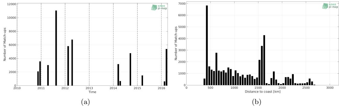
Figure 1: Number of match-ups between TSG-SAMOS and SMOS-L3-ICDC-V3-MONTHLY-0.5DEG SSS as a function of time (a) and as function of the distance to coast (b) over the OTT zone Pi-MEP region and for the full satellite product period.
