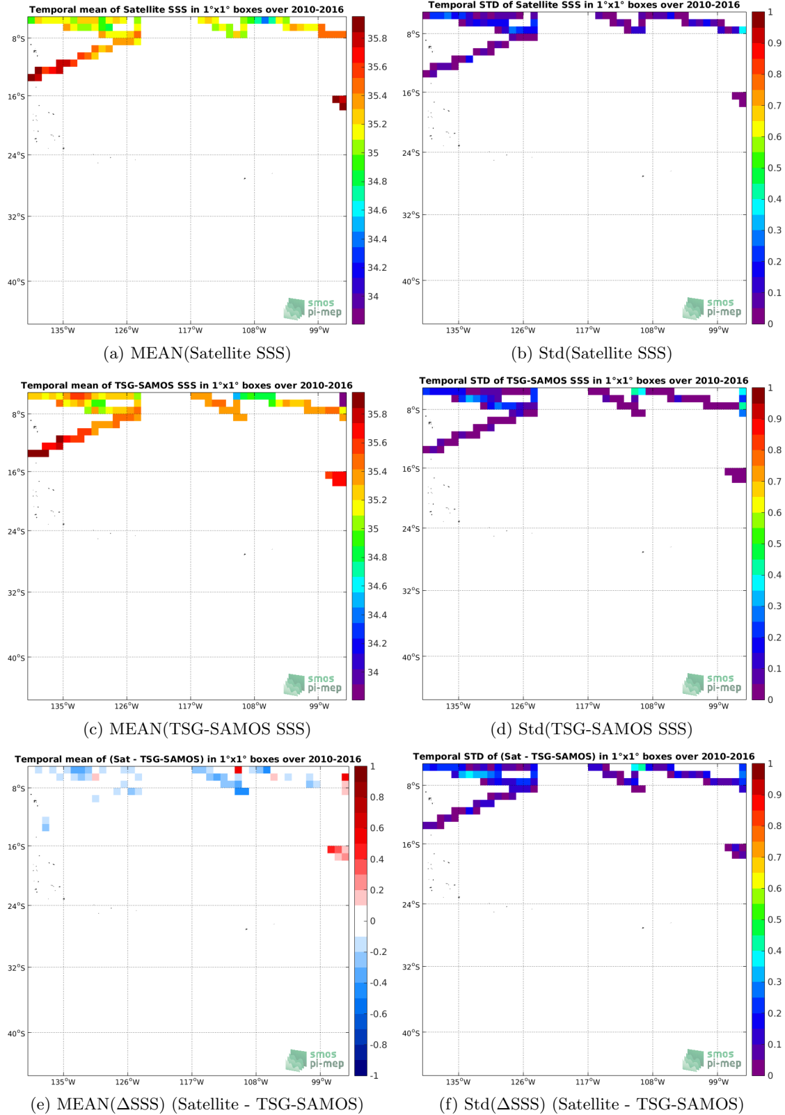
Figure 6: Temporal mean (left) and Std (right) of SSS from SMOS-L3-ICDC-V3-MONTHLY-0.5DEG (top), TSG-SAMOS (middle), and of \Delta SSS (Satellite - TSG-SAMOS). Only match-up pairs are used to generate these maps.
