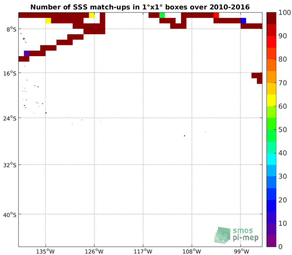
Figure 4: Number of SSS match-ups between TSG-SAMOS SSS and the SMOS-L3-ICDC-V3-MONTHLY-0.5DEG SSS product for the OTT zone Pi-MEP region over 1°x1° boxes and for the full satellite product period.
