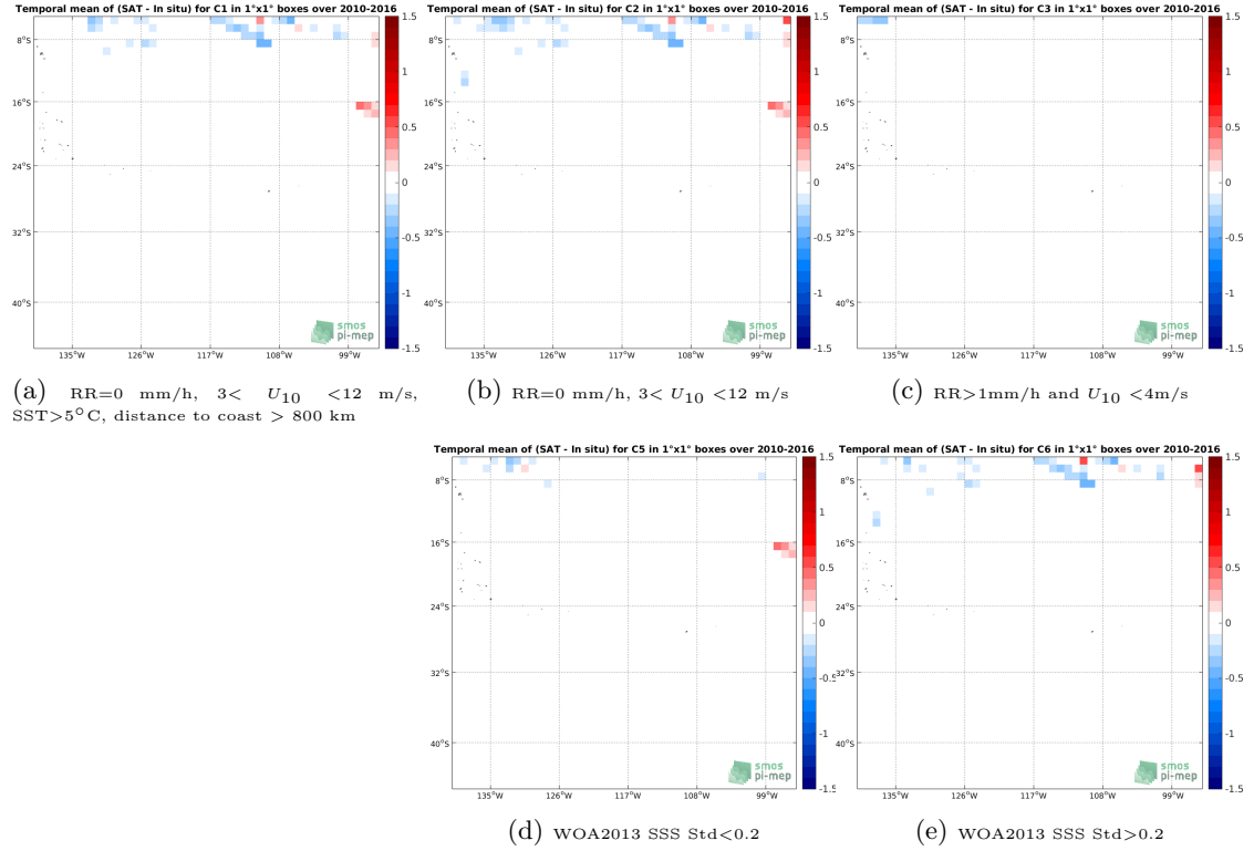
Figure 12: Temporal mean gridded over spatial boxes of size 1^\circ \times 1^\circ of \Delta SSS (SMOS-L3-ICDC-V3-MONTHLY-0.5DEG - TSG-SAMOS) for 5 different subdatasets corresponding to:RR=0 mm/h, 3 < U_{10} < 12 m/s, SST >5^\circ C, distance to coast > 800 km (a), RR=0 mm/h, 3 < U_{10} < 12 m/s (b), RR >1 mm/h and U_{10} < 4 m/s (c), WOA2013 SSS Std <0.2 (d), WOA2013 SSS Std >0.2 (e).
