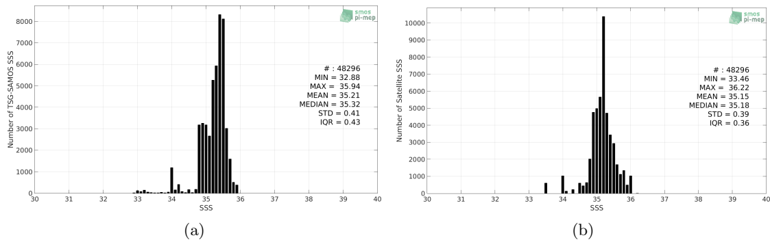
Figure 2: Histograms of SSS from TSG-SAMOS (a) and SMOS-L3-ICDC-V3-MONTHLY-0.5DEG (b) considering all match-up pairs per bins of 0.1 over the OTT zone Pi-MEP region and for the full satellite product period.
