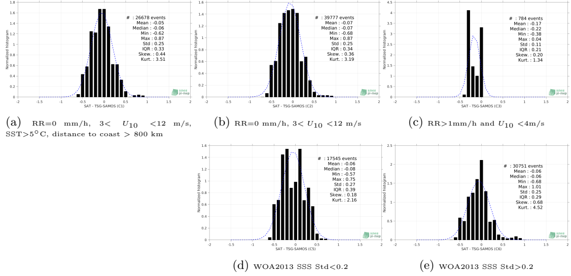
Figure 13: Normalized histogram of \Delta SSS (SMOS-L3-ICDC-V3-MONTHLY-0.5DEG - TSG-SAMOS) for 5 different subdatasets corresponding to: RR=0 mm/h, 3 < U_{10} < 12 m/s, SST>5°C, distance to coast > 800 km (a), RR=0 mm/h, 3 < U_{10} < 12 m/s (b), RR>1mm/h and U_{10} < 4 m/s (c), WOA2013 SSS Std<0.2 (d), WOA2013 SSS Std>0.2 (e).
