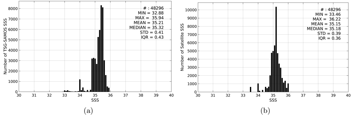
Figure 2: Histograms of SSS from TSG-SAMOS (a) and SMOS-L3-ICDC-V3-MONTHLY-0.5DEG (b) considering all match-up pairs per bins of 0.1 over the OTT zone Pi-MEP region and for the full satellite product period.
