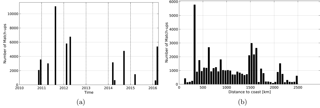
Figure 1: Number of match-ups between TSG-SAMOS and SMOS-L3-ICDC-V3-MONTHLY-0.5DEG SSS as a function of time (a) and as function of the distance to coast (b) over the OTT zone Pi-MEP region and for the full satellite product period.
