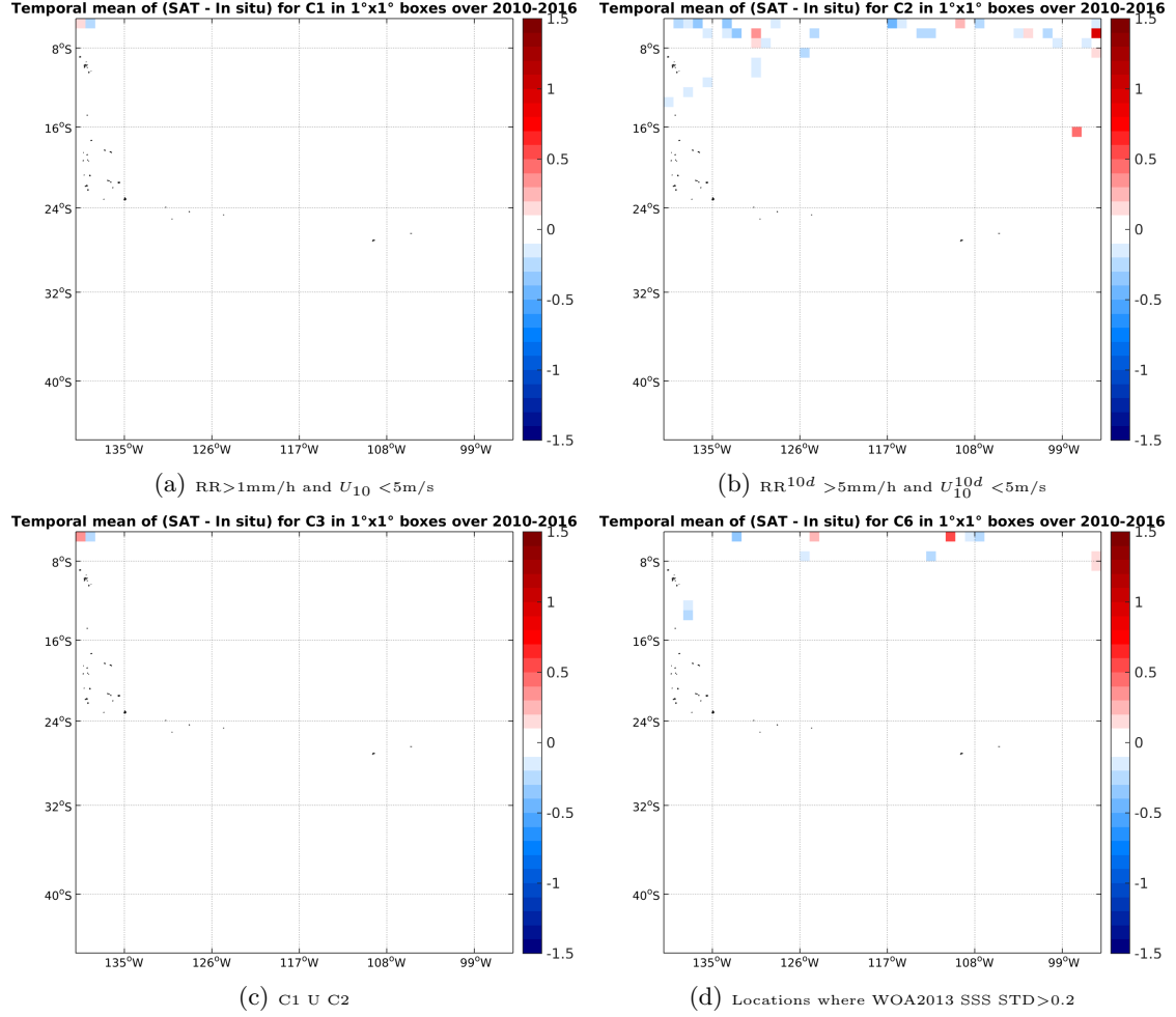
Figure 12: Temporal mean gridded over spatial boxes of size 1^\circ \times 1^\circ of \Delta SSS (SMOS-L3-ICDC-V3-MONTHLY-0.5DEG - TSG-SAMOS) for 4 different subdatasets corresponding to: RR > 1 mm/h and U_{10} < 5 m/s (a), RR^{10d} > 5 mm/h and U_{10}^{10d} < 5 m/s (b), C1 U C2 (c), Locations where WOA2013 SSS STD > 0.2 (d).
