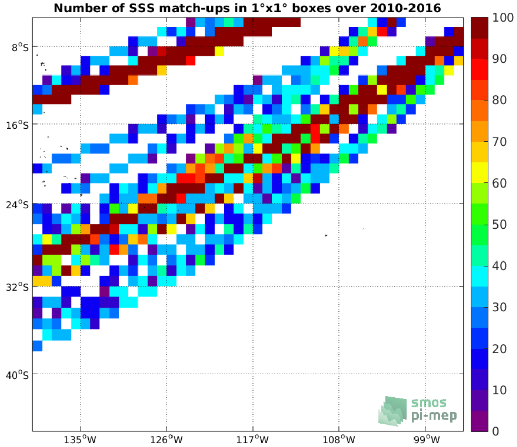
Figure 4: Number of SSS match-ups between TSG (LEGOS-DM) SSS and the SMOS SSS L3 v3 Monthly (ICDC) SSS product for the OTT zone Pi-MEP region over 1°×1° boxes and for the full satellite product period.
