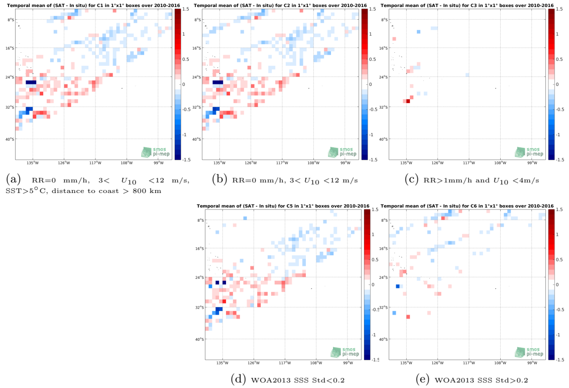
Figure 12: Temporal mean gridded over spatial boxes of size 1^\circ \times 1^\circ of \Delta SSS (SMOS SSS L3 v3 Monthly (ICDC) - TSG (LEGOS-DM)) for 5 different subdatasets corresponding to:RR=0 mm/h, 3 < U_{10} < 12 m/s, SST >5^\circ C, distance to coast > 800 km (a), RR=0 mm/h, 3 < U_{10} < 12 m/s (b), RR >1 mm/h and U_{10} < 4 m/s (c), WOA2013 SSS Std <0.2 (d), WOA2013 SSS Std >0.2 (e).
