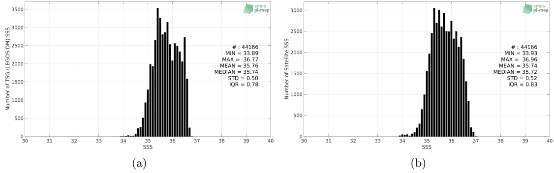
Figure 2: Histograms of SSS from TSG (LEGOS-DM) (a) and SMOS SSS L3 v3 Monthly (ICDC) (b) considering all match-up pairs per bins of 0.1 over the OTT zone Pi-MEP region and for the full satellite product period.
