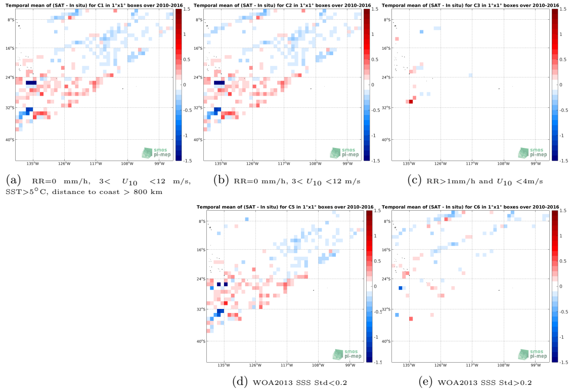
Figure 12: Temporal mean gridded over spatial boxes of size 1^\circ \times 1^\circ of \Delta SSS (SMOS SSS L3 v3 Monthly (ICDC) - TSG (LEGOS-DM)) for 5 different subdatasets corresponding to: RR=0 mm/h, 3 < U_{10} < 12 m/s, SST >5^\circ C, distance to coast > 800 km (a), RR=0 mm/h, 3 < U_{10} < 12 m/s (b), RR >1 mm/h and U_{10} < 4 m/s (c), WOA2013 SSS Std <0.2 (d), WOA2013 SSS Std >0.2 (e).
