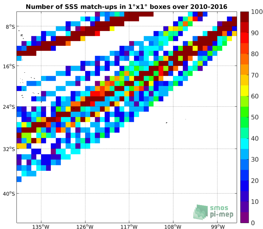
Figure 4: Number of SSS match-ups between TSG (LEGOS-DM) SSS and the SMOS SSS L3 v3 Monthly (ICDC) SSS product for the OTT zone Pi-MEP region over 1°x1° boxes and for the full satellite product period.
