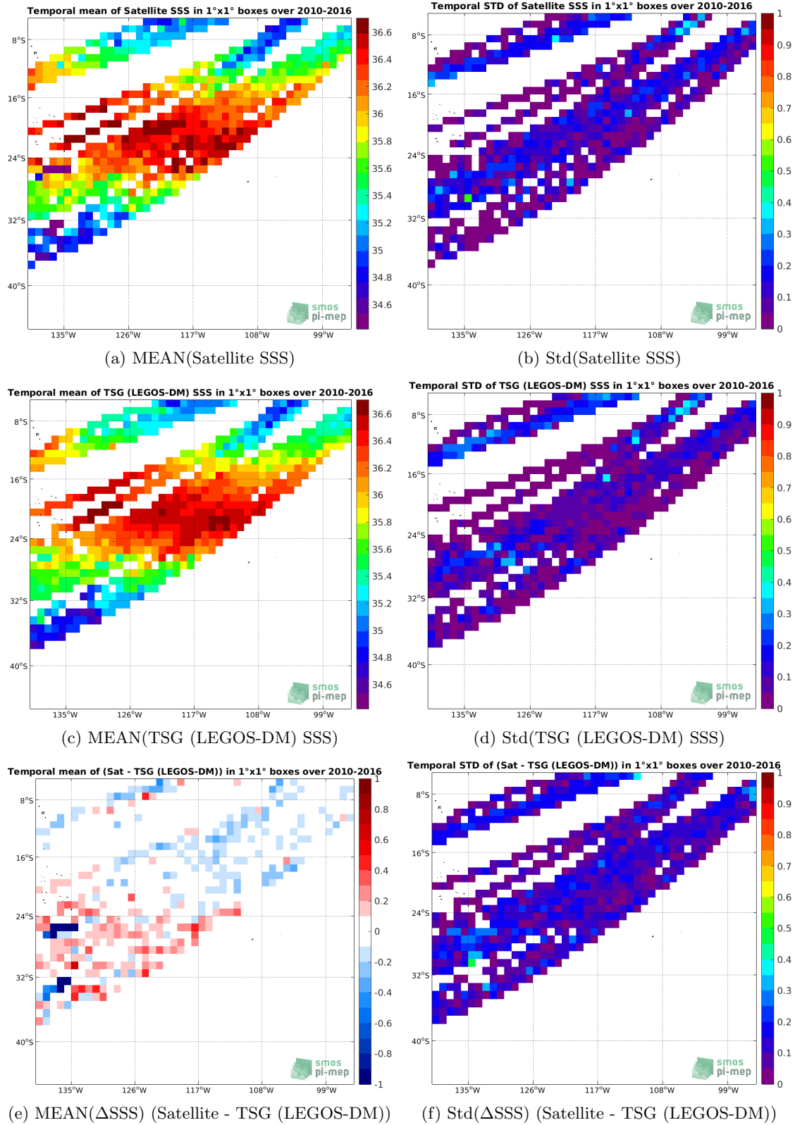
Figure 6: Temporal mean (left) and Std (right) of SSS from SMOS SSS L3 v3 Monthly (ICDC) (top), TSG (LEGOS-DM) (middle), and of \Delta SSS (Satellite - TSG (LEGOS-DM)). Only match-up pairs are used to generate these maps.
