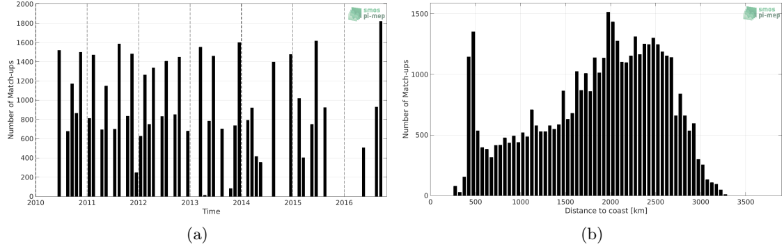
Figure 1: Number of match-ups between TSG (LEGOS-DM) and SMOS SSS L3 v3 Monthly (ICDC) SSS as a function of time (a) and as function of the distance to coast (b) over the OTT zone Pi-MEP region and for the full satellite product period.
