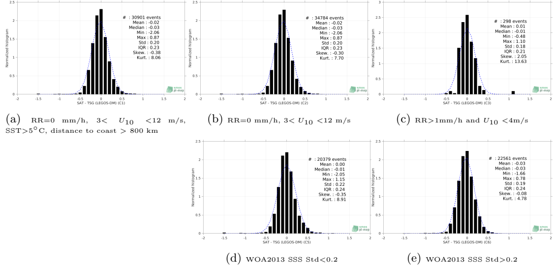
Figure 13: Normalized histogram of \Delta\text{SSS} (SMOS SSS L3 v3 Monthly (ICDC) - TSG (LEGOS-DM)) for 5 different subdatasets corresponding to: RR=0 mm/h, 3 < U_{10} < 12 m/s, SST > 5^\circ\text{C} , distance to coast > 800 km (a), RR=0 mm/h, 3 < U_{10} < 12 m/s (b), RR > 1 mm/h and U_{10} < 4 m/s (c), WOA2013 SSS Std < 0.2 (d), WOA2013 SSS Std > 0.2 (e).
