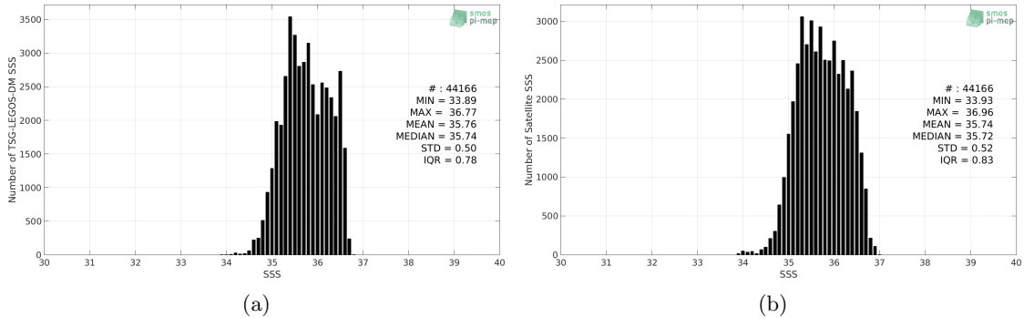
Figure 2: Histograms of SSS from TSG-LEGOS-DM (a) and SMOS-L3-ICDC-V3-MONTHLY-0.5DEG (b) considering all match-up pairs per bins of 0.1 over the OTT zone Pi-MEP region and for the full satellite product period.
