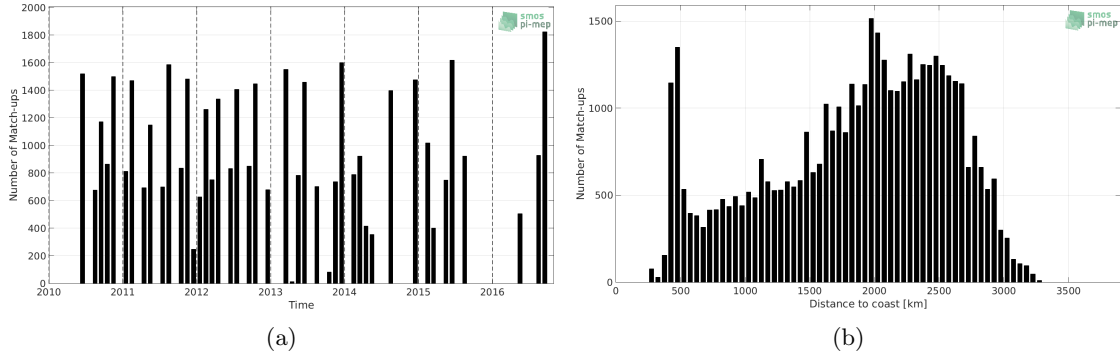
Figure 1: Number of match-ups between TSG-LEGOS-DM and SMOS-L3-ICDC-V3-MONTHLY-0.5DEG SSS as a function of time (a) and as function of the distance to coast (b) over the OTT zone Pi-MEP region and for the full satellite product period.
