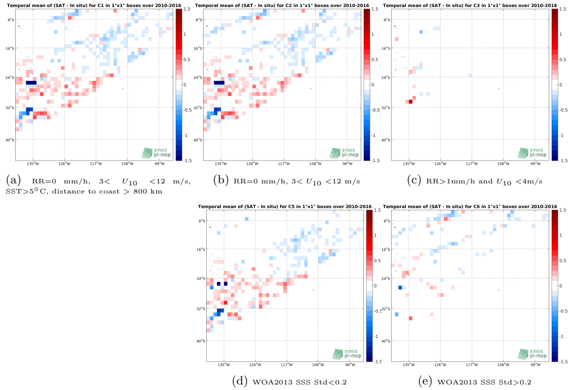
Figure 12: Temporal mean gridded over spatial boxes of size 1^\circ \times 1^\circ of \Delta SSS (SMOS-L3-ICDC-V3-MONTHLY-0.5DEG - TSG-LEGOS-DM) for 5 different subdatasets corresponding to:RR=0 mm/h, 3 < U_{10} < 12 m/s, SST >5^\circ C, distance to coast > 800 km (a), RR=0 mm/h, 3 < U_{10} < 12 m/s (b), RR >1 mm/h and U_{10} < 4 m/s (c), WOA2013 SSS Std <0.2 (d), WOA2013 SSS Std >0.2 (e).
