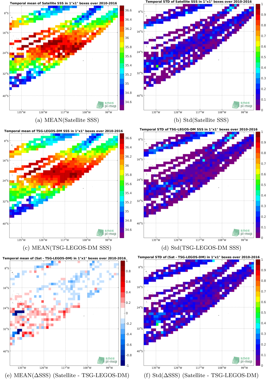
Figure 6: Temporal mean (left) and Std (right) of SSS from SMOS-L3-ICDC-V3-MONTHLY-0.5DEG (top), TSG-LEGOS-DM (middle), and of \Delta SSS (Satellite - TSG-LEGOS-DM). Only match-up pairs are used to generate these maps.
