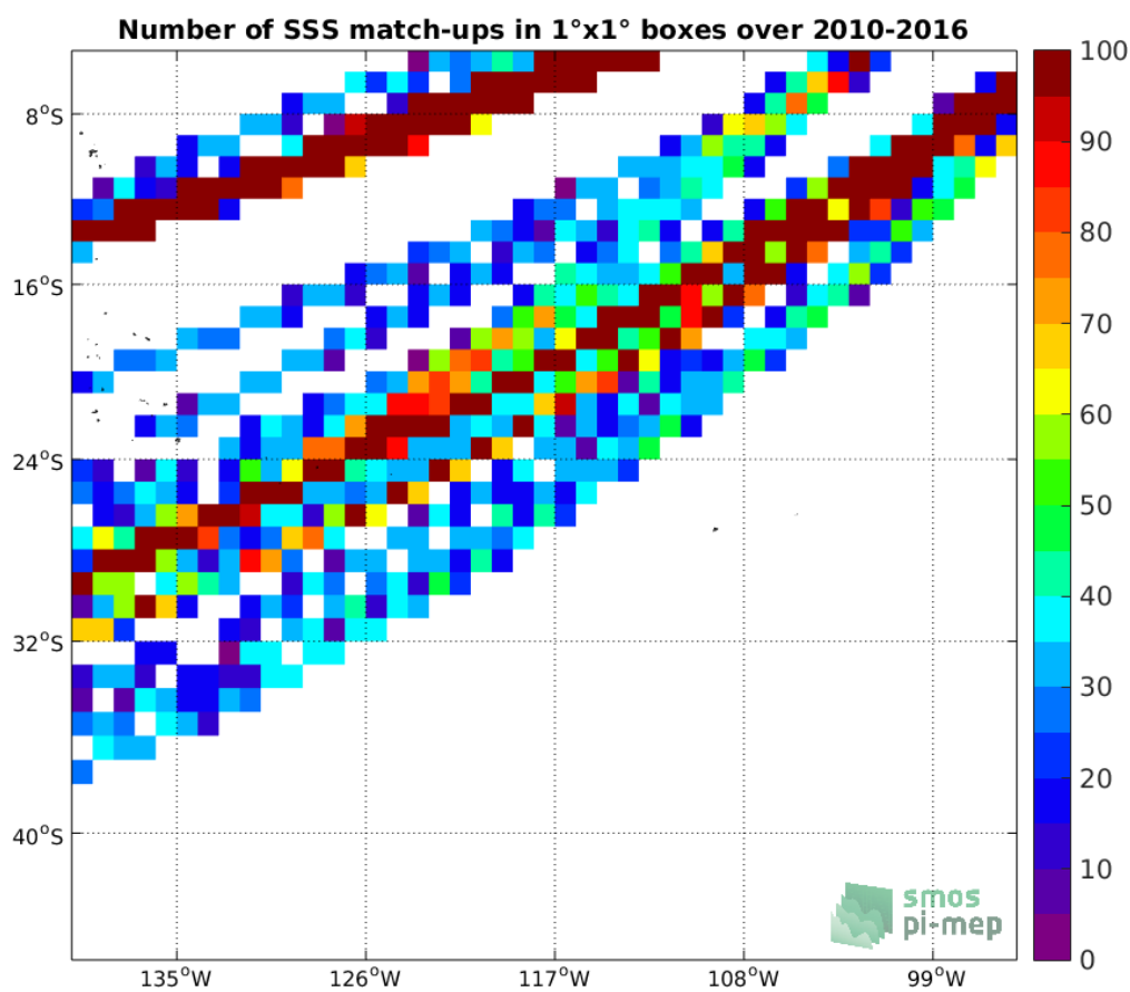
Figure 4: Number of SSS match-ups between TSG-LEGOS-DM SSS and the SMOS-L3-ICDC-V3-MONTHLY-0.5DEG SSS product for the OTT zone Pi-MEP region over 1°x1° boxes and for the full satellite product period.
