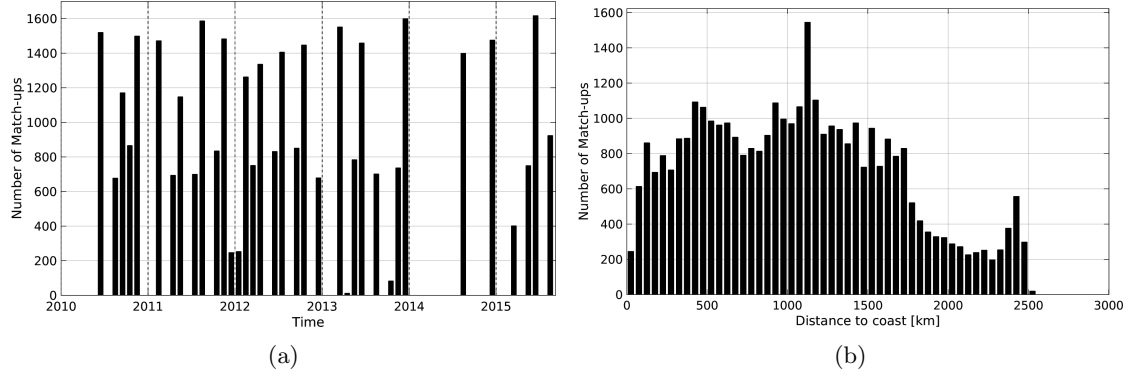
Figure 1: Number of match-ups between TSG-LEGOS-DM and SMOS-L3-ICDC-V3-MONTHLY-0.5DEG SSS as a function of time (a) and as function of the distance to coast (b) over the OTT zone Pi-MEP region and for the full satellite product period.
