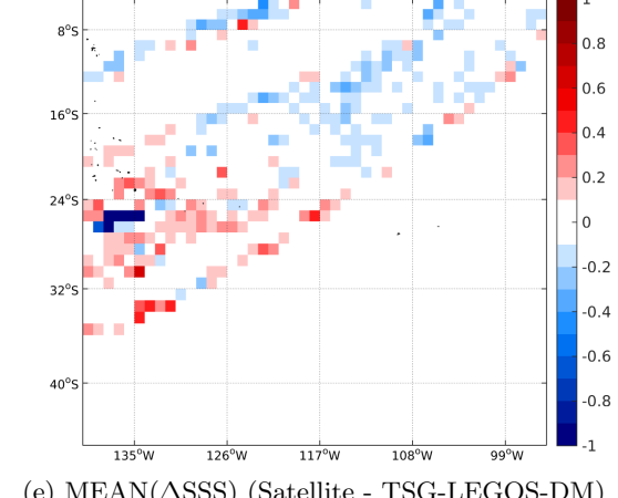
Figure 6: Temporal mean (left) and STD (right) of SSS from SMOS-L3-ICDC-V3-MONTHLY-0.5DEG (top), TSG-LEGOS-DM (middle), and of \Delta SSS (Satellite - TSG-LEGOS-DM). Only match-up pairs are used to generate these maps.
