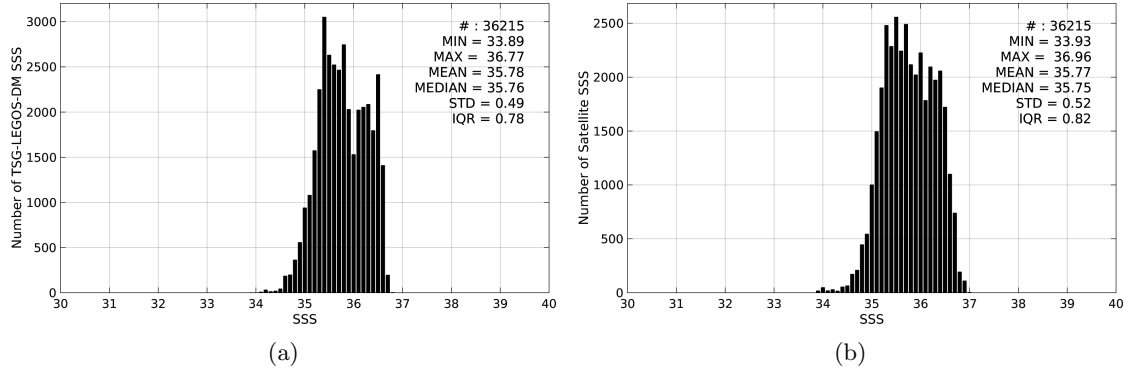
Figure 2: Histograms of SSS from TSG-LEGOS-DM (a) and SMOS-L3-ICDC-V3-MONTHLY-0.5DEG (b) considering all match-up pairs per bins of 0.1 over the OTT zone Pi-MEP region and for the full satellite product period.
