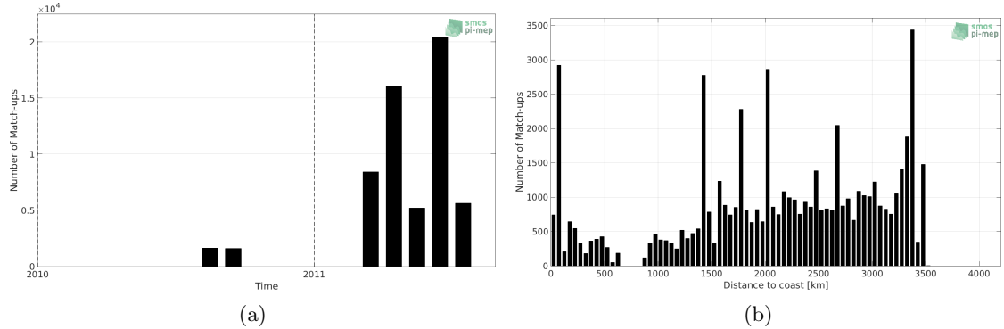
Figure 1: Number of match-ups between TSG (GOSUD-Sailing-ship) and SMOS SSS L3 v3 Monthly (ICDC) SSS as a function of time (a) and as function of the distance to coast (b) over the OTT zone Pi-MEP region and for the full satellite product period.
