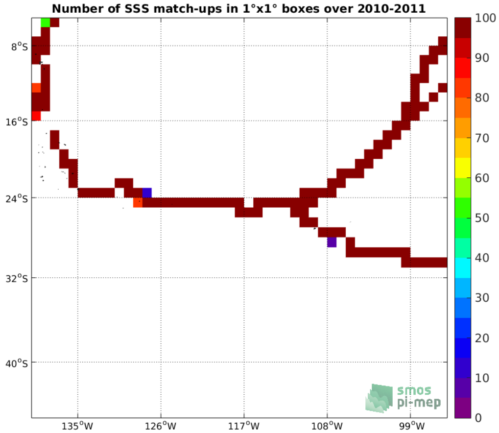
Figure 4: Number of SSS match-ups between TSG (GOSUD-Sailing-ship) SSS and the SMOS SSS L3 v3 Monthly (ICDC) SSS product for the OTT zone Pi-MEP region over 1°x1° boxes and for the full satellite product period.
