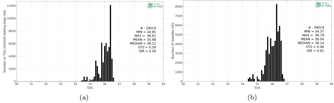
Figure 2: Histograms of SSS from TSG (GOSUD-Sailing-ship) (a) and SMOS SSS L3 v3 Monthly (ICDC) (b) considering all match-up pairs per bins of 0.1 over the OTT zone Pi-MEP region and for the full satellite product period.
