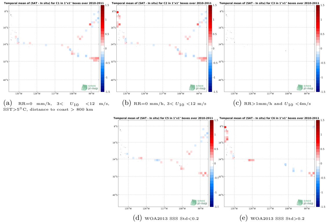
Figure 12: Temporal mean gridded over spatial boxes of size 1^\circ \times 1^\circ of \Delta SSS (SMOS SSS L3 v3 Monthly (ICDC) - TSG (GOSUD-Sailing-ship)) for 5 different subdatasets corresponding to: RR=0 mm/h, 3 < U_{10} < 12 m/s, SST > 5^\circ C , distance to coast > 800 km (a), RR=0 mm/h, 3 < U_{10} < 12 m/s (b), RR > 1 mm/h and U_{10} < 4 m/s (c), WOA2013 SSS Std < 0.2 (d), WOA2013 SSS Std > 0.2 (e).
