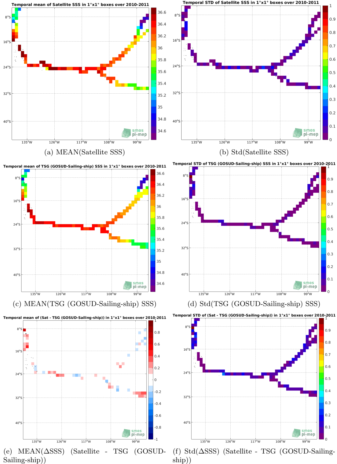
Figure 6: Temporal mean (left) and Std (right) of SSS from SMOS SSS L3 v3 Monthly (ICDC) (top), TSG (GOSUD-Sailing-ship) (middle), and of \Delta SSS (Satellite - TSG (GOSUD-Sailing-ship)). Only match-up pairs are used to generate these maps.
