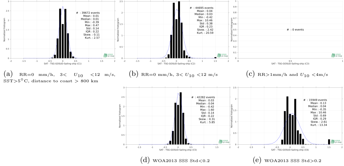
Figure 13: Normalized histogram of \Delta SSS (SMOS-L3-ICDC-V3-MONTHLY-0.5DEG - TSG-GOSUD-Sailing-ship) for 5 different subdatasets corresponding to: RR=0 mm/h, 3 < U_{10} < 12 m/s, SST > 5^\circ\text{C} , distance to coast > 800 km (a), RR=0 mm/h, 3 < U_{10} < 12 m/s (b), RR > 1\text{mm/h} and U_{10} < 4\text{m/s} (c), WOA2013 SSS Std < 0.2 (d), WOA2013 SSS Std > 0.2 (e).
