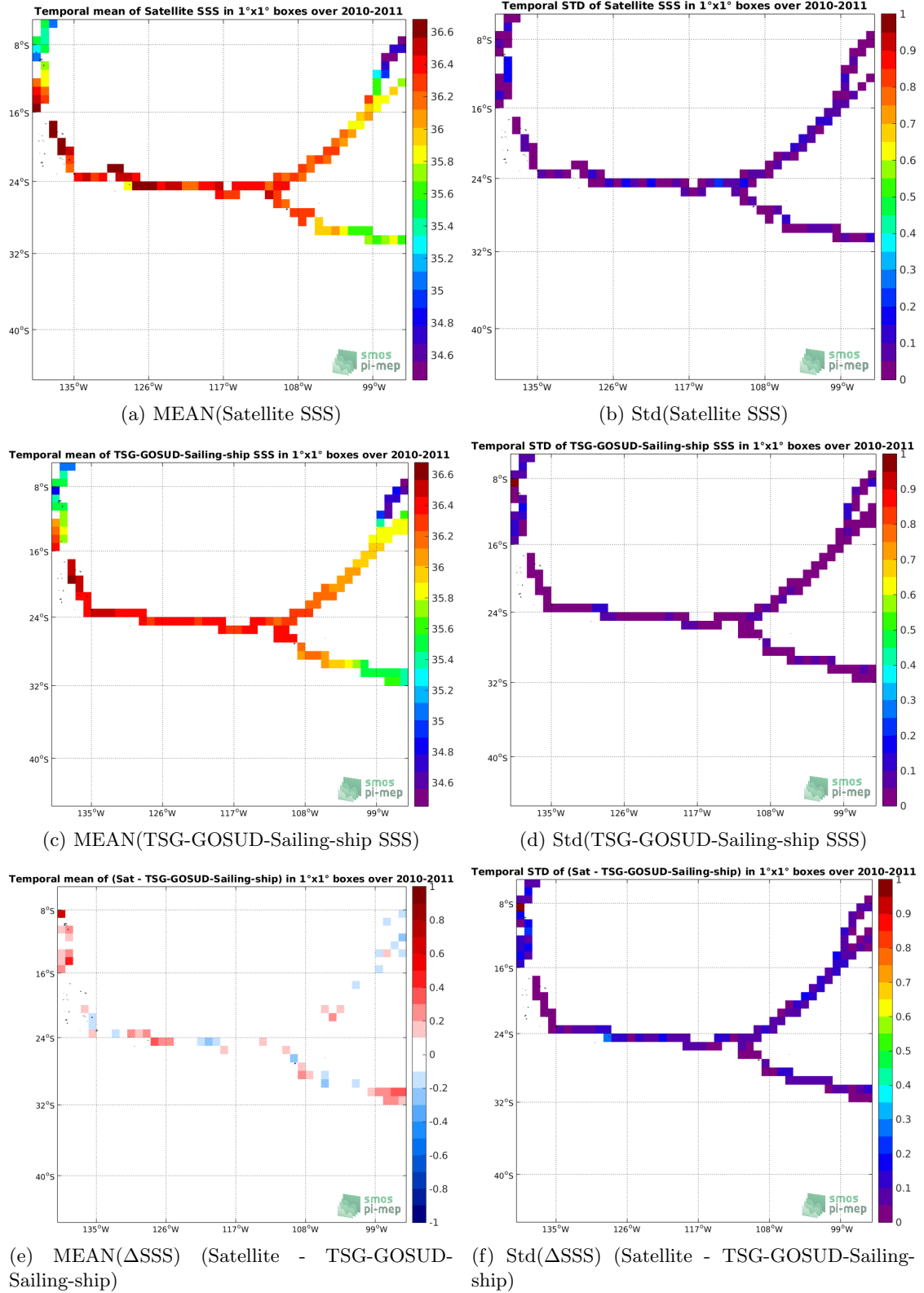
Figure 6: Temporal mean (left) and Std (right) of SSS from SMOS-L3-ICDC-V3-MONTHLY-0.5DEG (top), TSG-GOSUD-Sailing-ship (middle), and of \Delta SSS (Satellite - TSG-GOSUD-Sailing-ship). Only match-up pairs are used to generate these maps.
