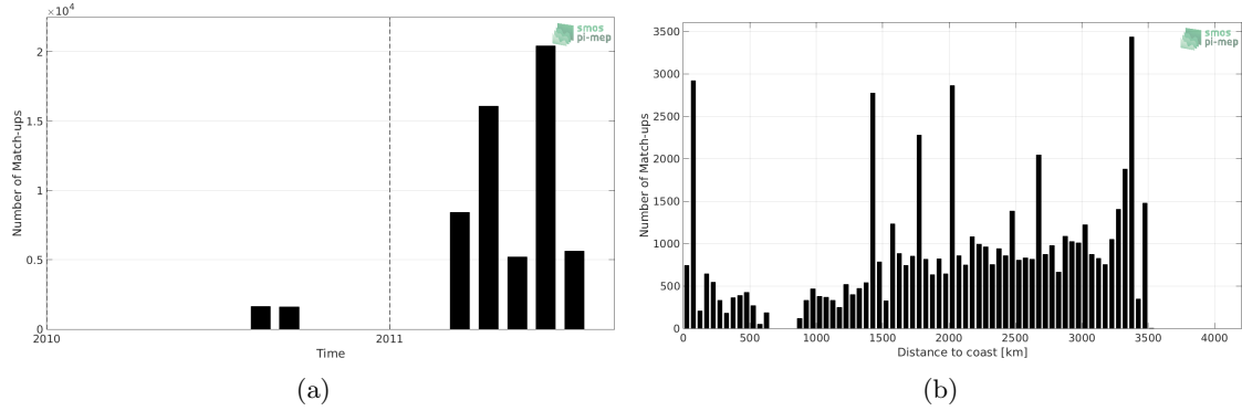
Figure 1: Number of match-ups between TSG-GOSUD-Sailing-ship and SMOS-L3-ICDC-V3-MONTHLY-0.5DEG SSS as a function of time (a) and as function of the distance to coast (b) over the OTT zone Pi-MEP region and for the full satellite product period.
