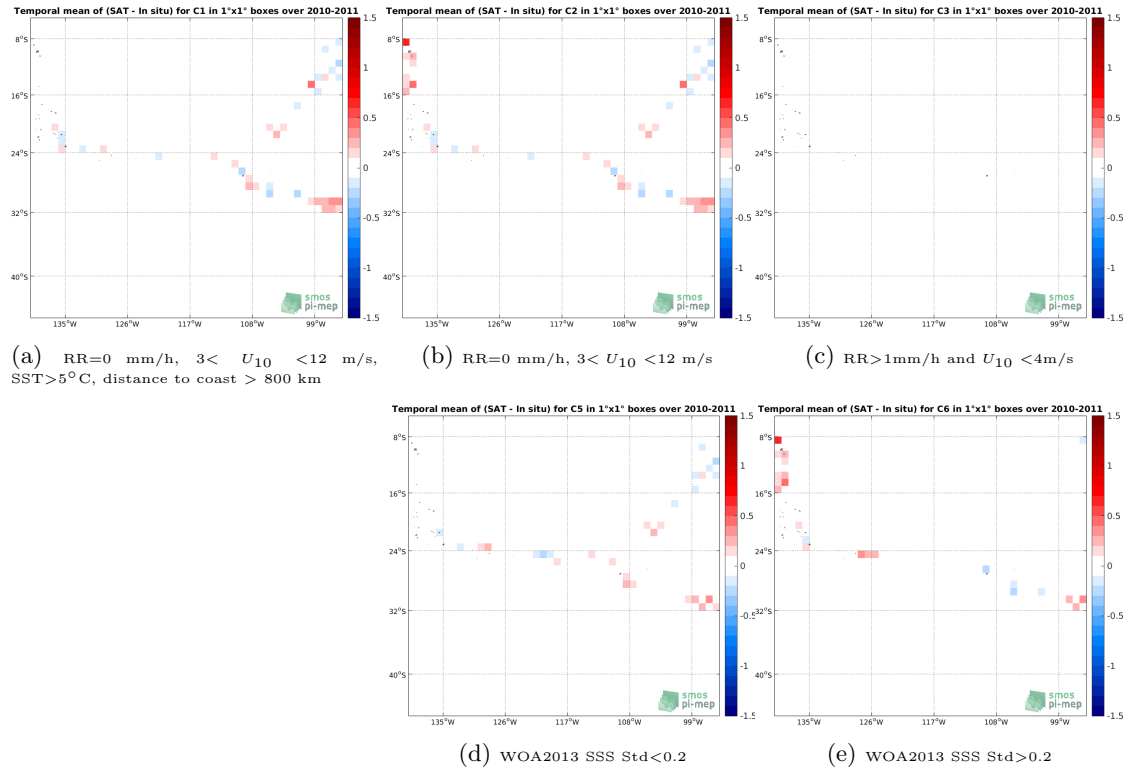
Figure 12: Temporal mean gridded over spatial boxes of size 1^\circ \times 1^\circ of \Delta SSS (SMOS-L3-ICDC-V3-MONTHLY-0.5DEG - TSG-GOSUD-Sailing-ship) for 5 different subdatasets corresponding to: RR=0 mm/h, 3 < U_{10} < 12 m/s, SST >5^\circ C, distance to coast > 800 km (a), RR=0 mm/h, 3 < U_{10} < 12 m/s (b), RR >1 mm/h and U_{10} < 4 m/s (c), WOA2013 SSS Std <0.2 (d), WOA2013 SSS Std >0.2 (e).
