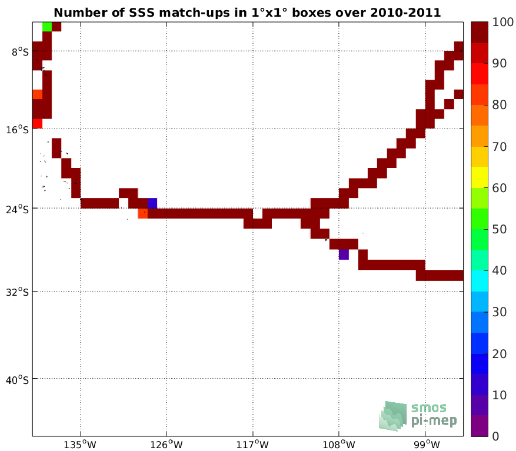
Figure 4: Number of SSS match-ups between TSG-GOSUD-Sailing-ship SSS and the SMOS-L3-ICDC-V3-MONTHLY-0.5DEG SSS product for the OTT zone Pi-MEP region over 1°x1° boxes and for the full satellite product period.
