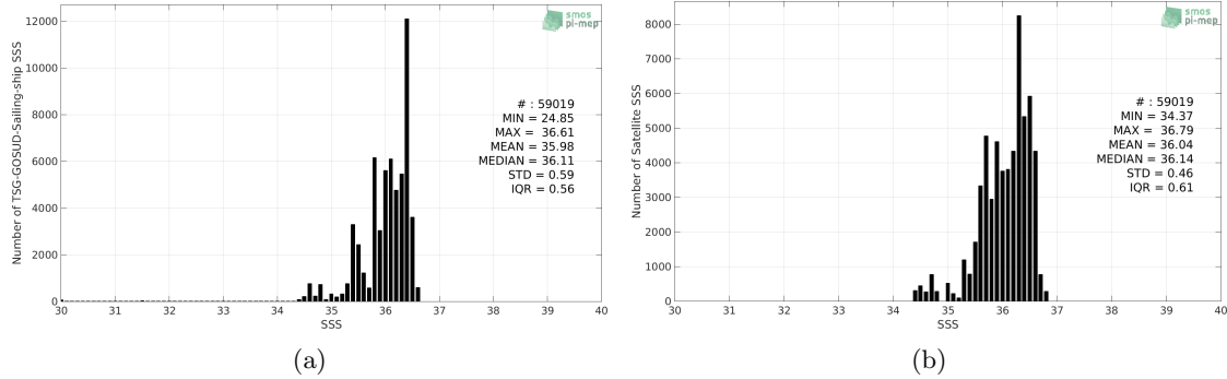
Figure 2: Histograms of SSS from TSG-GOSUD-Sailing-ship (a) and SMOS-L3-ICDC-V3-MONTHLY-0.5DEG (b) considering all match-up pairs per bins of 0.1 over the OTT zone Pi-MEP region and for the full satellite product period.
