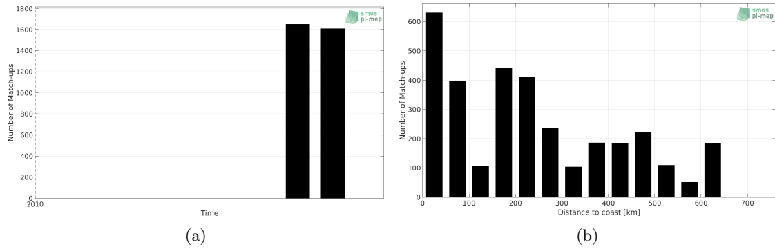
Figure 1: Number of match-ups between TSG-GOSUD-Sailing-ship and SMOS-L3-ICDC-V3-MONTHLY-0.5DEG SSS as a function of time (a) and as function of the distance to coast (b) over the OTT zone Pi-MEP region and for the full satellite product period.
